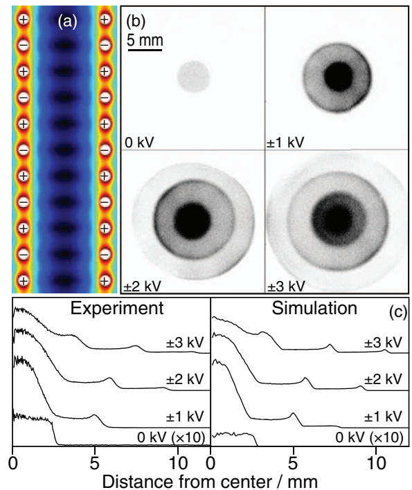
FIG. 5. (Color online) Transverse position distribution of the molecules after the decelerator with 0 \text{ kV} , \pm 1 \text{ kV} , \pm 2 \text{ kV} , and \pm 3 \text{ kV} applied to the electrodes. Panel (a): Electric field distribution in the decelerator with alternating positive and negative voltages on the electrodes. Panel (b): two-dimensional transverse distributions at the detector for the various applied potentials. Panel (c): angle-integrated radial intensity profile of the distributions shown in panel (b).
