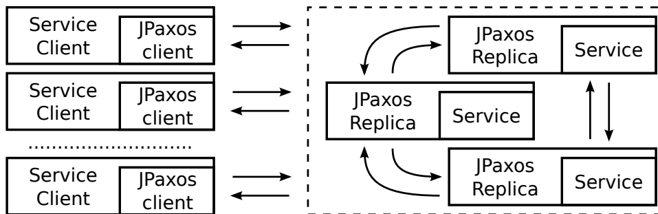
Figure 3: A service replicated in three replicas accessed by several clients. Arrows indicate communication flows.
