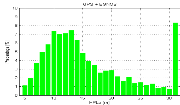
Figure 10: HPL distribution GPS + EGNOS
