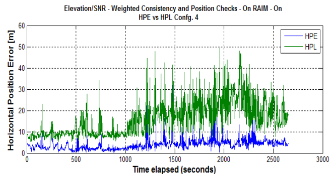
Figure 7: Position Error and Protection Level - Nottingham City Centre
