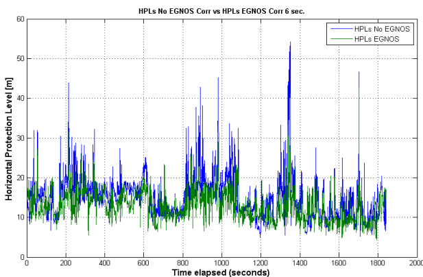
Figure 8: HPL GPS vs GPS + EGNOS
