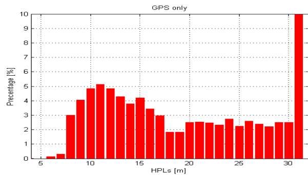
Figure 9: HPL distribution GPS
