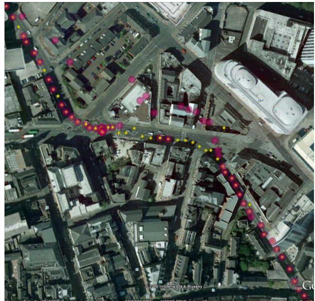
Figure 6: RAIM Impact (red = no RAIM, yellow = RAIM)
