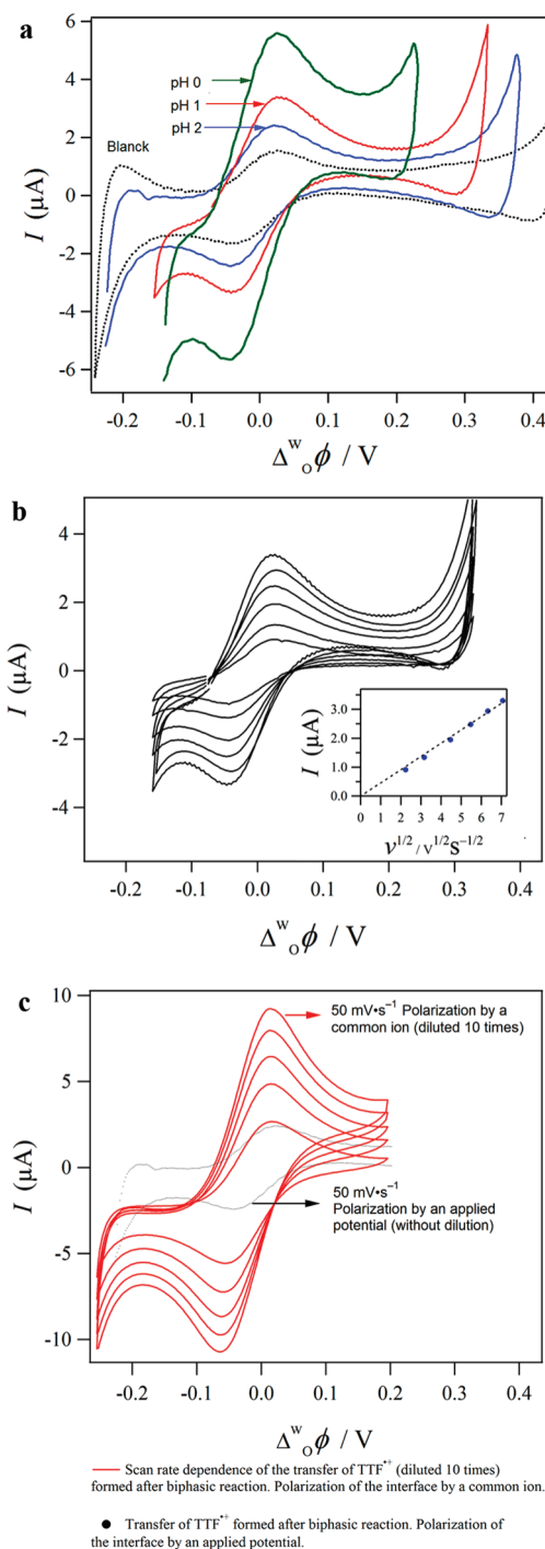
Figure 5. Ion transfer voltammograms obtained by using the system illustrated in Scheme 2 (5 mM TTF); (a) pH dependence; (b) scan rate dependence at pH = 1; (c) transfer of the \text{TTF}^{*+} formed after biphasic reaction (12 h) using the common ion \text{TB}^- (cell II, Scheme 1: 5 mM TTF, pH = 2). The organic phase was diluted 10 times prior to ion transfer analysis.
