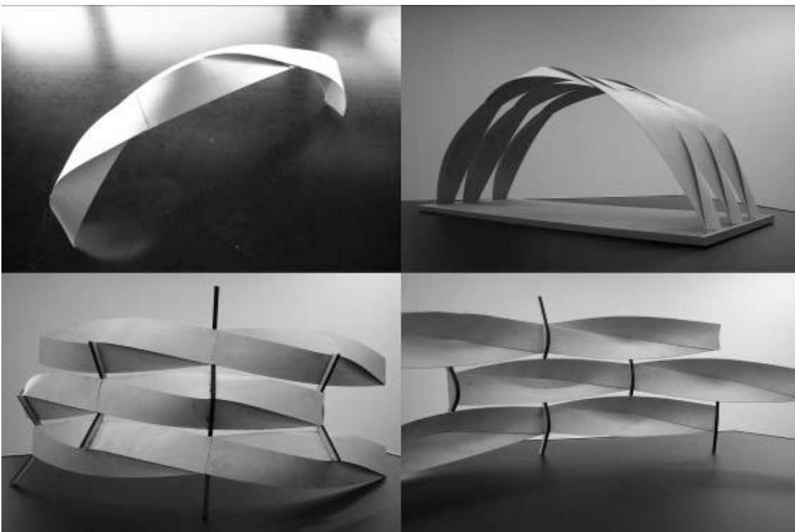
Figure 5. Textile module and their combinations on building scale
