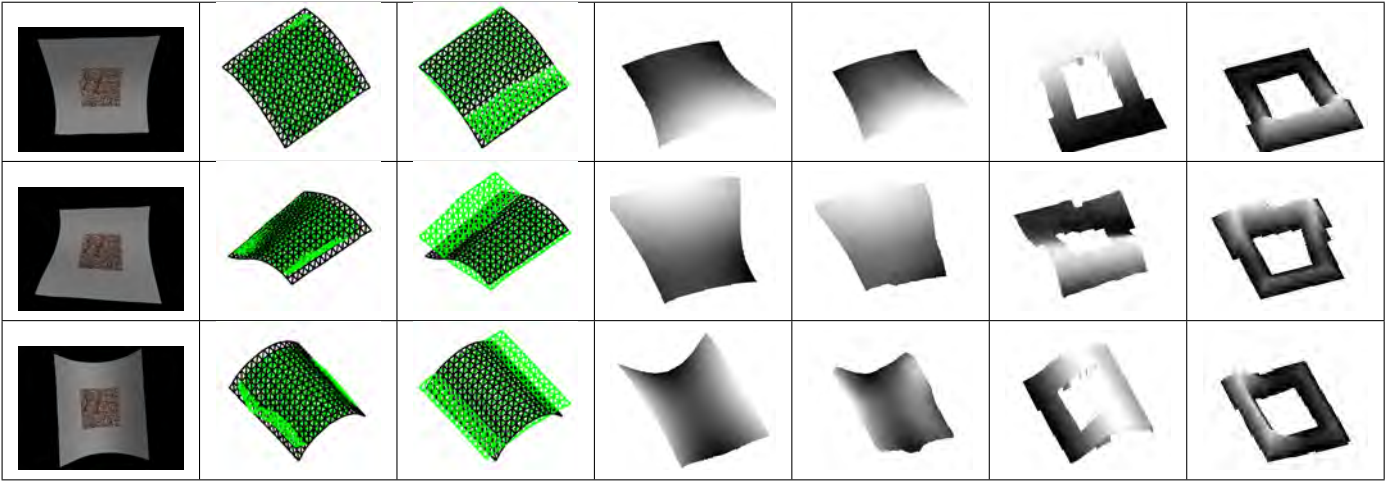
Fig. 9. Synthetic Experiments First column. Input images. Second column. Estimated triangulation (green) and ground-truth triangulation (black) seen from another view point. Third column. Reconstruction results using the method in [35] (green mesh) and ground-truth triangulation (black). Forth column. Ground truth depth maps. Fifth column. Depth maps computed from our reconstructions. Sixth and last columns. Depth maps computed by the methods of [45] and [14], respectively.
