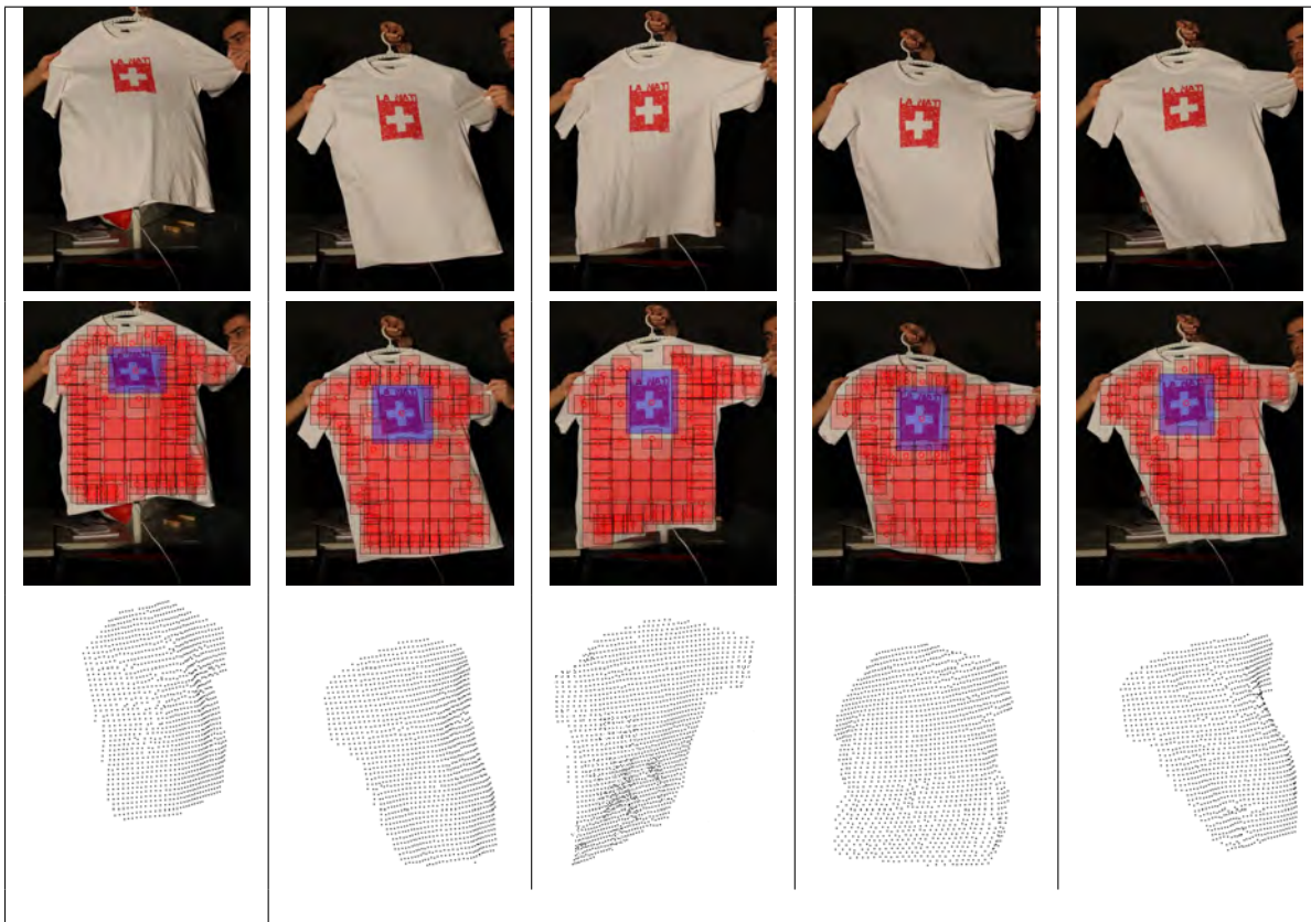
Fig. 14. T-Shirt Sequence. First row Input images. Second row Local Patches. The blue patch is the one for which enough correspondences are found and the red ones are featureless patches. Third row Reconstructed point cloud seen from another viewpoint.
