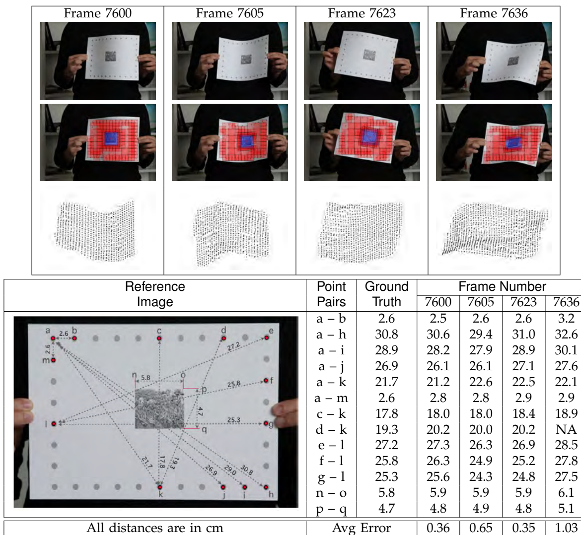
Fig. 13. Paper Sequence. First row Input images. Second row Local Patches. The blue patch is the one for which enough correspondences are found and the red ones are featureless patches. Third row Reconstructed point cloud seen from another viewpoint. Fourth row Geodesic distances between prominent landmarks as identified on the left. Point d in frame 7636 was outside our reconstruction, which explains the missing value in the table.
