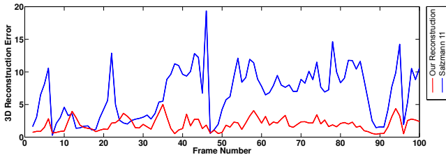
Fig. 10. Reconstruction error of both methods for all the frames in the sequence. Note that the proposed method provides much better reconstructions, except for 6 frames in the sequence.
