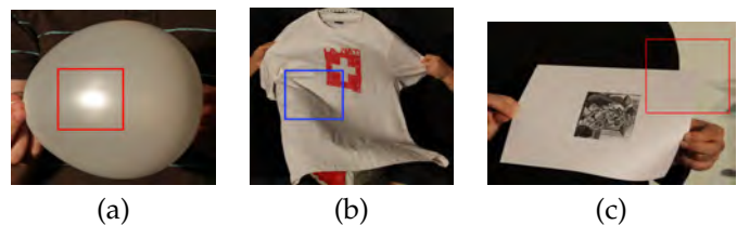
Fig. 16. Failure Modes. (a) Non-Lambertian surface. (b) Folds that create self-shadows. (c) Background albedo very similar to the surface.
