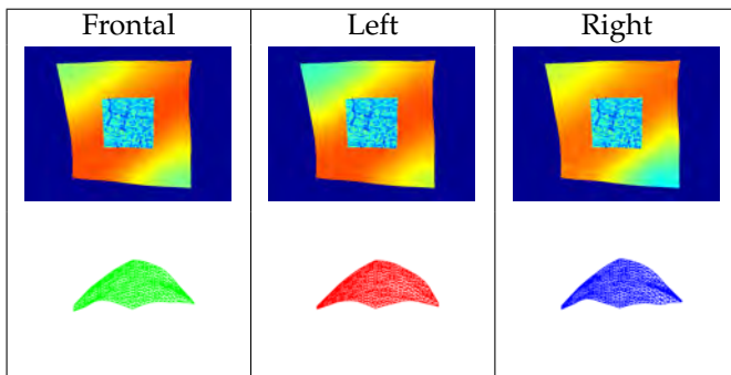
Fig. 12. Robustness to Lighting Environment The surface is lit by three different lighting schemes. Top row: Intensity variation in the surface. Bottom row: Reconstructed surfaces.
