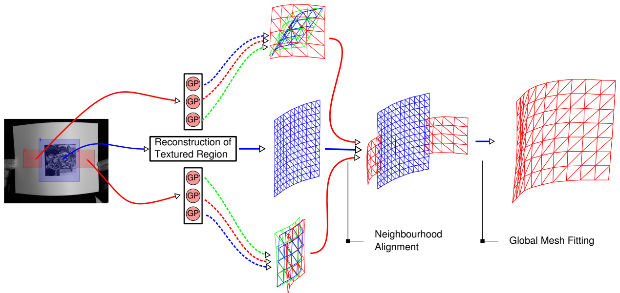
Fig. 2. Algorithmic flow. We partition the image into patches, some of which are labeled as textured and others as featureless. We compute the 3D shape of textured patches such as the blue one by establishing point correspondences with a reference image in which the shape is known. We use Gaussian Processes trained on synthetic data to predict plausible 3D shapes for featureless patches such as the red ones. Finally, neighborhood alignment of the patches is done using a Markov Random Field to choose among all possible local interpretations those that are globally consistent.
