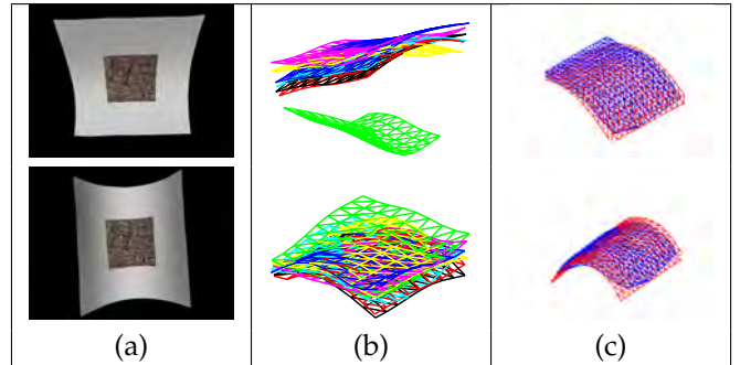
Fig. 11. Reconstruction with multiple 3D hypotheses for the textured patch. (a) Input images. (b) 3D hypotheses for the textured patches. (c) 3D reconstructions of the surfaces.
