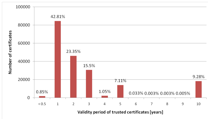
Fig. 10 Distribution of validity periods (in years) of trusted valid certificates. Almost half of the certificates are issued for one year, indicating that it might be too costly for businesses to pay for certificates valid for several years or that they do not favor long term investment. It might also be due to unwillingness of CAs to trust websites for too long, as it limits the risk of bad publicity in case a malicious websites is actually issued a certificate.
