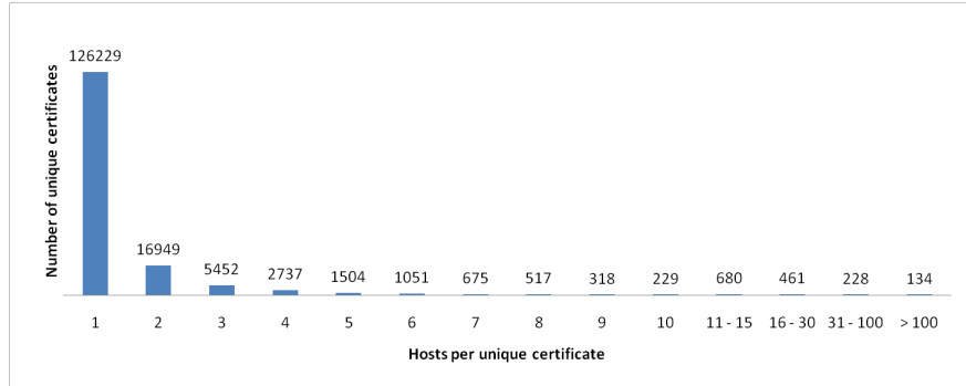
Fig. 7 Reusing certificates across multiple domains. A high number of certificates (both trusted and self-signed) that are issued for a single domain appear across a number of different domains. Deployment on those other (invalid) domains causes a domain mismatch authentication failure.
