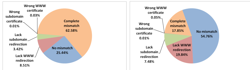
(a) Domain matching for trusted certificates with (b) Domain matching for unique, trusted certificates with valid signatures.
