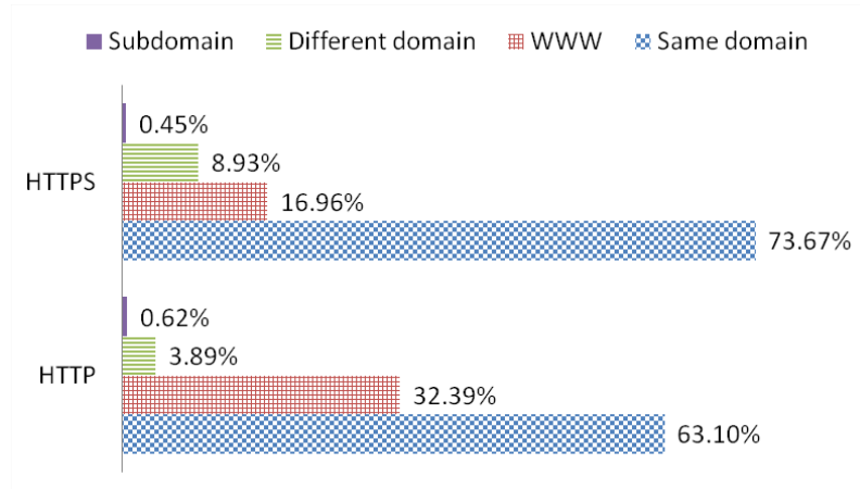
Fig. 4 Final domain after following redirections, compared to initial domain. Typically, the final page is in the initial domain or in the www subdomain with both HTTP and HTTPS.
