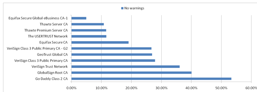
Fig. 14 Authentication success rate across CAs. Certificates issued by GlobalSign, GoDaddy and VeriSign achieve higher authentication success rate. Either they help their clients manage certificates properly or their customers are more security conscious and resourceful and take better care of their certificates.
