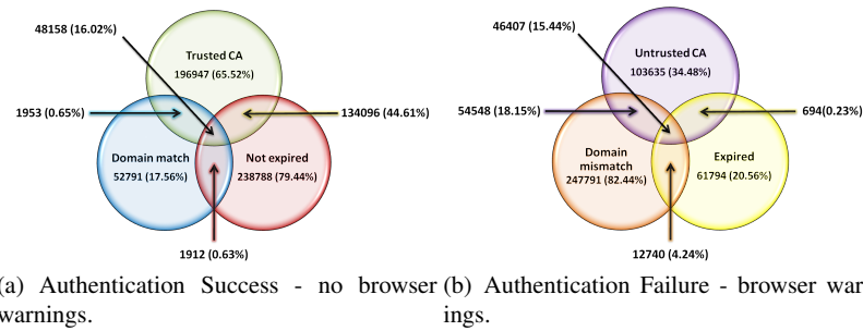
Fig. 6 Web browser authentication outcomes for websites that implement HTTPS and whose certificate signatures can be verified. Certificates of only 16.02% (48'158) of those websites allow for a correct authentication. When authentication fails, in 82.44% of the cases it is due to a domain mismatch.
