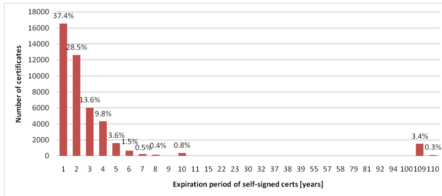
Fig. 8 Distribution of the expiration periods (in years) of self-signed certificates. In addition to being untrusted, most of the self-signed certificates are also expired (45.54%) and have a domain mismatch (97.48%). Even though self-signed certificates have almost no cost and are easy to generate, they are not maintained properly.
