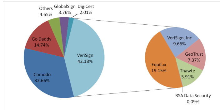
Fig. 11 CA root certificates. VeriSign has the largest share of the market, followed by Comodo. The certificates issued by GeoTrust, Thawte and Equifax are counted as VeriSign certificates as these CAs were acquired by VeriSign.
