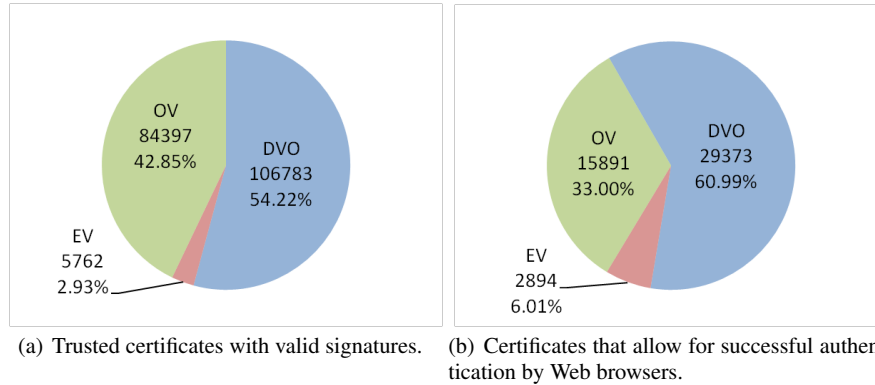
Fig. 12 Types of certificates: EV, OV and DVO. A small number of websites have certificates (EV or OV) that provide the trust in the identity of the organization owning a certificate. About 61% of the certificates trusted by Web browsers do not guarantee the legitimacy of the owner, i.e., are DVO.
