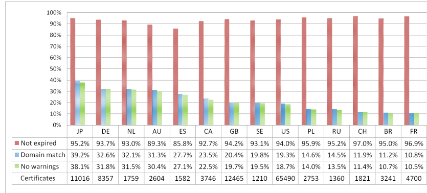
Fig. 15 Certificate validity across countries. Organizations from Japan, Germany and Netherlands have the best, whereas France, Brazil and Switzerland have the poorest practices in deploying certificates. The major reason for authentication failure is due to domain mismatch, as most of the certificates are not expired.
