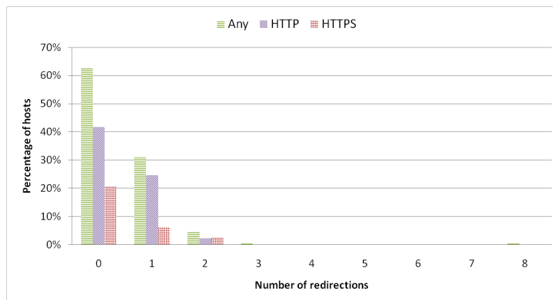
Fig. 3 Number of Redirections with HTTP and HTTPS. Most of the websites perform one or no redirection at all. Redirections occur more frequently when websites are browsed via HTTP than via HTTPS.
