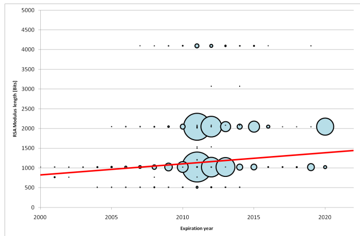
Fig. 13 Appropriateness of the key length wrt. expiration time. Data point (Expiration Year, Key Length) is represented with the center of a bubble and the size of the bubble represent a number of data points with the same value. Data points above the recommended key length curve (linear) are well chosen, the ones below are not considered to be secure at the time they are used. About half of the trusted certificates have inappropriate key length with respect to their time validity.
