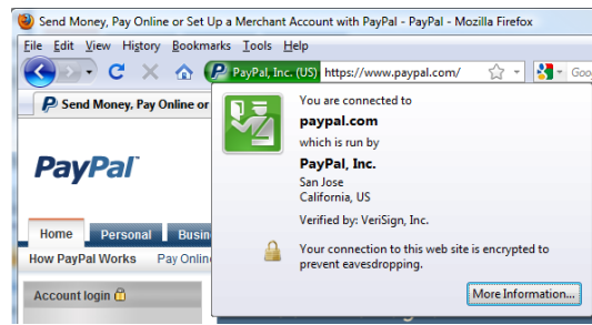
Fig. 2 User interface for EV SSL certificates in Firefox.
