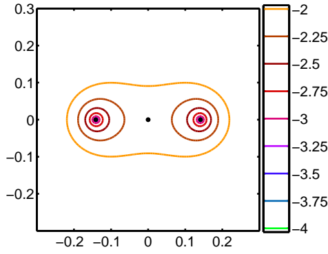
(b) Skew-symmetric pseudospectrum
