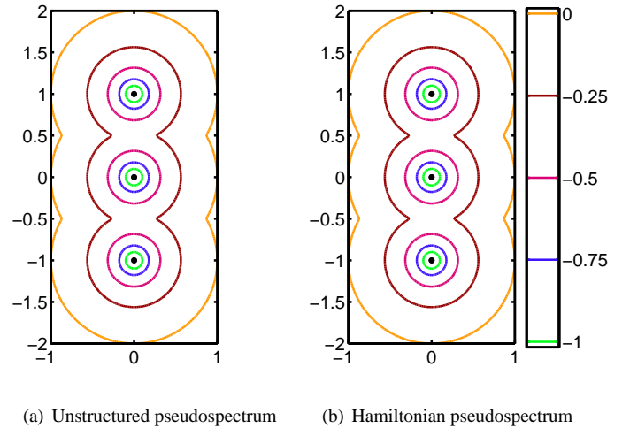
Figure 6: Pseudospectra of the matrix (31)
