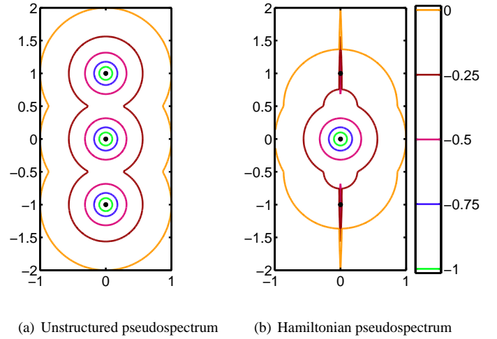
Figure 5: Pseudospectra of the matrix (30)
