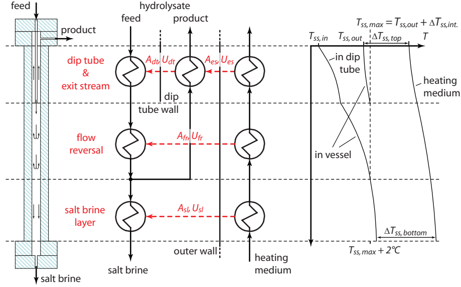
Figure 3: Schematic of the salt separator and its heat transfer model representation
