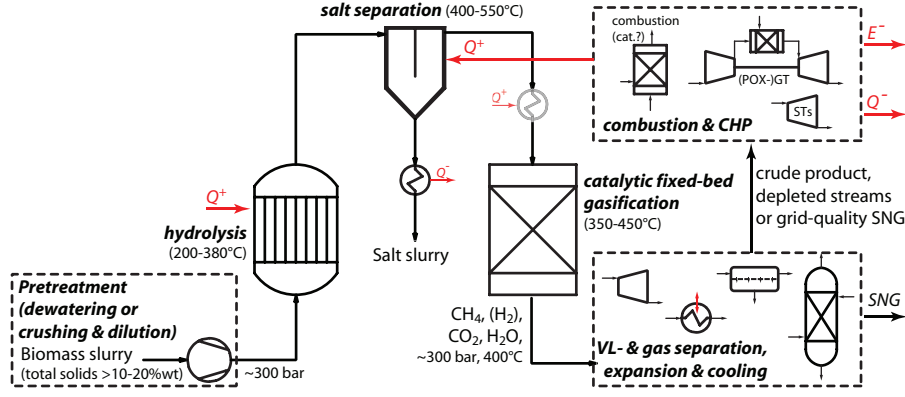
Figure 1: Conceptual process flow diagram for hydrothermal gasification in supercritical water
