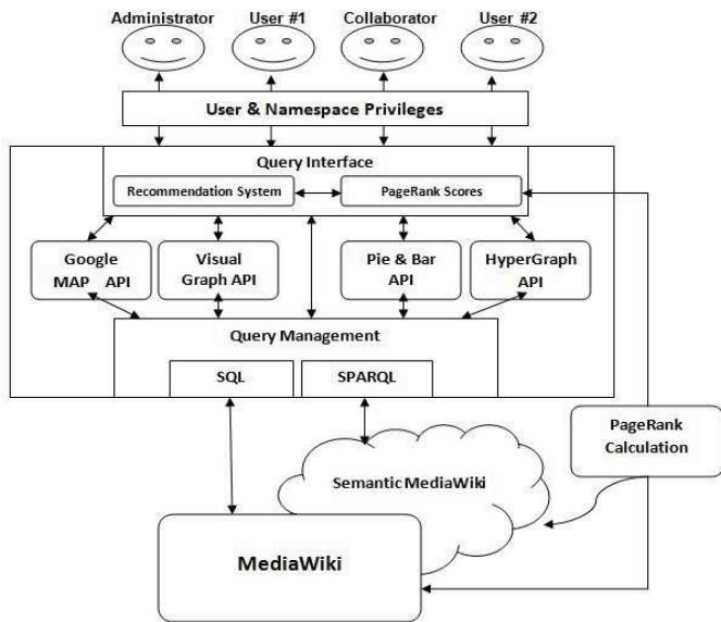
Fig. 1. System architecture.
