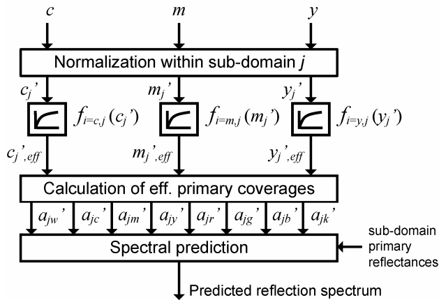
Figure 3. Cellular Yule-Nielsen model accounting for ink spreading.
