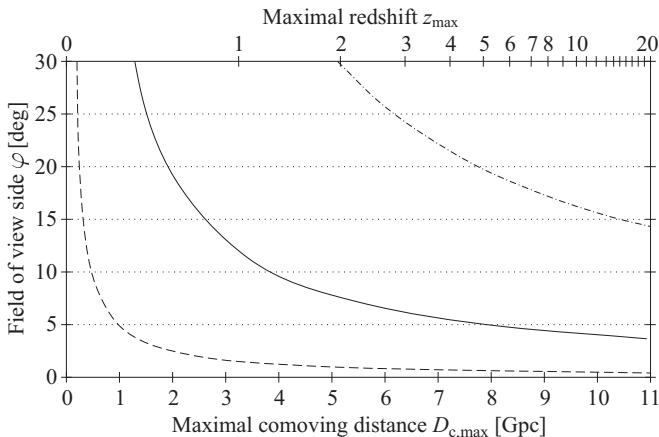
FIG. 2.— Relation between the maximal comoving distance D_{C,\max} or maximal redshift z_{\max} and the opening angle \varphi of the mock observing cone. The different lines correspond to the box sizes of the Millennium Simulation (solid), the Milli-Millennium Simulation (dashed), and the Horizon- 4\pi Simulation (dash-dotted).
