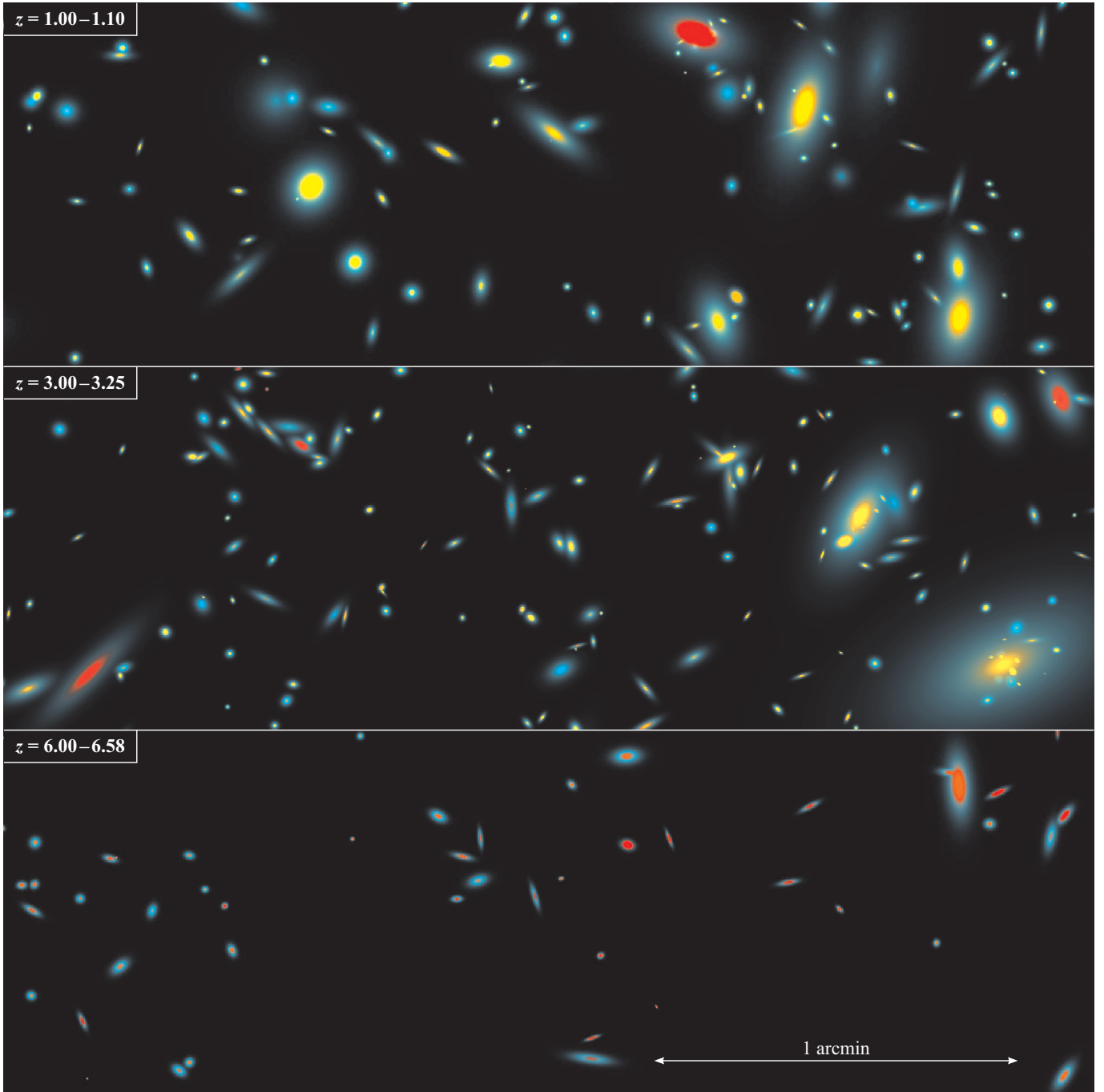
FIG. C1.— Simulated sky field covering 3 \times 1 \text{ arcmin}^2 . The three panels correspond to three different redshift slices, with an identical comoving depth of 240 Mpc. The coloring is identical to Fig. 4, but the flux scales are 10-times smaller at z = 3 and 100-times smaller at z = 6 .
