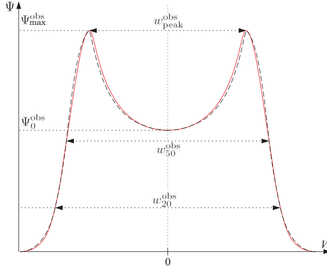
FIG. A1.— Comparison of a simulated normalized emission line \Psi(V) (solid line) with the emission line \Psi_{\text{approx}}(V) (dashed line), recovered from the five parameters \Psi_0^{\text{obs}} , \Psi_{\text{max}}^{\text{obs}} , w_{\text{peak}}^{\text{obs}} , w_{50}^{\text{obs}} , and w_{20}^{\text{obs}} .
