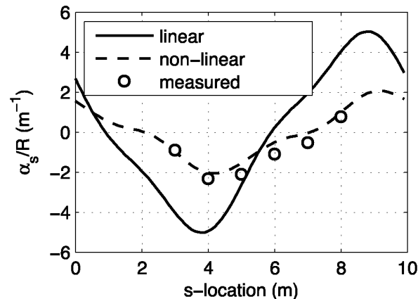
Figure 3. Transverse flow structure for the Kinoshita shaped meander flume calculated by the linear and non-linear hydrodynamic models and compared to measurement data.
