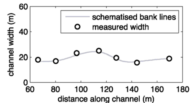
Figure 5. Width along the Tollense River (Schnauder & Sukhodolov, 2010).
