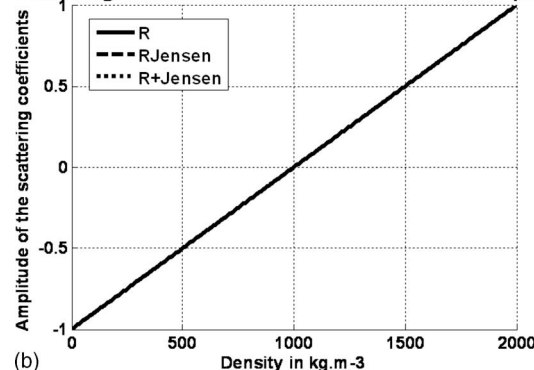
FIG. 2. Illustration of the dependence of the relative bulk modulus scattering coefficient R on changes in speed of sound (a) and density (b) separately, compared to the values provided by the Jensen coefficient R_{\text{Jensen}} (Ref. 8) and its modified version R_{\text{Jensen}}^+ .
