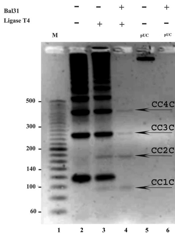
Figure 7. Bal31 nuclease detects a destabilized duplex DNA structure in covalently closed supercoiled DNA molecules but does not reveal the presence of kinks in 94-bp covalently closed DNA minicircles. A 2.5% agarose gel run in the presence of ethidium bromide (0.5 µg/ml) reveals that while negatively supercoiled DNA (lane 6) and nonligated nicked rings are completely digested by Bal31 nuclease (see lanes 2–4), the covalently closed monomeric, dimeric, trimeric and tetrameric circles (indicated with arrows) remain resistant to action of Bal31 nuclease (compare lanes 4 and 3).
