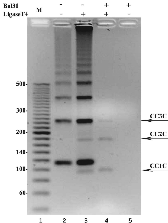
Figure 2. The formation and purification of 94-bp-long covalently closed DNA minicircles. A 2.5% agarose gel run in the presence of ethidium bromide (0.5 \mu\text{g/ml} ) reveals that after the ligation reaction of minicircles with nicks, new species appear on the gel (compare lanes 3 with 2). Only these new species resist digestion by Bal31 (lane 4) indicating that they are covalently closed DNA molecules. The electrophoretic migration of these new species is as expected for monomeric, dimeric and trimeric rings that acquired writhe due to ethidium bromide intercalation to covalently closed DNA molecules.
