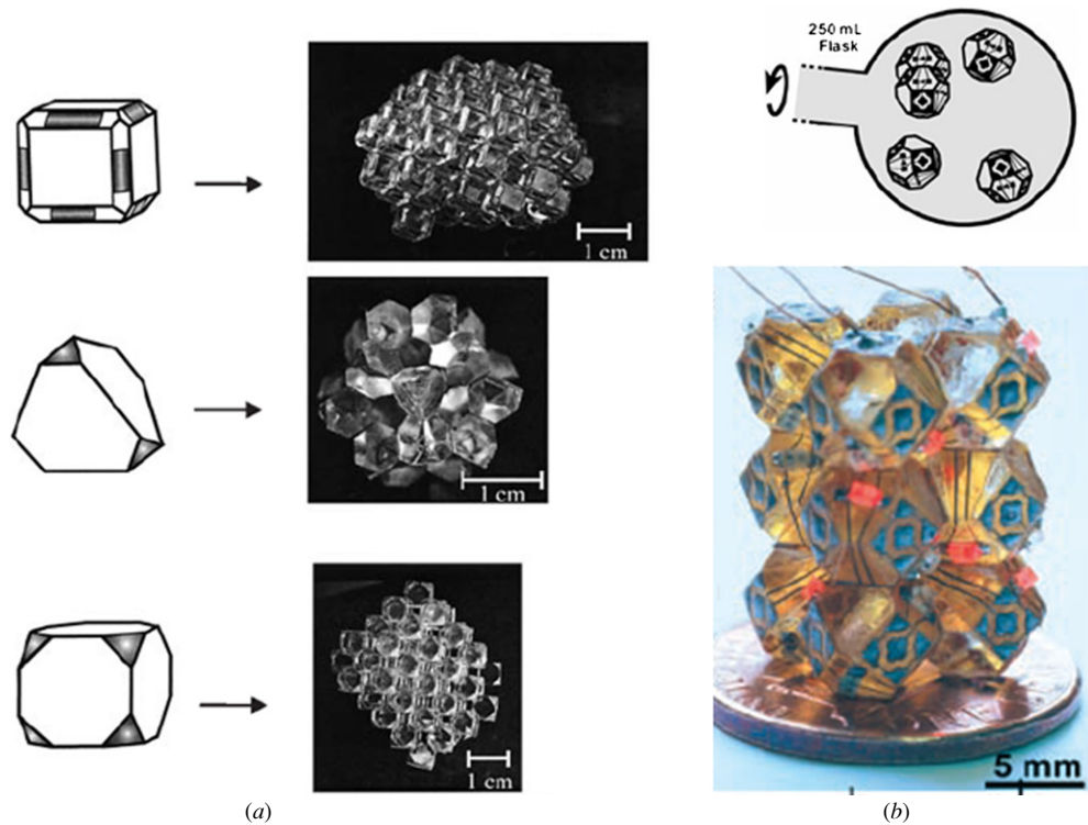
Figure 9. (a) Open lattice structures formed by self-assembly of polyhedra having selected faces coated with liquid alloy by agitation in an aqueous potassium bromide solution. (Reprinted from [57], with permission from AAAS.) (b) Self-assembled structure of polyhedra with electronic circuits and LEDs. Two electrically isolated pairs of wires connected to a battery illuminated six LEDs in an electrically continuous loop. (Reprinted from [59], with permission from AAAS.)
