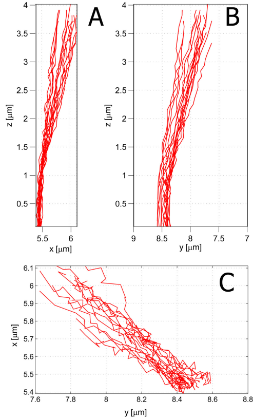
Figure 15: Three-dimensional coordinates of the cilium shown in Fig. 14 were obtained by image processing. The fluctuations are more pronounced in the y direction than in x, and apparently higher at the tip than at the base.
