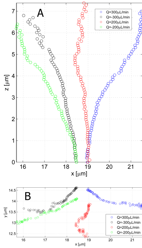
Figure 18: Coordinates of a cilium exposed to different flow rates with (A) showing the side view and (B) the top view. The cilium deflects under flow, and it looks as if the base rotates in the xy -plane.
