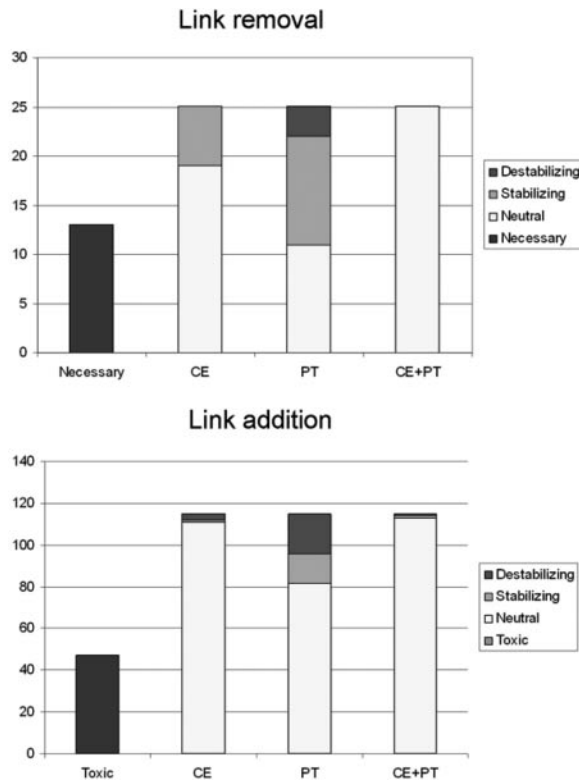
Fig. 6. Link classification according to functional categories. Top: Removed links are necessary, neutral, stabilizing or destabilizing depending on their effect on CE, PT or both. In the latter category, all links are either necessary or neutral. More than two-thirds of the 30% necessary links are inhibitory (Supplementary Table 1). Bottom: Added links can be toxic, neutral, stabilizing or destabilizing. Nearly all toxic links are activating (Supplementary Table 2).
