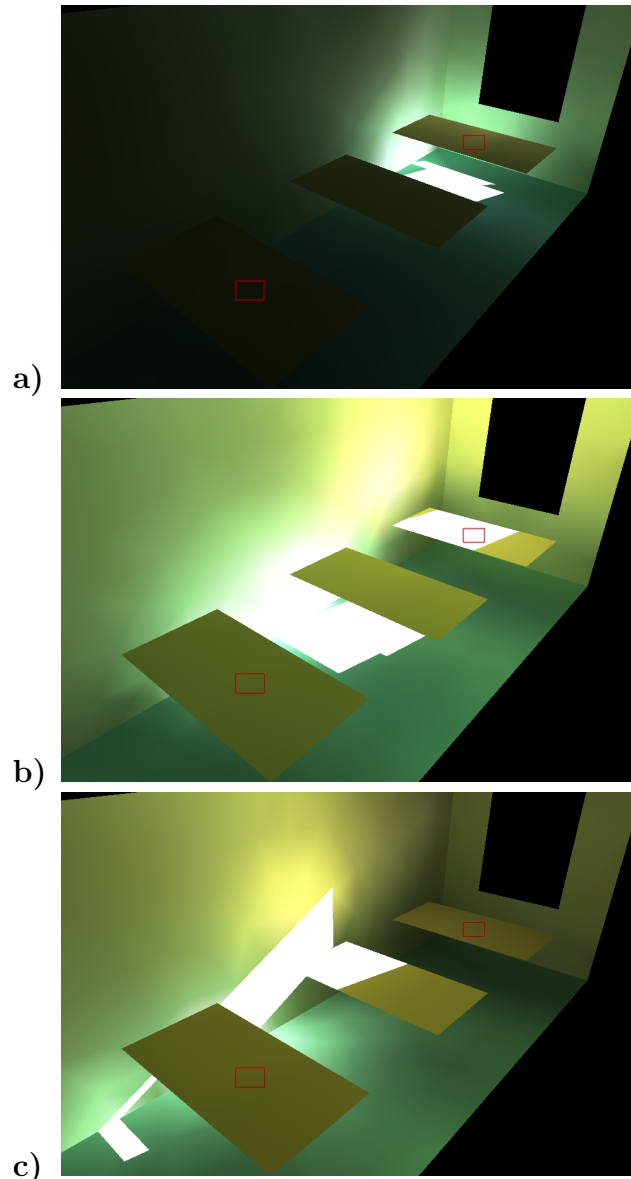
Fig. 9. A simple office scene with a single southern-facing window. The designer uses daylighting optimization to select an appropriate fenestration material to more uniformly illuminate the desks nearest and furthest from the window (outlined with small red squares). The optimization process is shown in Figure 10.
