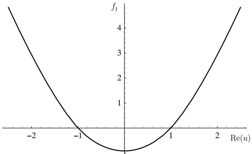
Fig. 1. Fig. 1. Potential induced by a soft scalar mass m_{\phi_0}^2 .
