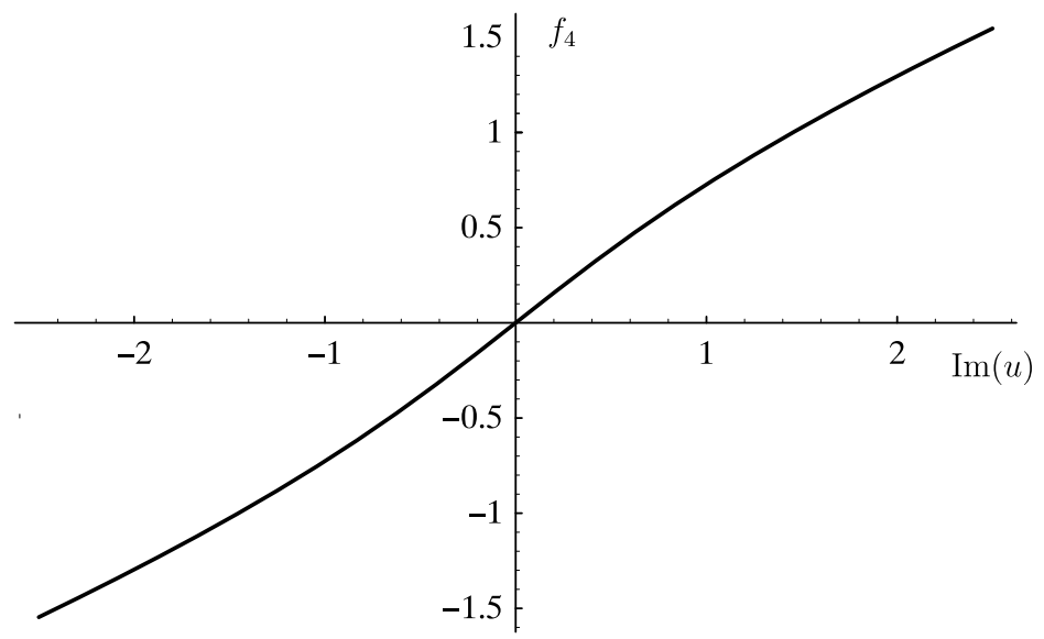
Fig. 4. Fig. 4. Potential induced by \text{Im}(\Delta_0) , where \Delta_0 is the determinant of the fermion mass matrix.
