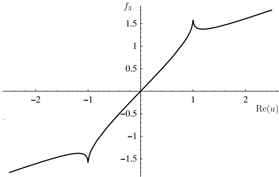
Fig. 3. Fig. 3. Potential induced by \text{Re}(\Delta_0) , where \Delta_0 is the determinant of the fermion mass matrix. The potential approaches a finite value at the cusp singularities at the monopole/dyon points u = \pm 1 .
