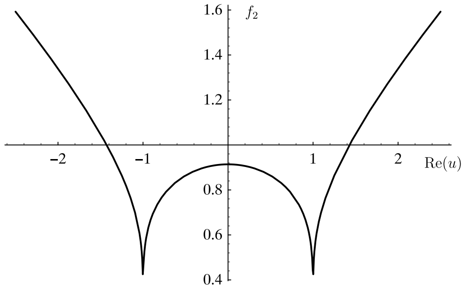
Fig. 2. Fig. 2. Potential induced by the trace of the fermion mass matrix T_0 . The potential approaches a finite value at the cusp singularities at the monopole/dyon points u = \pm 1 .
