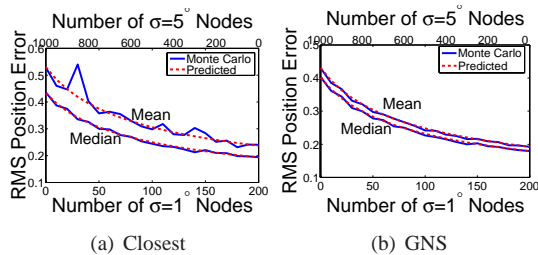
Figure 2. Comparison of theory and Monte Carlo simulations
