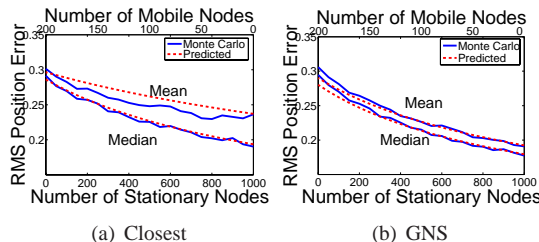
Figure 4. Localization performance of a mixed network
