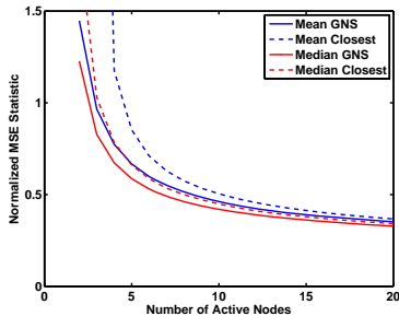
Figure 1. The MSE localization performance
