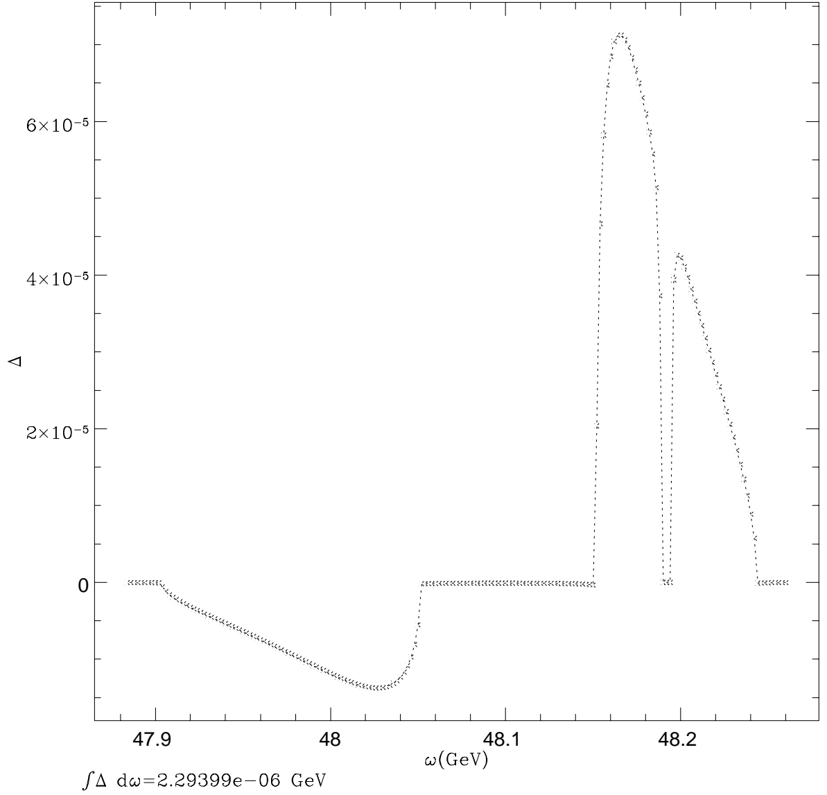
Figure Caption: \Delta , the asymmetry in the reflection probabilities of right-chiral quarks and antiquarks incident from the unbroken phase, for zero wall velocity.
