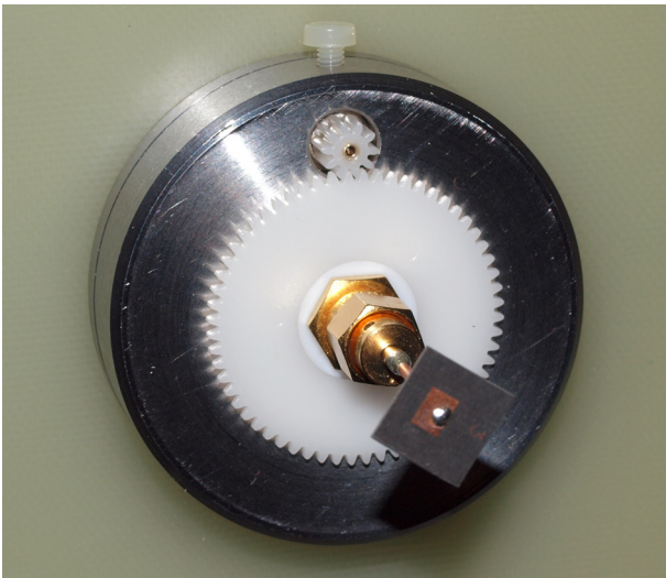
Figure 6: the second rotary joint with a 30 GHz patch (outer diameter of the device: 50 mm)
