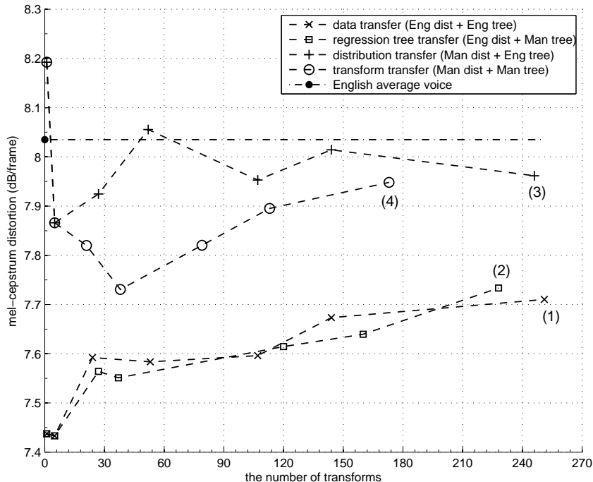
Figure 2: MCD comparison (cross-lingual speaker adaptation with 100 adaptation utterances)
