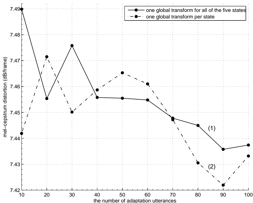
Figure 3: MCD comparison (data transfer with the number of transforms fixed)
