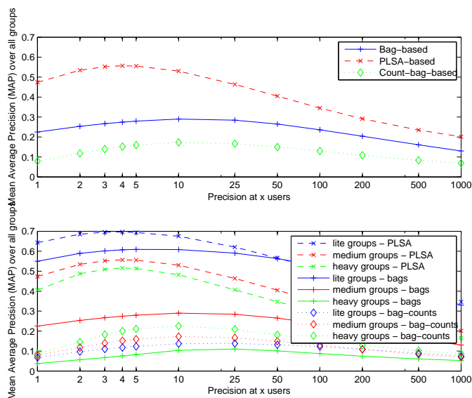
Fig. 13. Mean Average Precision for the user retrieval experiment, computed separately for lite, medium and heavy groups in terms of user memberships. Lite groups are in the first quartile (less than 12 users), medium groups in the second and third quartiles (12 to 49 users) and heavy groups in the fourth quartile (more than 49 users).
