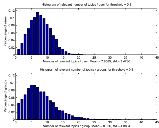
Fig. 6. Comparison of the number of relevant topics for groups and users. For ease of comparison, we normalized the histograms and display on the y axis the percentage of users and groups respectively.
