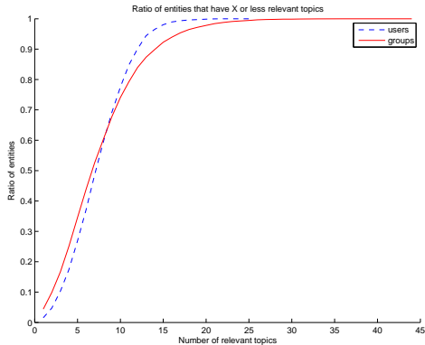
Fig. 7. Ratio of either type of entities that are about x or less topics. For example, 60.2% of groups and 59.3% of users are about at most 8 topics.
