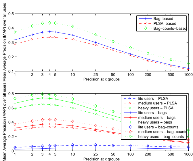
Fig. 14. Mean Average Precision for the group retrieval experiment, computed separately for light, medium and heavy users in terms of group membership. Lite users are in the first quartile (less than 10 groups), medium users in the second and third quartiles (10 to 91 groups) and heavy users in the fourth quartile (more than 92 users).
