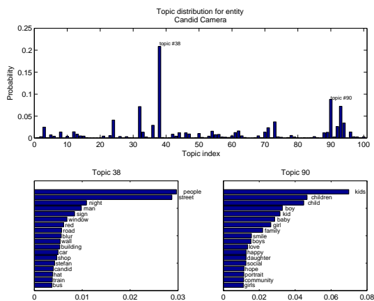
Fig. 5. Topic distribution for the entity Candid Camera (a Flickr group). In the lower part of the figure, the two most relevant topics, described by their top most probable tags. Topic 38 could be described by the concept “street portraits” and topic 90 by “children”.
