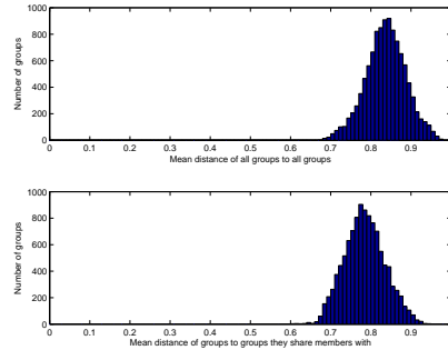
Fig. 8. Distributions of the mean distances from each group to all groups, or to just groups who share at least one member. We observe a significant shift in distances when only “overlapping” groups are considered.
