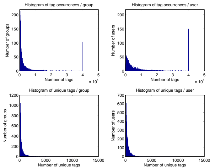
Fig. 2. Top half: histograms of the total number of tag occurrences per group and per user; bottom half: histograms of the number of unique tags per group and per user
