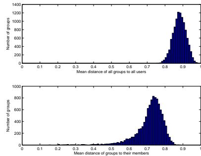
Fig. 10. Distribution of the mean distances from all groups to all users, or to just member users. We observe a distinct difference, explained by the fact that members' representations are closer to that of the group they belong to than those of users who do not belong to the group.
