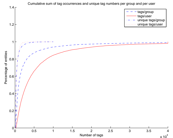
Fig. 3. Cumulative sums of the total number of tag occurrences and unique tags for groups and users respectively; 66.2% of the users and 87.3% of the groups have less than 5,000 tag occurrences, but in terms of unique tags the two types of entities are very similar.
