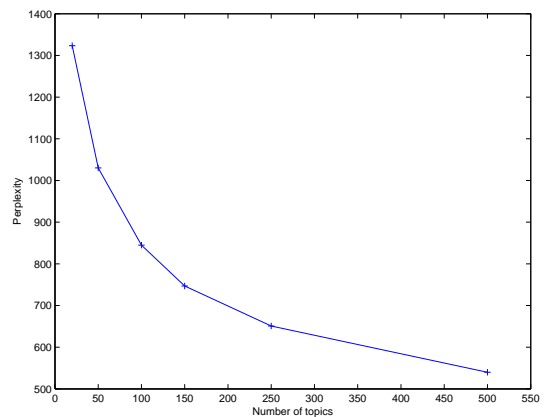
Fig. 4. Variation of the perplexity with respect to the number of topics learned by the model. The + markers show the perplexity values for each N_z in the set \{20, 50, 100, 150, 250, 500\} . Perplexity decreases with the increase in number of topics.
