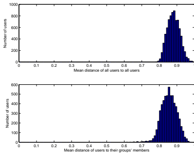
Fig. 9. Distribution of the mean distances from all users to all users, or to just users whom they share at least one group with. We observe a clear difference between the two histograms, the distances between users who are part of the same groups are smaller on average than those between all users.
