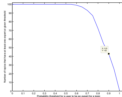
Fig. 12. The number of topics that have at least one topic-expert, varying with the topic-expert's probability for the given topic. In this model, 93 topics out of 100 have at least one entity whose probability for that topic is higher than 0.7 and 43 topics out of 100 have at least one entity whose probability is higher than 0.9.
