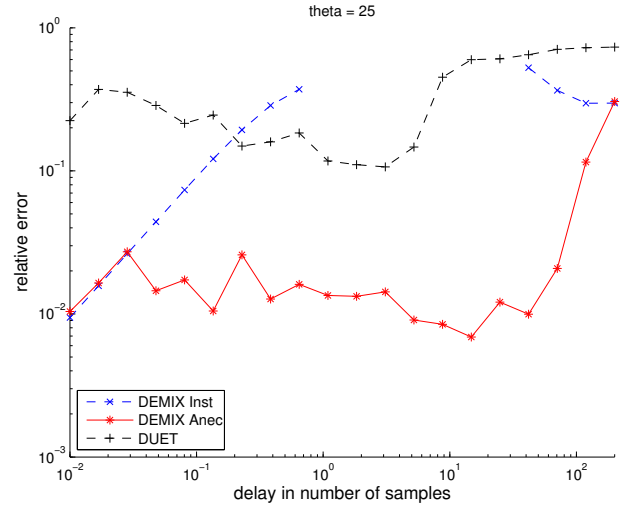
(a) angular distance between IP is \Delta\theta = 25 degrees.
