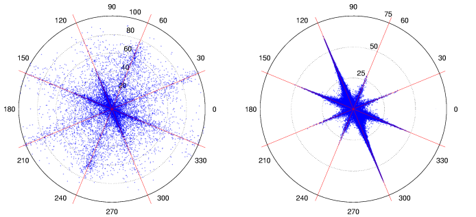
(a) Real-valued global scatter plot of points \mathbf{X}^{\mathbb{R}}(t, f) / \|\mathbf{X}^{\mathbb{R}}(t, f)\| weighted by their energy \rho^2(t, f) = \|\mathbf{X}^{\mathbb{R}}(t, f)\|^2 . (b) Scatter plot of points \hat{\mathbf{u}}(\Omega_{t,f}) weighted by their confidence measure 10 \log_{10} \hat{\mathcal{T}}(\Omega_{t,f}) . Neighborhood size is |\Omega_{t,f}| = 10 .
