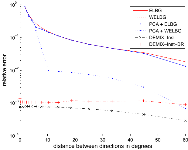
Fig. 6. Relative mean direction error (RMDE) as a function of the angular distance in degrees ( \Delta\theta ) between the 3 directions for DEMIX-Instantaneous (DEMIX-Inst), its variant DEMIX-Instantaneous-BR (DEMIX-Inst-BR) and the best instance (over 10) of the four variants of the ELBG
