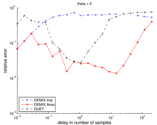
(b) angular distance between IP is \Delta\theta = 5 degrees.
