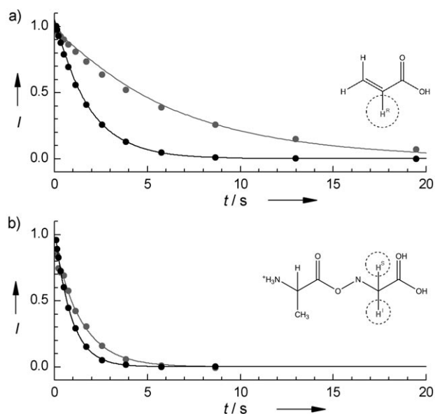
Figure 3. Transverse relaxation times T_2 (actually T_{1p} determined by spin locking.) a) The proton H R in acrylic acid in D 2 O with 2.5 mM TEMPOL without scavenger (●, T_2 = 1.802 \pm 0.014 s) and after addition of 30 mM sodium ascorbate (●, T_2 = 6.29 \pm 0.15 s). b) The two diastereotopic protons H I and H S of glycine in L-Ala-Gly in D 2 O with 2.5 mM TEMPOL without scavenger (●, T_2 = 0.875 \pm 0.008 s) and after addition of 30 mM sodium ascorbate (●, T_2 = 1.43 \pm 0.095 s).
