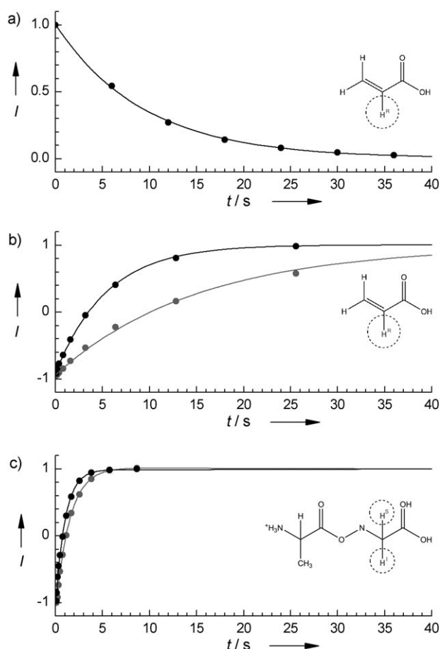
Figure 2. a) Decay of the hyperpolarized magnetization of proton H R ( T_1 = 9.36 \pm 0.12 s) in acrylic acid ( \text{CH}_2=\text{CH}^{\text{R}}\text{COOH} ), measured 4.5 s after dissolution with hot D 2 O of a mixture of frozen beads of acrylic acid containing TEMPOL and frozen beads of 3 M sodium ascorbate (vitamin C). b) Inversion recovery without DNP of proton H R in acrylic acid in D 2 O with 2.5 mM TEMPOL without scavenger (●, T_1 = 5.35 \pm 0.1 s) and, again without DNP, after addition of 30 mM sodium ascorbate (●, T_1 = 14.9 \pm 0.8 s). c) Inversion recovery without DNP of the two diastereotopic protons H I and H S of glycine in L-Ala-Gly in D 2 O with 2.5 mM TEMPOL without scavenger (●, T_1 = 1.01 \pm 0.05 s) and after addition of 30 mM sodium ascorbate (●, T_1 = 1.47 \pm 0.05 s).
