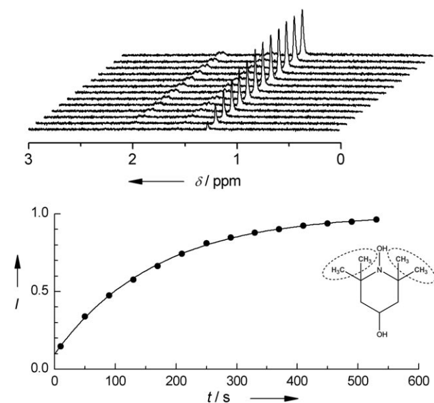
Figure 1. Slow reaction of 2.5 mM TEMPOL with 30 mM sodium ascorbate in \text{D}_2\text{O} (much less than in the actual DNP experiments) at T=296\text{ K} in a magnetic field B_0=7.05\text{ T} (300 MHz for protons). The singlet at \delta=1.28\text{ ppm} that arises from the four degenerate methyl groups in diamagnetic TEMPOL-H (●) appears only after reduction of the paramagnetic TEMPOL.
