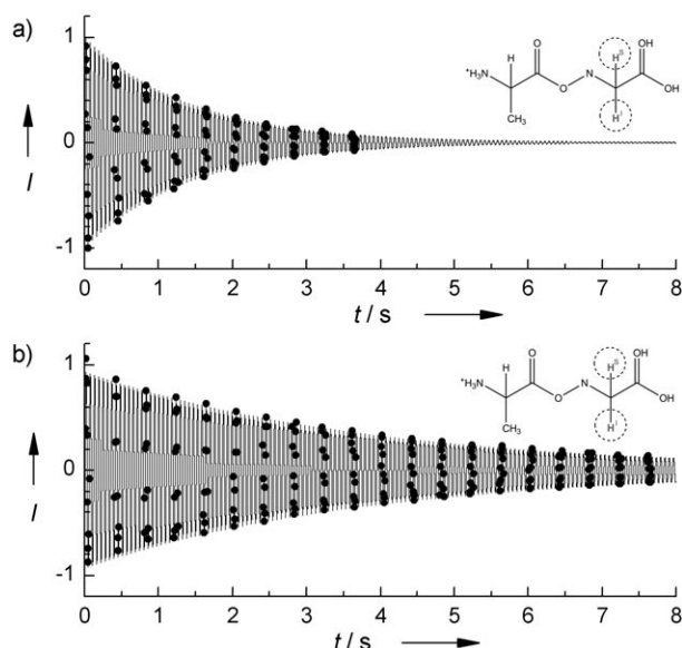
Figure 5. a) The decay of the long-lived coherence (LLC) involving the two protons H^1 and H^5 of glycine in L-Ala-Gly is affected by the presence of 2.5 mM TEMPO ( T_{LLC} = 1.43 s). b) After addition of 30 mM sodium ascorbate, the lifetime ( T_{LLC} = 3.82 s) is extended by a factor of 2.7. Both signals were measured at T = 296 K and B_0 = 7.05 T without DNP and fitted with mono-exponential decays multiplied by a sine functions. The modulation arises from the scalar coupling constant J = -17.242 Hz.
