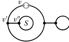
Figure 8: The set of singularities E_7 \oplus 2A_6
