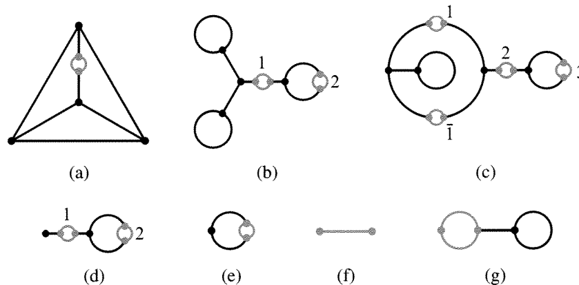
Figure 5: The skeletons Sk' and Sk
