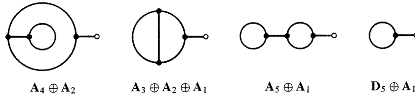
Figure 11: Perturbations of E_7 with nonabelian fundamental group
