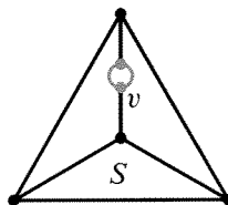
Figure 9: The set of singularities E_7 \oplus 2A_4 \oplus 2A_2
