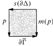
Figure 2: The square spanned by p
