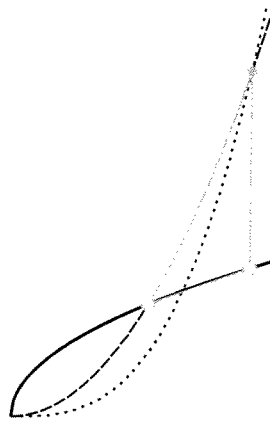
Figure 3: Computing the inclusion homomorphism
