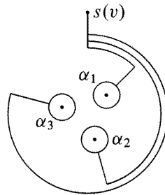
Figure 1: The canonical basis
