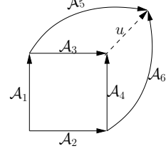
Fig. 4: The pushout property.
