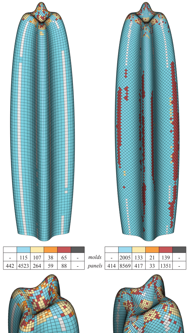
Figure 10: Paneling solutions for different curve networks on the Liliun tower. Significant changes in the curve network layout result in different paneling solutions. The left curve network, being closer to a conjugate network [Pottmann et al. 2007], is better suited for rationalization with planar and single curved panels.
