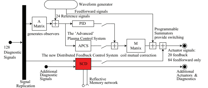
Fig. 7. Simplified schematic of the TCv central magnetic control systems. The ability to switch between controllers (between shots) is provided by programmable summaters. All the hybrid input signals are replicated for the SCD controller together with the addition of other input signals. The outputs are passed through the summaters, to provide switching between the control systems.
