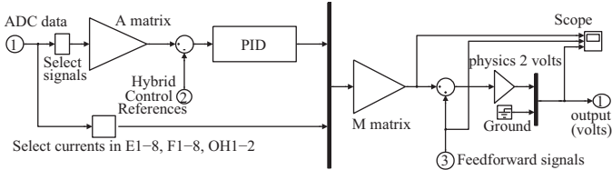
Fig. 6. Simulink diagram of the matrix operations and PID controller in the TCV Hybrid control algorithm. The Scope provides the capability to analyze various signals in the algorithm, either before or post-shot using the actual real time data acquired by the system and stored in the MdsPlus [7] tree.
