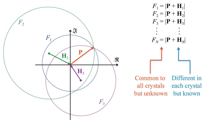
Figure 2 The Harker construction. In the example given the first ‘derivative’ is a native crystal, so that \mathbf{H}_1 = 0 .
