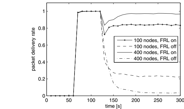
Fig. 8. Flooding attack resilience. The attack begins at the 120s mark. The five 4pkt/s flows begin at 60s. The curves are averages over 50 independent randomly seeded runs.
