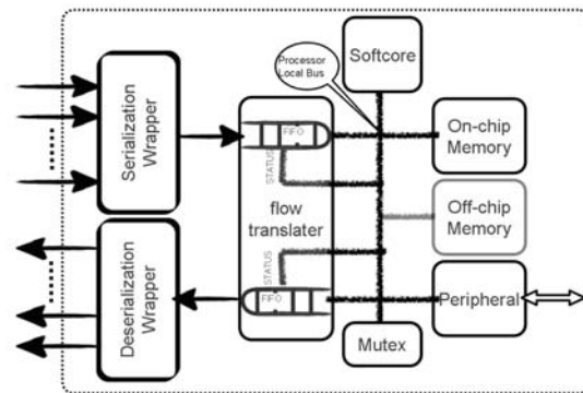
Figure 9: Wrapper overview
