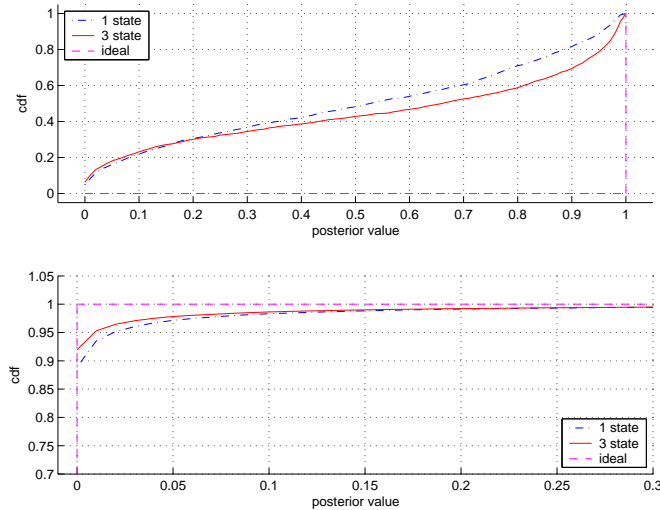
FIG. 1 – CDF of posterior probability of phoneme /uw/ when phoneme /uw/ is said (top) and when other phonemes are said (bottom).
