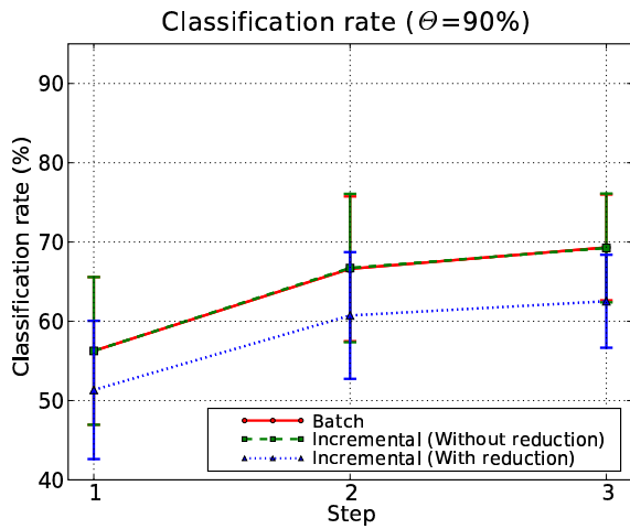
Figure 3. Results on the TIPS2 database obtained using batch SVM, the fixed-partition incremental method, and the memory controlled incremental algorithm.
