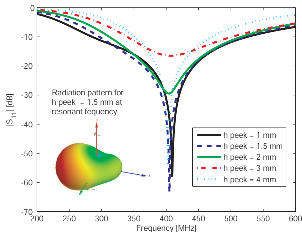
Fig. 9. Simulated |S_{11}| variation due to different insulation thicknesses and 3D radiation pattern of the final design.
