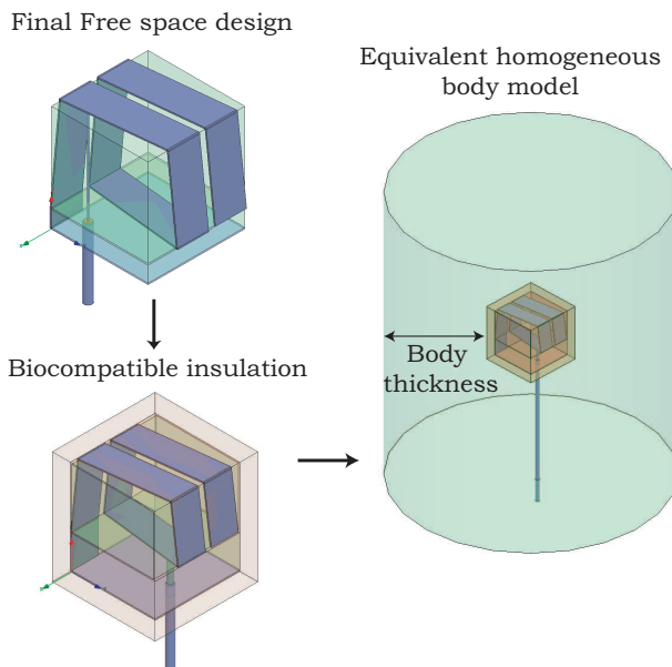
Fig. 8. Scheme of the introduction of the insulation layer and the equivalent body model.
