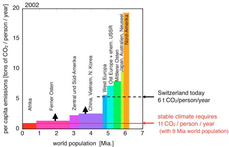
Figure 2: Per capita emissions are very different depending on the continent we look at. With a population approaching 9 Mia persons by 2050 the emissions must fall below about 1 ton of CO 2 per person per year to reach a stable climate. [2]
