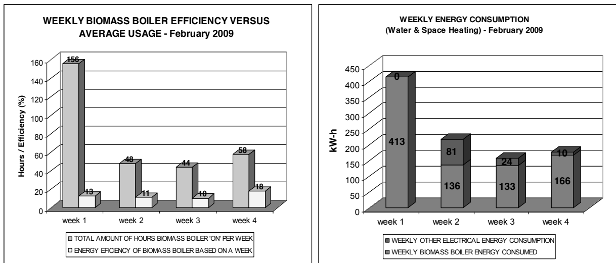
Figure 3 (left) Weekly Biomass Boiler Efficiency versus Average Usage. And Figure 4 (right) Appliance's comparison of weekly energy consumption for water and space heating.
