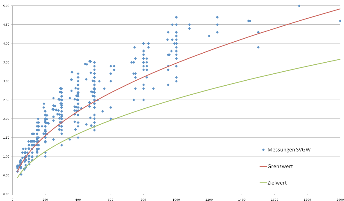
Figure 2: Overview of the heat losses of factory-insulated hot water stores, measured in the testing laboratory since the beginning of the mandatory tests (1992) imposed by Swiss legislation. The heat losses recorded within 24 hours under a 45 K temperature difference between store water and store surrounding air is plotted, in kWh/24 h, as a function of the nominal store size, in litres. Each of the 776 tested stores is represented by one data point [4]. From 200 to 500 litres, 0.1 kWh/24 h and 100 l of tank content have been subtracted from the measured value, and 0.3 kWh/24 h in the range 500-2000 litres, this in order to eliminate the additional heat losses caused by connection pipes (assumption: 0.1 kWh/24 h for each additional connection pipe; base case: 2 connection pipes as in the range < 200 l). Also shown are the proposed curves for threshold and target values of the heat losses, respectively. They imply 2 connection pipes in the whole size range.
