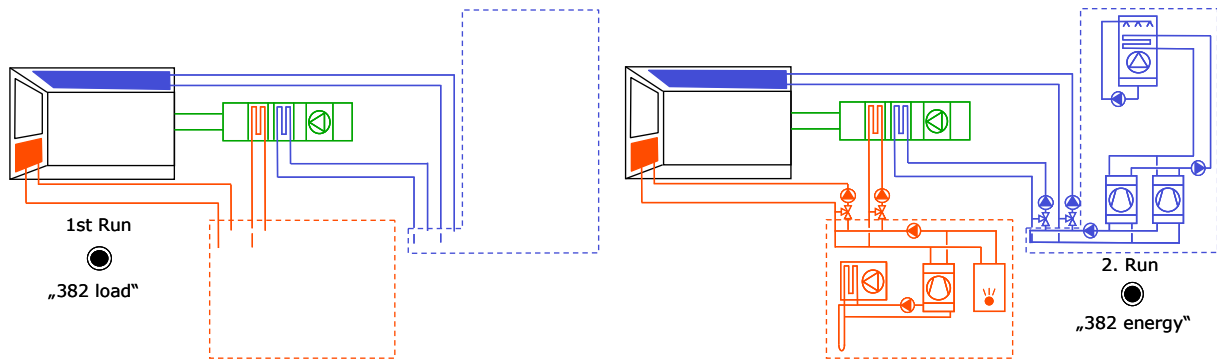
Figure 3: System schematics at the load calculation level (left) and the system calculation level (right)
