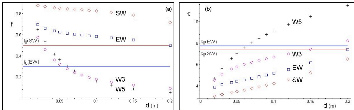
Figure 2 – M=M_{lim}/2 , the trend of the decrement factor f (Fig. 2a) and of the time lag \tau (Fig. 2b) with the insulating thickness d (m), for the four considered walls.
