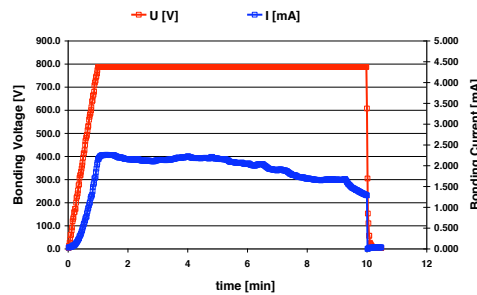
Figure 3b: I/V profile of SnAl anodic bonding (300°C)
