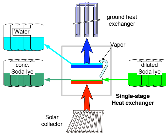
Figure 3: Charging mode. Weak sodium hydroxide is pumped to the heat exchanger and concentrated. Water and concentrated soda lye are stored separately.
