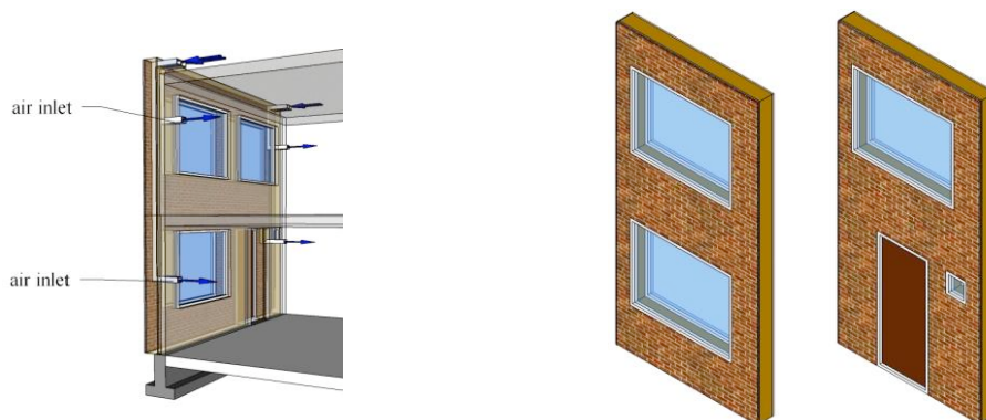
Figure 1: Visualization of the +Facade-elements with piping for ventilation and air inlet (left) and the vertical orientation of the elements (right).
