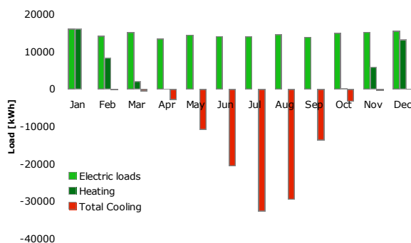
Figure 4: Monthly energy demand for heating, cooling and electricity. High-efficiency case.
