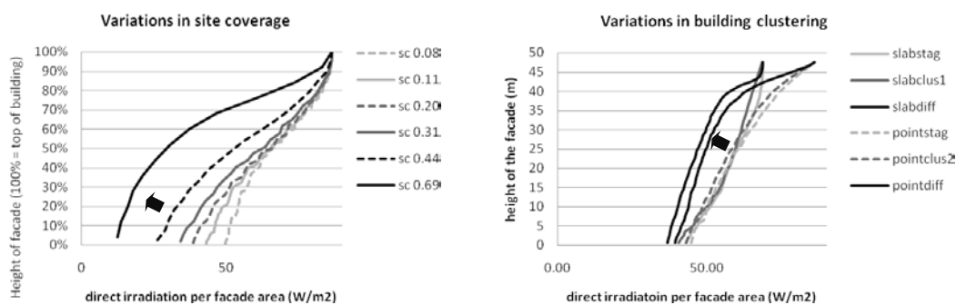
Figure 10: Vertical position on the façade vs. direct solar irradiation ( W/m^2 ) on building façades of the central block under the Abu Dhabi sky
