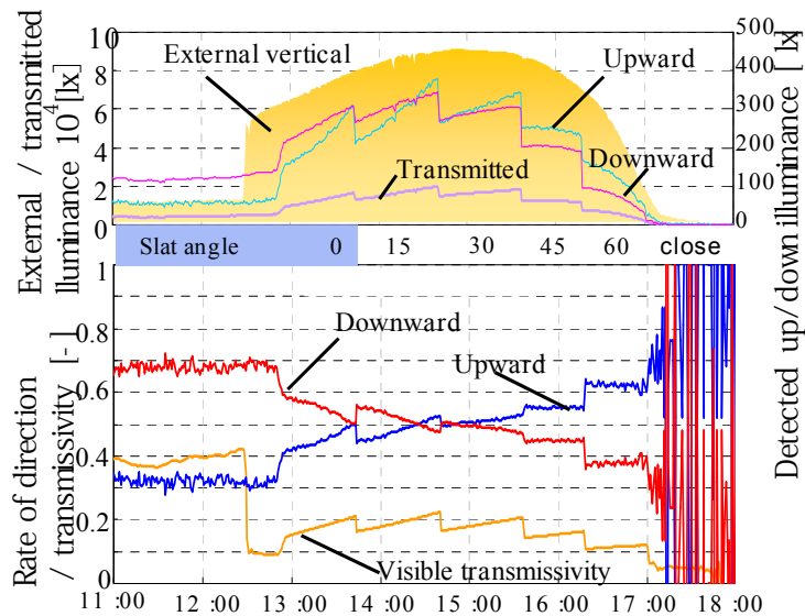
Figure 14: Intensity and ratio of upward / downward of transmitted light through windows.
