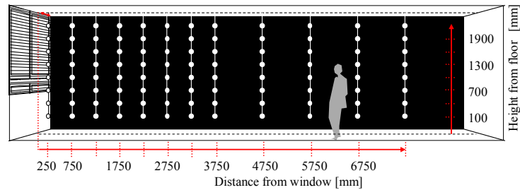
Figure 8: Sectional layout of white globes in the study room.
