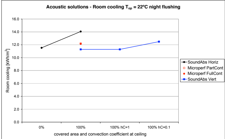
Figure 1: Cooling energy demand for various acoustic solutions, with set-point of 22°C and night flushing
