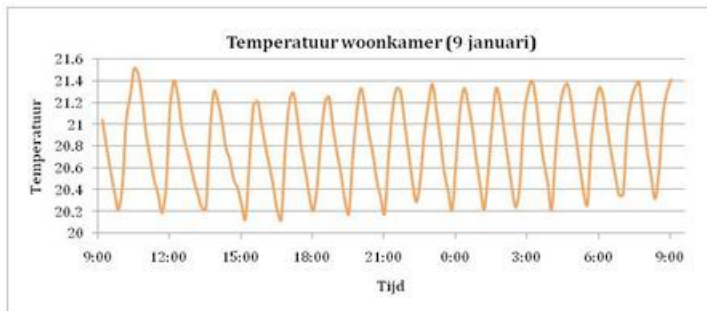
figure 3: Oscillating room temperature due to oversized boiler capacity.
