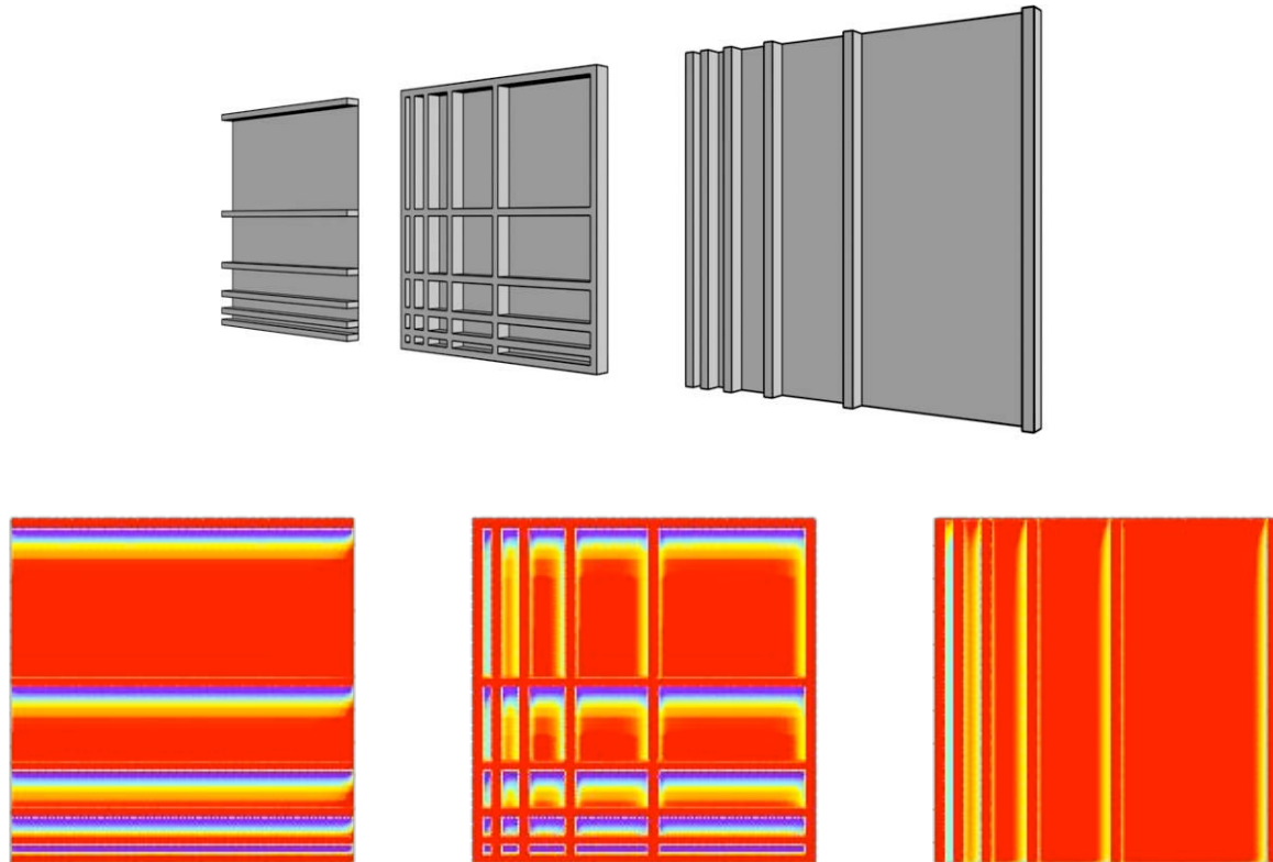
Figure 8: SOLARCHVISION front view analysis for west facade in Najaf which shows the suitable type (horizontal) and proportion (depth = 2 * height) of louvers.
