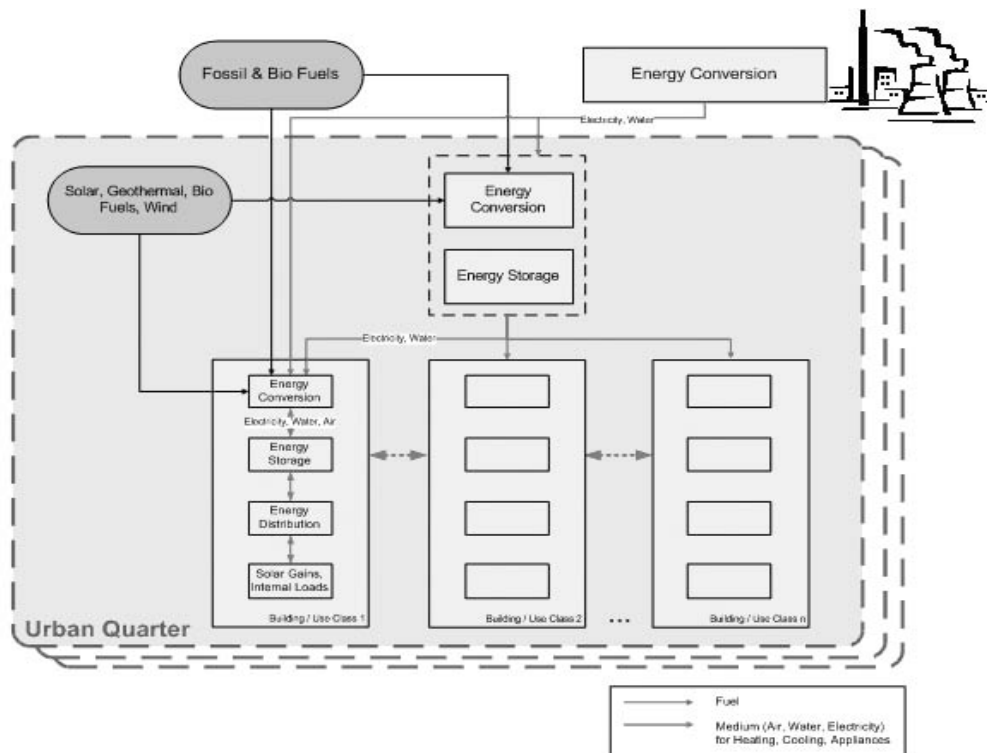
Figure 2: Schematic depiction of the energy demand and supply structure of an urban quarter
