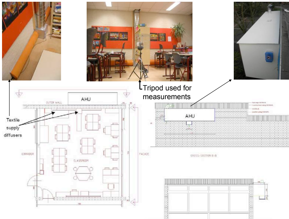
Figure 1: Experimental set-up ventilation system [11]
