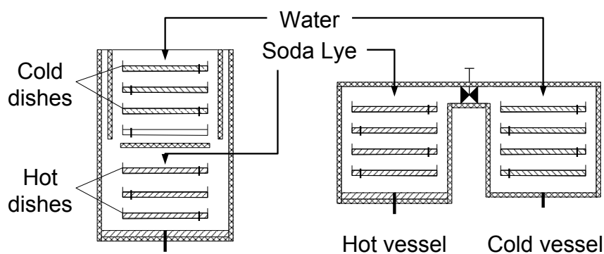
Figure 5: Left side: First version heat exchanger (still used as the first stage). Right side: Improved heat exchanger (used as the second stage).
