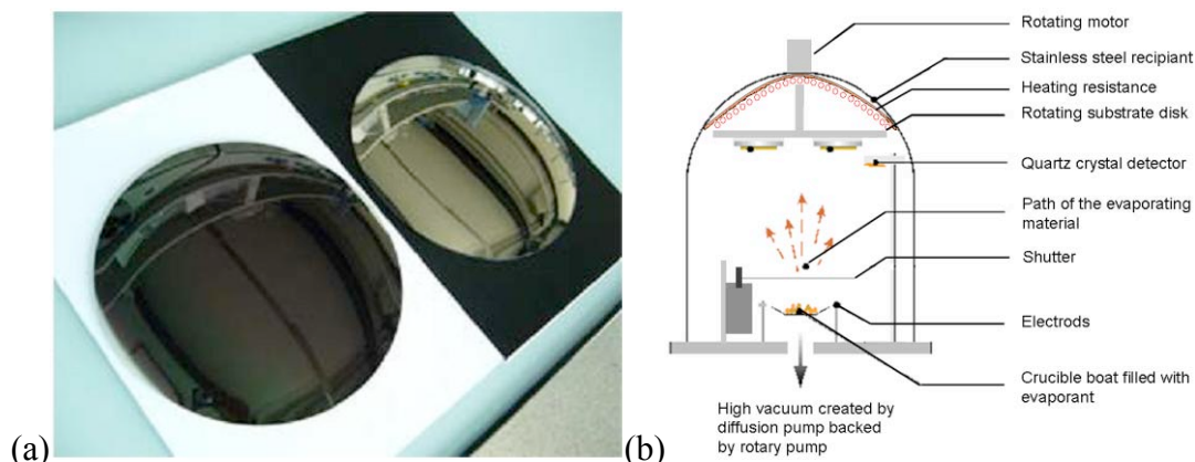
Figure 1: (a): Black absorbing VO x (left) and mirrorlike film samples (right). (b): a schematic representation of the thermal evaporator used for our experiences.
