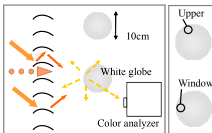
Figure 11: Measuring procedure of spatial distribution.
