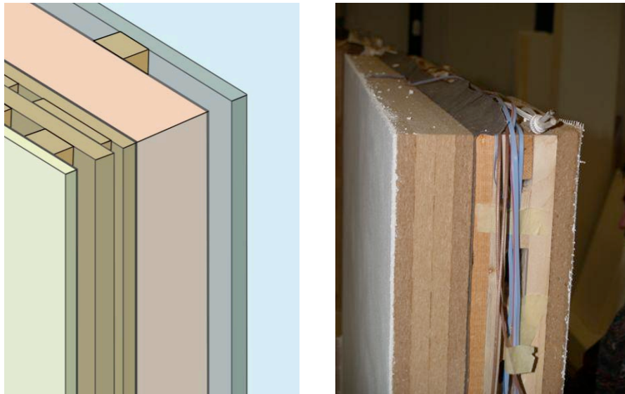
Figure 1: Schematic make-up of the system (left) and real wall specimen with temperature and humidity sensors at different depth (right).
