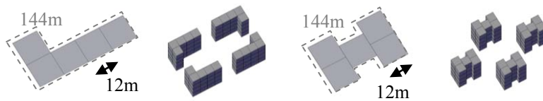
Figure 1: Constructing standardised “courtyards” and “point towers” with 12x12m squares
