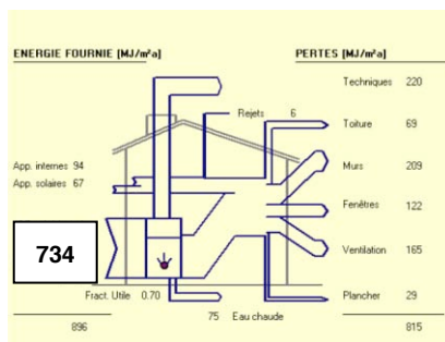
Figure 4: Before refurbishment, the building consumption for heating and hot water is 734 MJ/m 2 (class G). After refurbishment, energy consumption according to standard conditions is reduced to 164 MJ/m 2 . Although after refurbishment airflow is drastically reduced, the part of ventilation losses, according to standard conditions, represents 41% of total losses.
