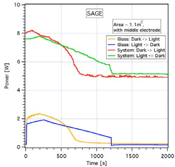
Figure 8: Power consumption of the SAGE glass during the switching of one colour state to the other and afterwards keeping this status.
