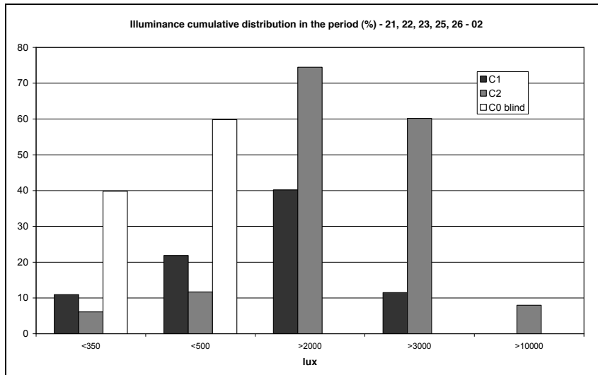
Figure 4: Illuminance cumulative distribution for C0 with blind, C1, C2.
