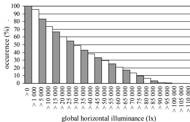
Figure 6: Percentage occurrence of global horizontal illuminance in April in Bratislava
