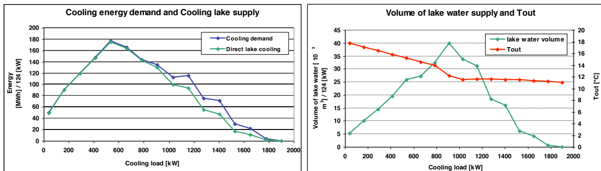
Figure 5. Cooling supply by the lake (left) and corresponding volumes by increasing cooling demand steps (right)
