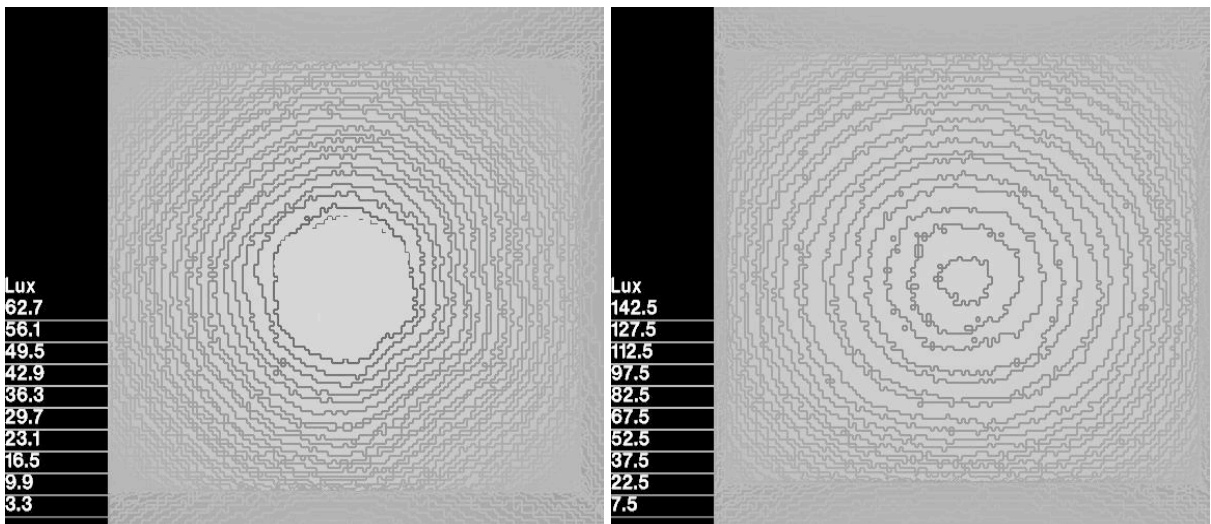
Figure 2: On the left the skylight and on the right the lightpipe isolux on May at 12 p.m..
