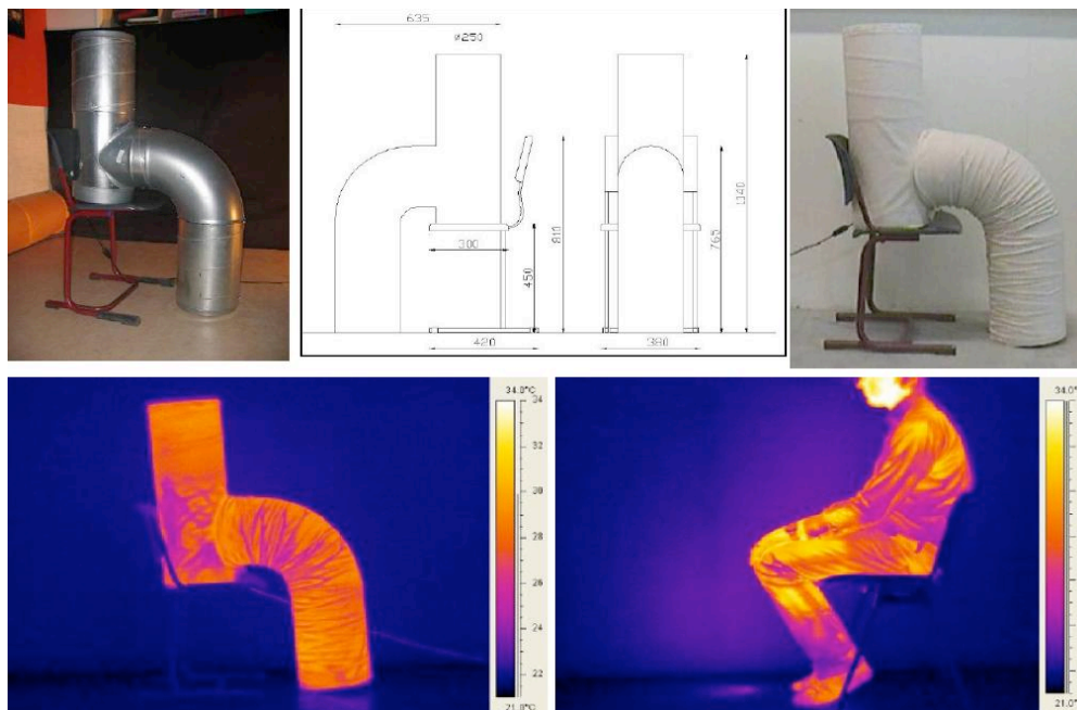
Figure 2: Undressed person simulator, its dimensions, the dressed version and the thermo graphical check by comparing the person simulator with a person [11]
