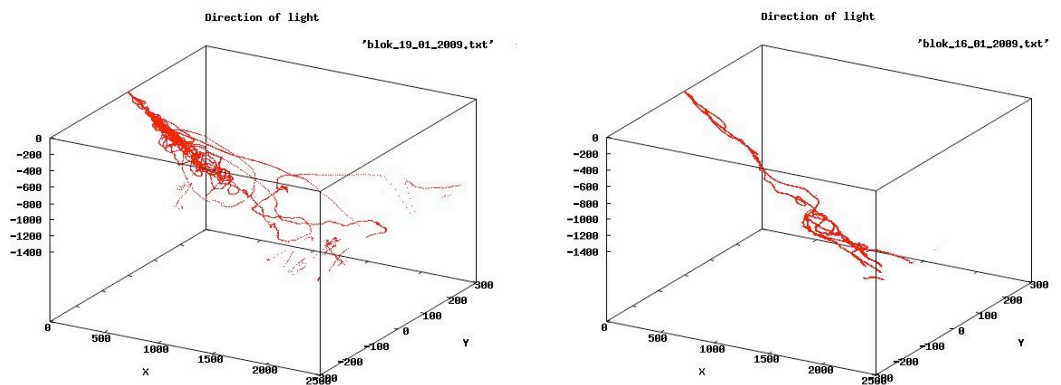
Figure 5. Direction of the daylight on January 19 th (sunny sky condition) and January 16 th (overcast sky condition)
