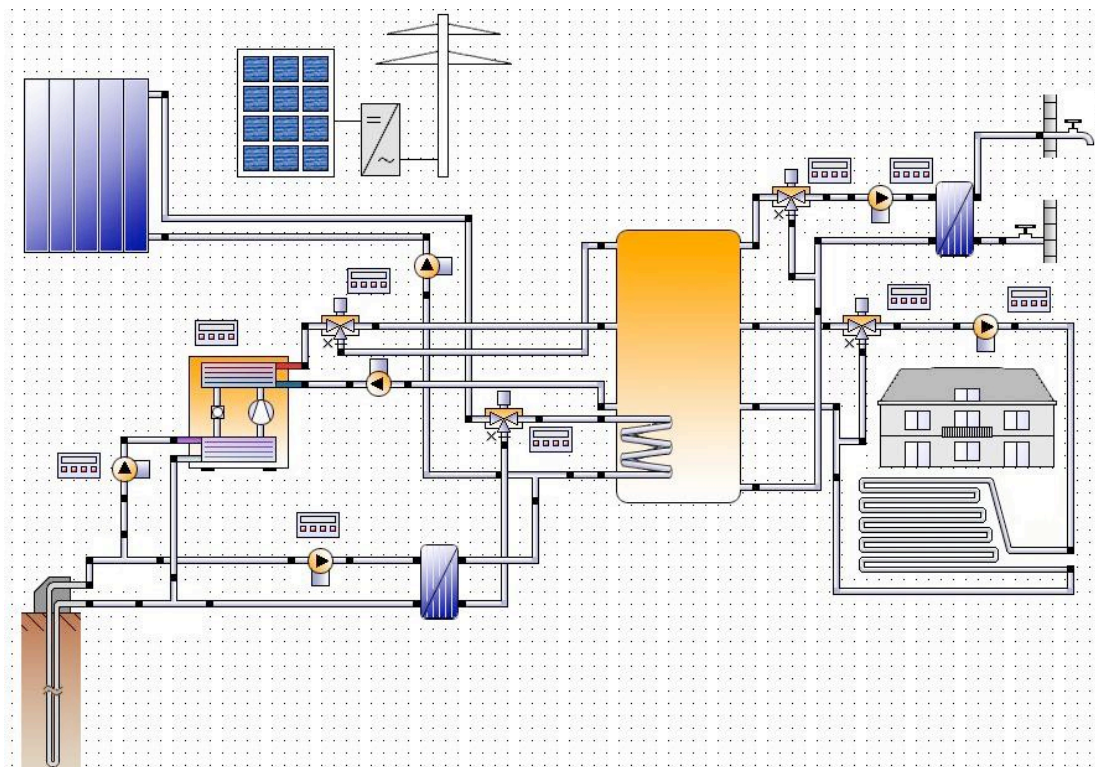
Figure 1: Polysun planning tool including solar thermal, geothermal/heatpump, and photovoltaics in one tool. Furthermore, all details of the heating system, such as radiators/floor heating, controllers and pumps are modeled with their physical behavior.
