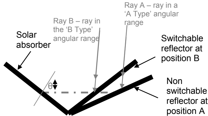
Figure 1: A single switchable reflector device
