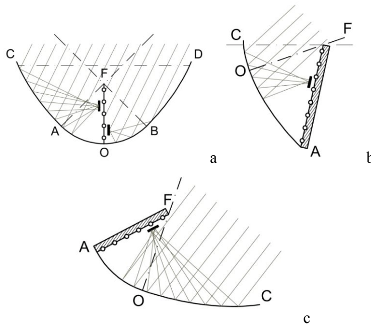
Fig. 4 The CPC reflector concept of symmetric type (a), with axis oriented to winter (b) and with axis oriented to summer (c) solstice
