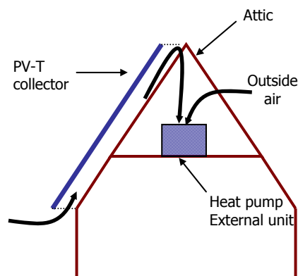
Figure 4-b –Heat pump in the attic (case2)
