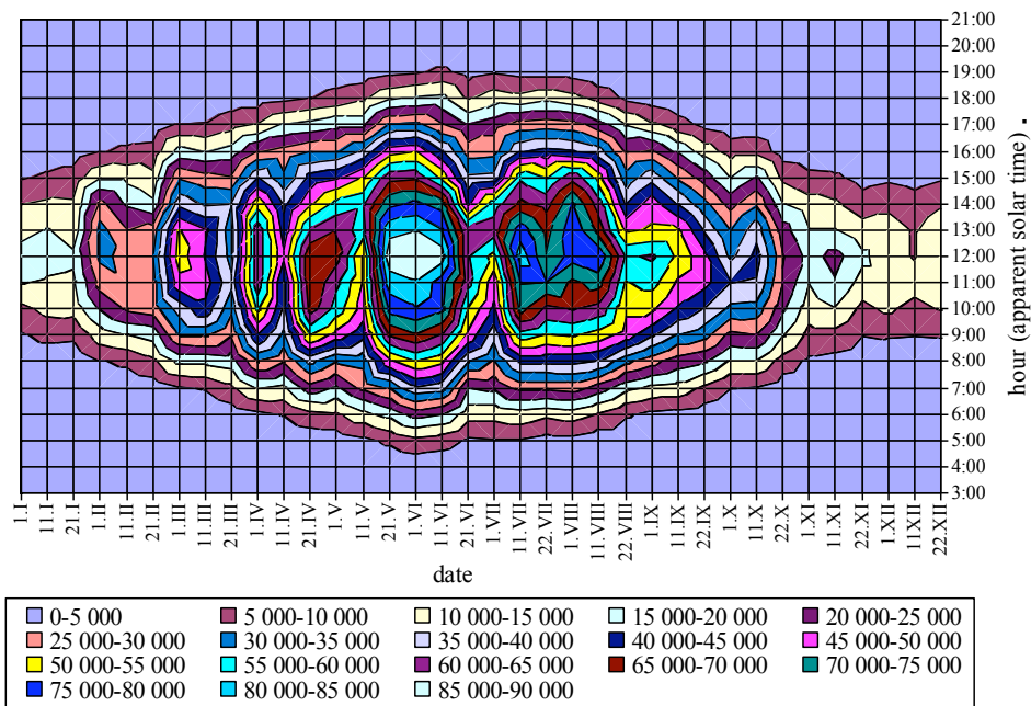
Figure 5: Global illuminance isolines for all year round in Bratislava
