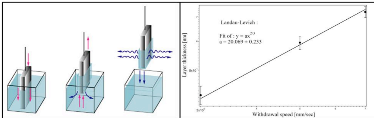
Figure 3: On the left: dip-coating process and the three main steps. On the right: measured thicknesses of the nanocomposite layer in a function of withdrawal speed. The data follow the exponential behaviour predicted by the Landau -Levich equation.
