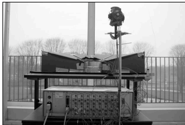
Figure 2. Measurement set-up including the Daylight Discomfort Detector, the cubic light direction detectors on the metal stand, the horizontal illuminance detector on the work plane (just right of the metal stand), the detectors near the daylight opening (partially visible on the right side of the set-up), and data acquisition equipment
