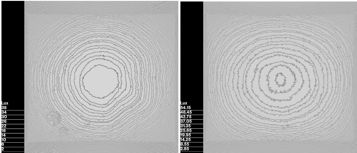
Figure 1: On the left the skylight and on the right the lightpipe isolux on February at 12 p.m..
