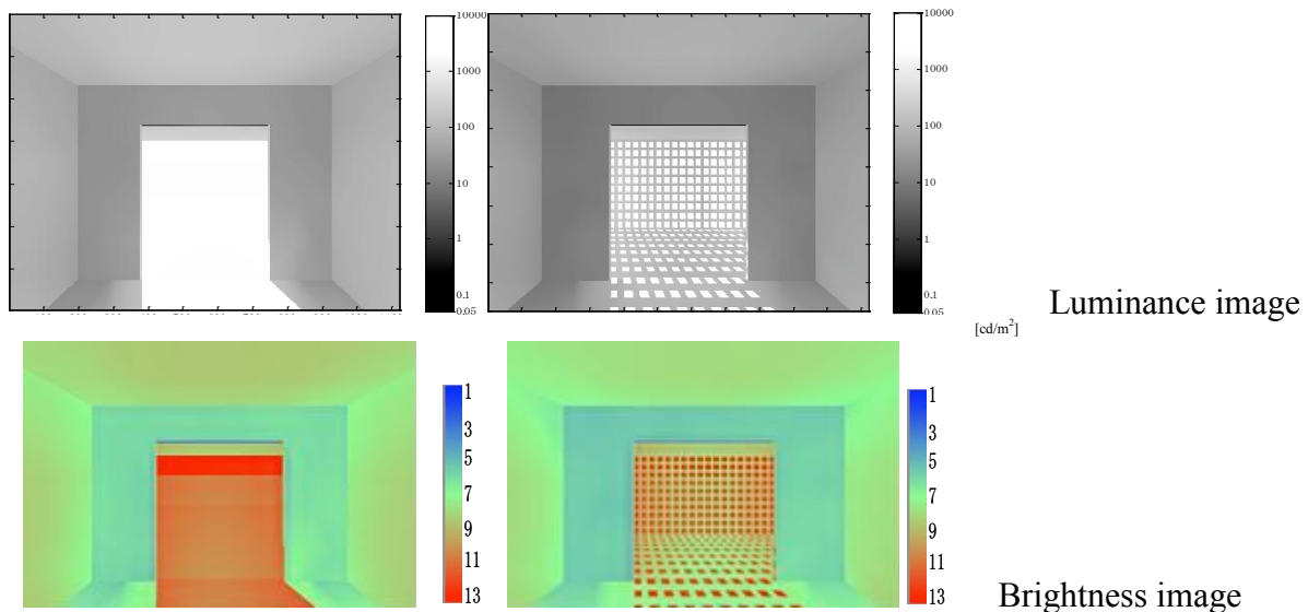
Figure 5: Comparisons between luminance images and brightness images with/without flower block (West opening, 3pm, March 21, Naha, Okinawa)
