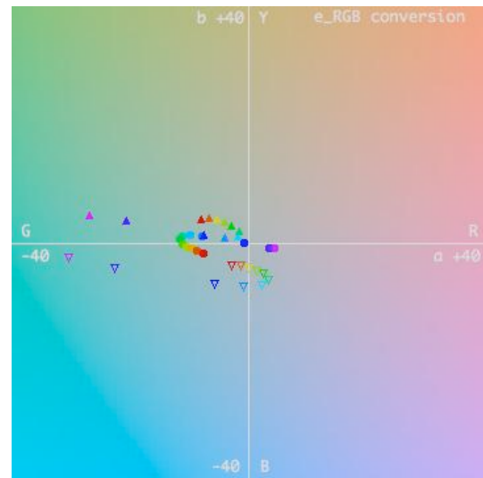
Figure 4: The colour evolution in the CIE Lab colour space at constant luminosity L of the transmittance (full circle, ●), reflectance glass side (full triangles, ▲), and reflectance layer side (empty triangles, ▽), if the angle of light incidence \phi is changed. For the smallest angle a purple symbol and for the largest a red symbol is used.
