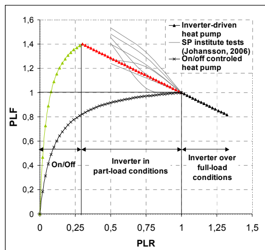
Figure 1-b PLF versus PLR
