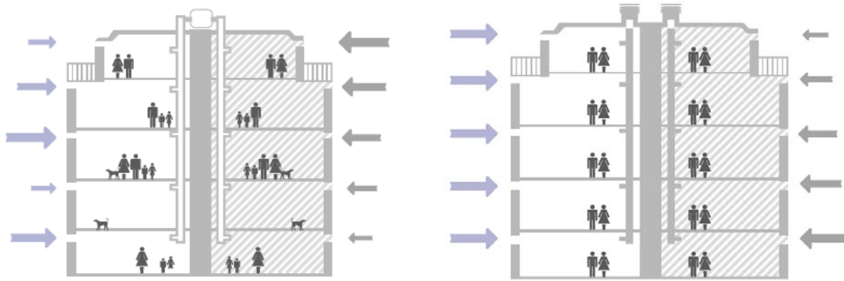
Figure 3: Dispatching of airflows between dwellings as a function of occupation and stack height. On the left, humidity sensitive ventilation, on the right standard extraction ventilation.
