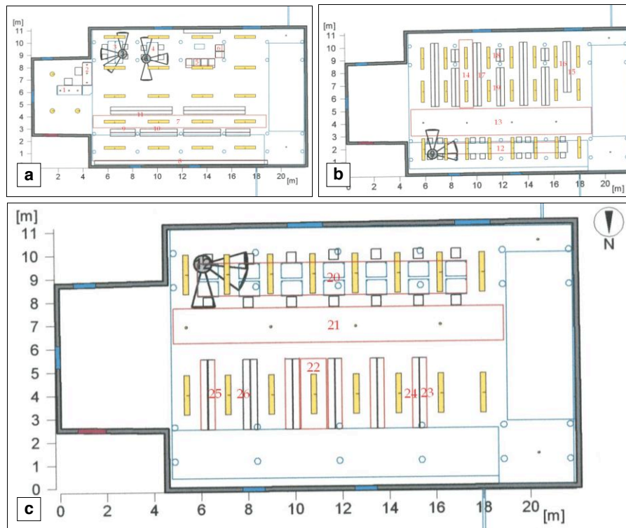
Figure 4 – Luminaires positioning: a) Ground floor; b) 1 st Floor; c) 2 nd Floor.
