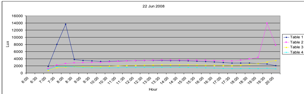
Fig. 11: Hourly illuminance values for a north facing opening on June 22 nd
