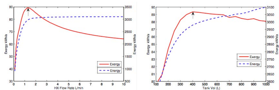
Figure 3: Plot of the exergy and energy recovery for different HX flow rates (left) and tank sizes (right). There is a clear optimum in the exergy analysis not given by the energy analysis.
