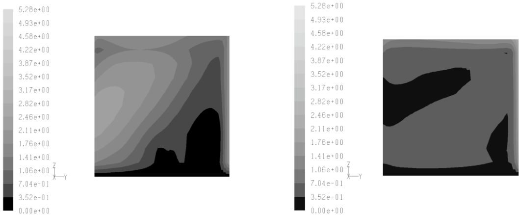
Figure 7. Contours of wind velocity in the vertical plane 0.5m from the east façade (case C, d=2.5\text{m} and d=10\text{m} , west wind direction).
