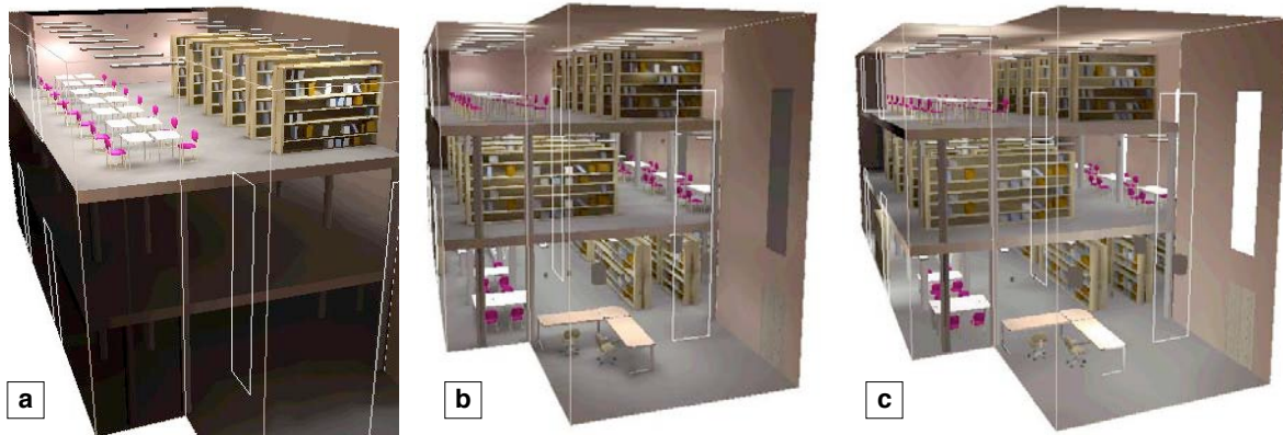
Figure 5 – 3D photorealistic images: a) 2 nd floor artificial lighting; b) artificial lighting; c) mixed lighting.
