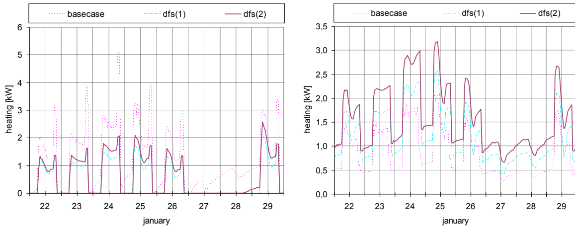
Figure 3: Power distribution for office (left) and hotel room (right).
