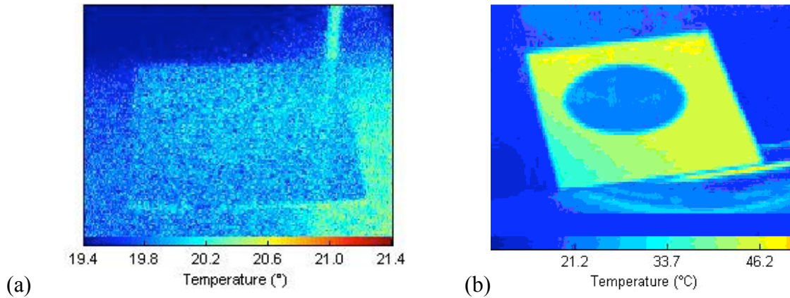
Figure 4: (a): At ambient temperature, VO_2:W is in the semiconducting state transparent for IR radiation. Therefore, the coating is not visible in the thermographic images. (b): In the metallic (hot) state, the film is clearly visible in the thermographic images. The entire system (substrate + film) emissivity is estimated to change from 85 % to 34 %. The saturation of the signal was avoided in all images.
