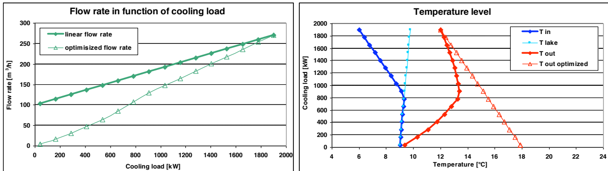
Figure 4. Chilled Loop flow rate (left) and operating temperatures (right)
