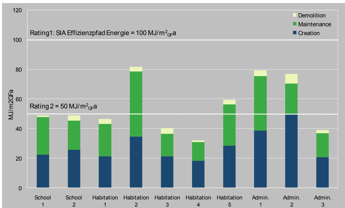
Figure 3: Analysis of new construction case studies: Comparison of embodied energy
