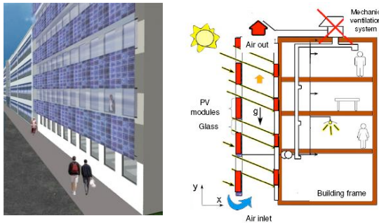
Figure 1: Schematic view of a double skin façade
