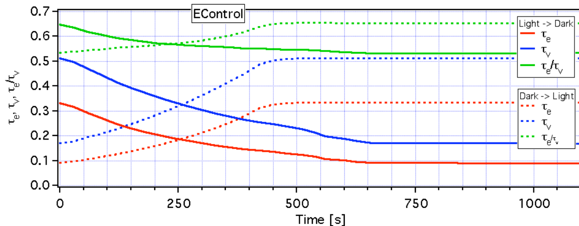
Figure 5: The evolution of the light transmittance \tau_v , the solar direct transmittance \tau_e , and the energy load coefficient \tau_e/\tau_v for the EControl glass, when switching from brightest (1) to darkest (5) transmittance.
