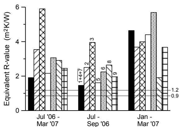
Figure 3: Equivalent R-values of test walls.
