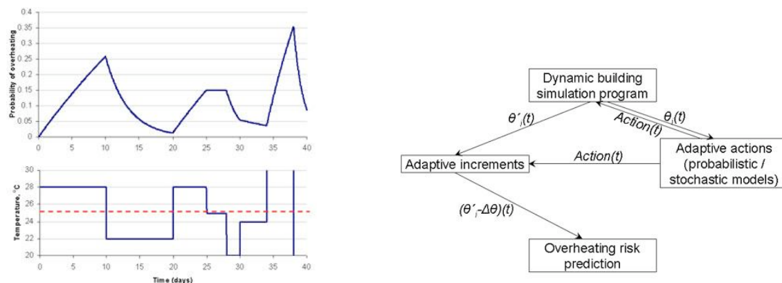
Figure 2: Step changes in indoor air temperature (bottom left) and a hypothetical overheating probability response curve (top left). Suggested model structure: integration of stochastic interaction and dynamic thermal comfort with building simulation models, the results post-processed by an overheating model
