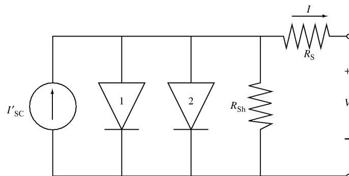
Figure 1: two diode model
