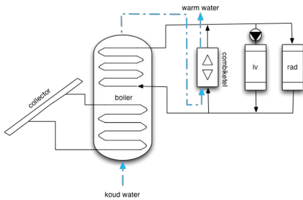
Figure 5: Solution II, combination with solar collector & boiler
