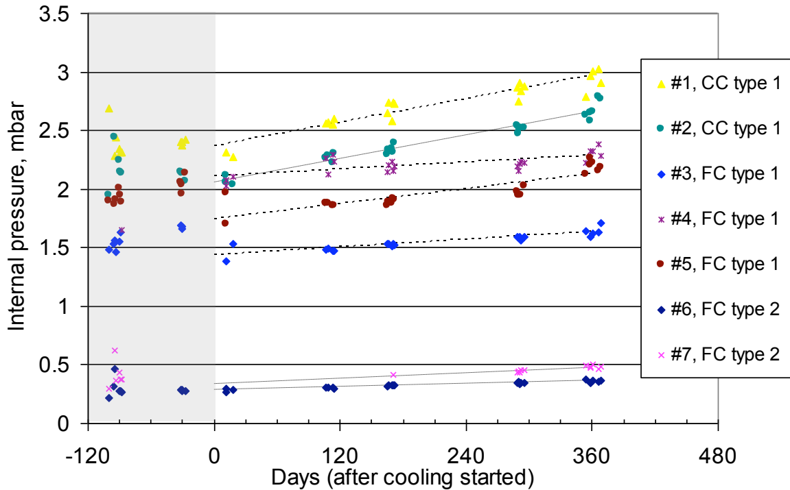
Figure 5: The pressure measured indirectly shows an increase of 0.6 mbar/year for the cooling room and about 0.2 mbar/year for the freezing room.
