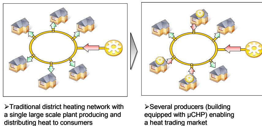
Figure 1. Distributed generation in a district heating network
