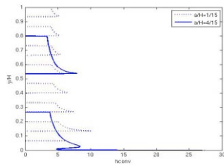
Figure 4: Heat transfer coefficients for case 1 and 4
