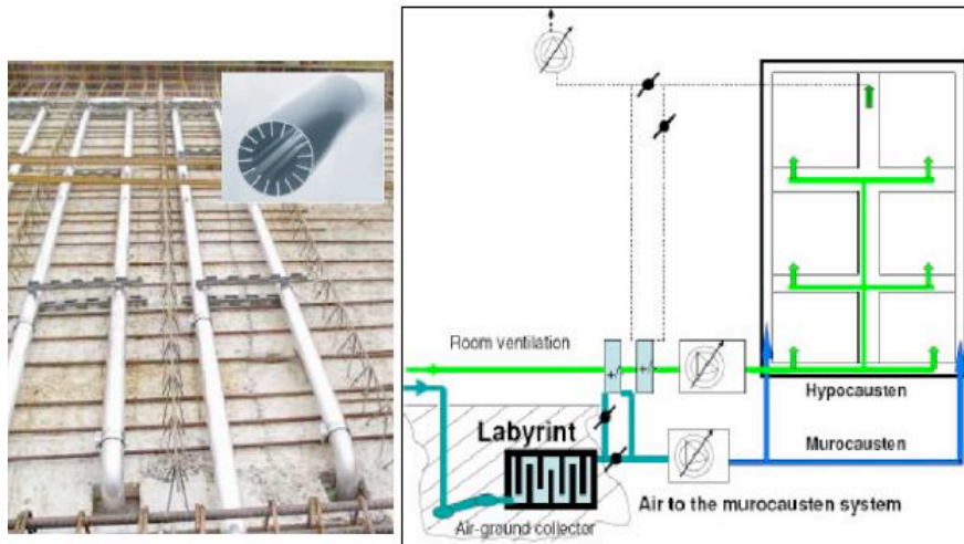
Figure 4: The concrete core activating system and schematic of the hypocausten /murocausten system in combination with air-ground collector and labyrinth foundation.
