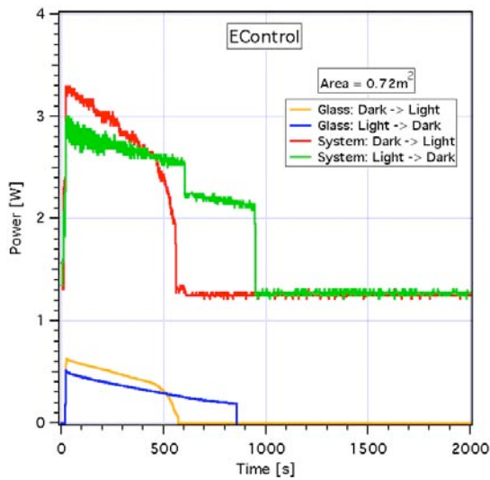
Figure 7: Power consumption of the EControl glass during the switching from the bright (1) state to the darkest (5) state or vice versa and afterwards keeping this status.
