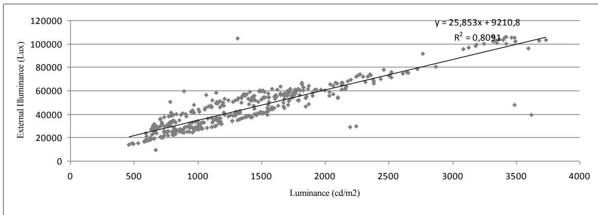
Figure 3: Diffuser luminance vs. external illuminance.
