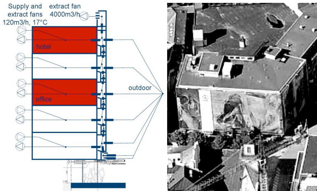
Figure 1: Model and airflow description and real building with textile facade.
