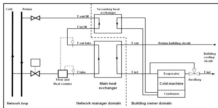
Figure 2: Connection between the cold network and a building, with a secondary heat exchanger
