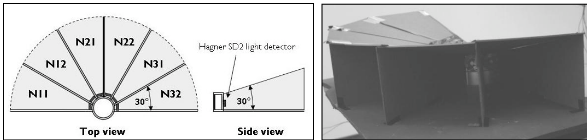
Figure 1. Daylight Discomfort Detector: schematic top and side view (left), and real-time model (right)
