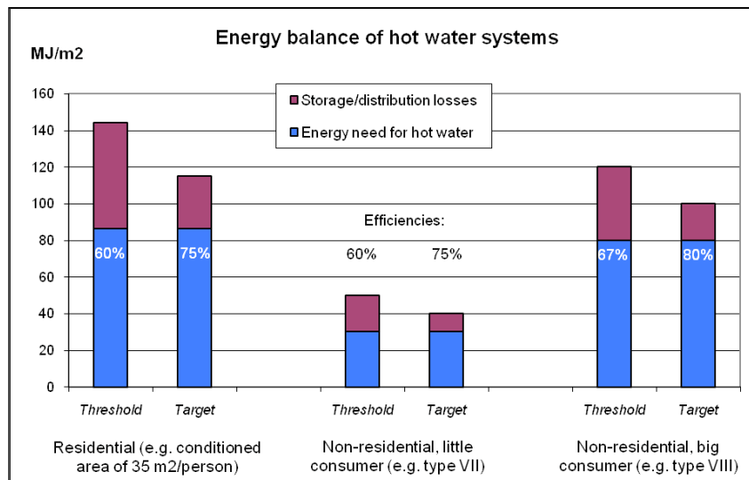
Figure 4: Suggested overall primary energy efficiency of hot water storage and distribution systems, for three building categories (residential, non-residential with low hot water consumption, other non-residential). Typical examples according to SIA standards. Left-hand bars: threshold values. Right-hand bars: target values.
