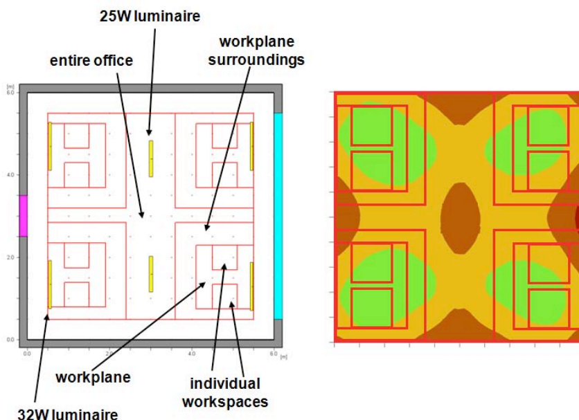
Figure 3: Luminaire positions and reference planes considered during computer simulations for the 36m 2 office room in Singapore (left) and resulting illuminance distribution at a reference height of 80 cm above floor level (right).
