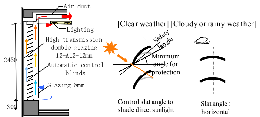
Figure 2: Cross-section of window.
