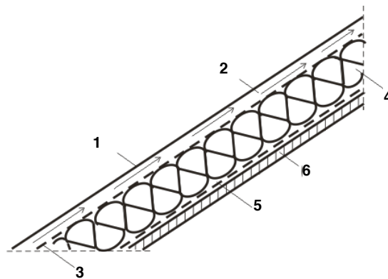
Figure 2: Roof covering structure: 1- air tight covering; 2- ventilated air layer; 3- thermoreflectant metallic sandwich sheet; 4- mineral wool; 5- vapour barrier; 6- support
