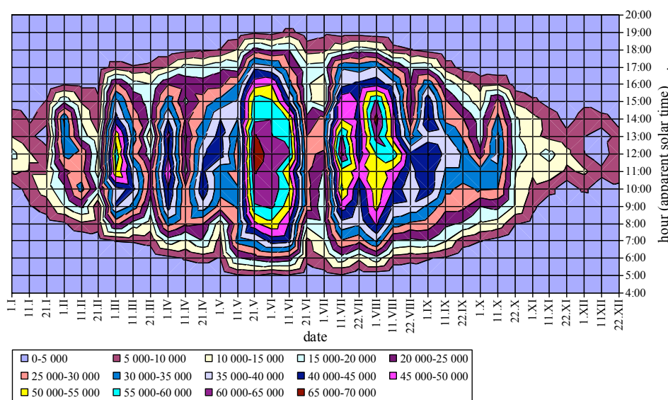
Figure 4: Direct illuminance isolines for all year round in Bratislava
