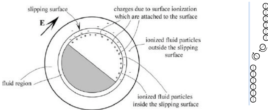
Figure 5: working principle of the Gyricon ball and the concept of a cluster of gyricon balls [2,6]
