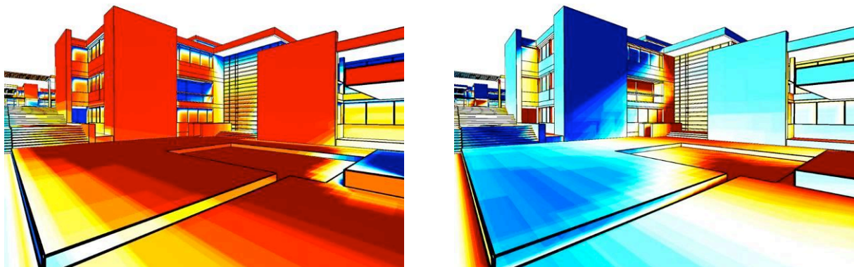
Figure 5: SOLARCHVISION summer analysis (left) and winter analysis (right)
