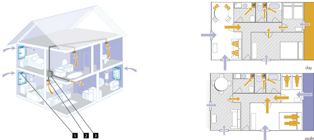
Figure 2: Airflows and humidity sensitive components in a single-family-house mechanical ventilation system. Typical day and nighttime dispatching of airflows within the dwelling.
