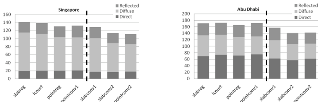
Figure 7: Solar irradiation on building façades per façade area ( W/m^2 ) for generic forms with different degrees of convolution (dash line: change in building depth)
