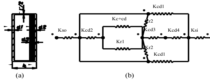
Figure 3: (a) Cross-section of one cell, d_3 denotes the thickness of aerogel insulation layer; (b) Simplified network. ( K_{cd} ) conductance of FRP or aerogel; ( K_{c+cd} ) effective conductance for conduction and convection of the air in the cavity; ( K_r ) effective conductance for radiation among the four enclosed FRP surfaces; ( K_s ) surface conductance.
