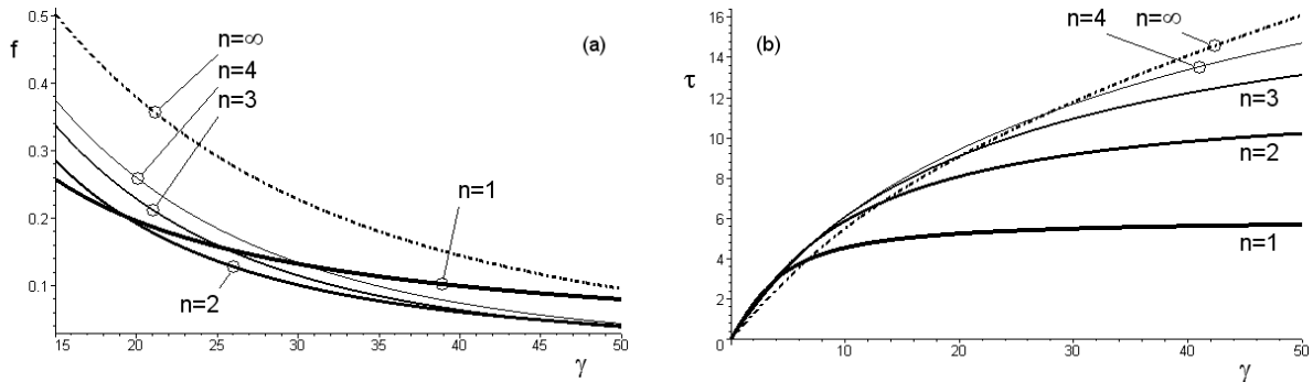
Figure 2 – Trends of the decrement factor f (Fig. 2a) and of the time lag \tau (Fig. 2b) with \gamma for various stratigraphies corresponding to n=1, 2, 3, 4 ; n=\infty refers to the homogeneous wall.
