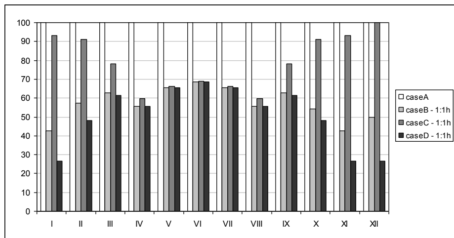
Figure 2. Comparison of solar direct radiation for analysed cases.
