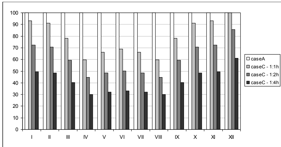
Figure 4. Comparison of solar direct radiation for different building height in case C.
