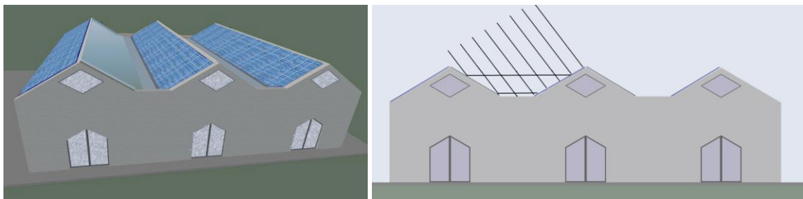
Fig. 2 Building integrated PV or PVT collectors combined with booster reflectors
