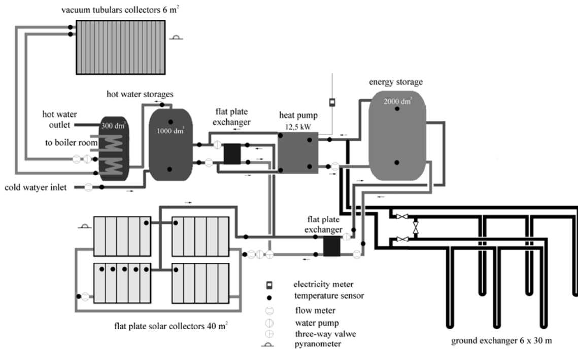
Fig. 1. The hybrid system flow chart
