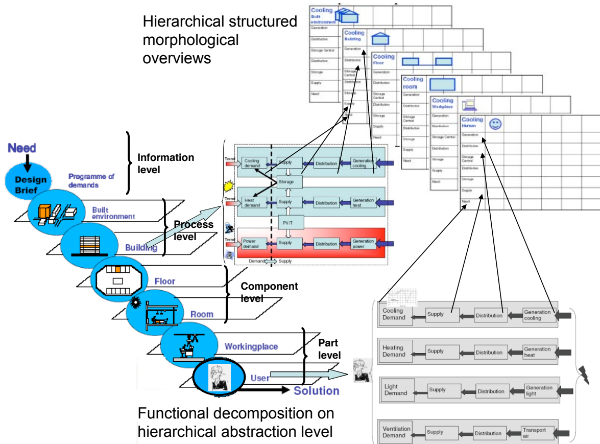
Figure 3: Set of connected morphological overviews about cooling on the different hierarchical abstraction and the infill on the built environment level
