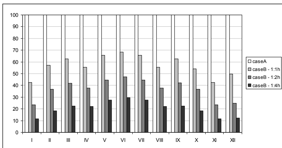
Figure 3. Comparison of solar direct radiation for different building height in case B.
