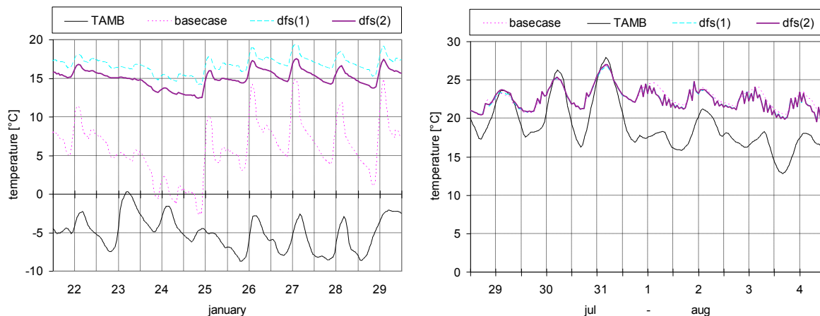
Figure 2: Temperature distribution in hotel room (5 th floor) winter (left) and summer (right).
