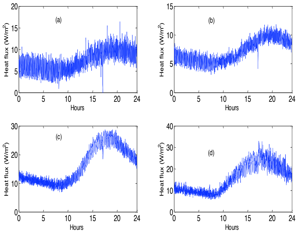
Figure 4: Eastern and western walls heat fluxes, (a), (b) for insulated room, (c), (d) for non insulated room
