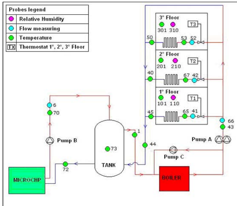
Figure 1: Experimental heating plant scheme
