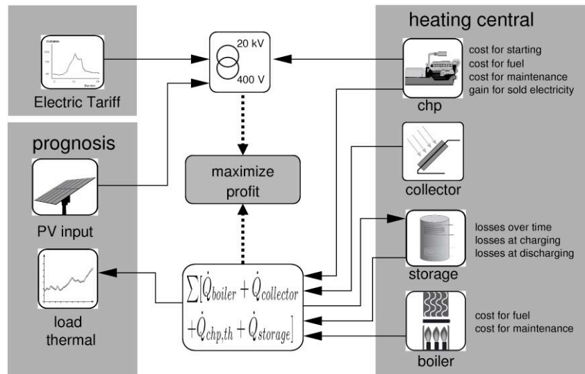
Figure 1: The components of a local energy management are shown. The components interact by power flows
