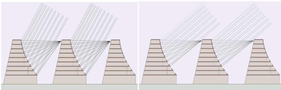
Fig. 7 Building integration of movable reflectors with stationary PV or PVT absorber
