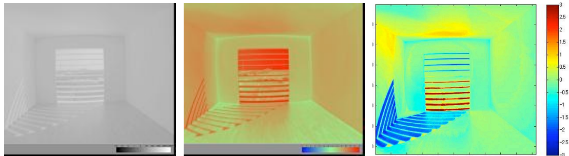
Figure 3: Examples of luminance image (left), Brightness image (centre) and Image by differences of brightness images with/without devices (right)
