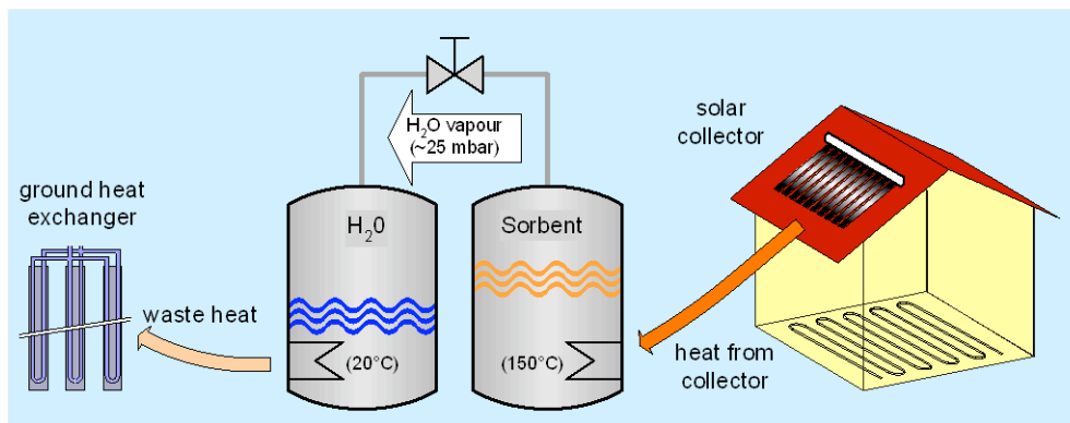
Figure 1: Charging mode. Sorbent is heated up to evaporate the working fluid.
