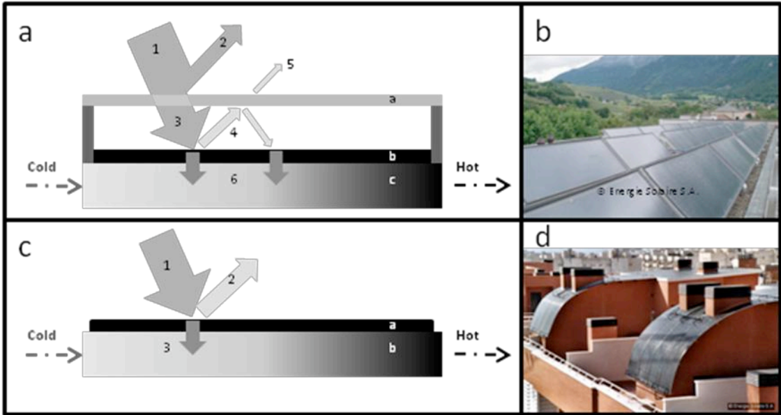
Figure 1: a) schematic diagram of radiative energy transfer in a glazed solar panel b) picture of glazed solar panels installed on the roof of a building c) schematic diagram of radiative energy transfer in an unglazed solar panel d) picture of unglazed solar roof.
