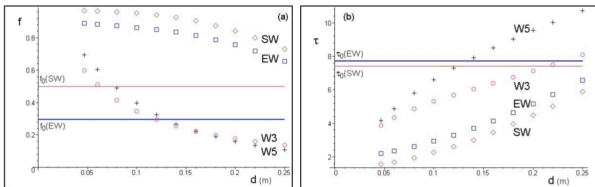
Figure 3 – M=M_{lim}/4 , the trend of the decrement factor f (Fig. 3a) and of the time lag \tau (Fig. 3b) with the insulating thickness d (m), for the four considered walls.
