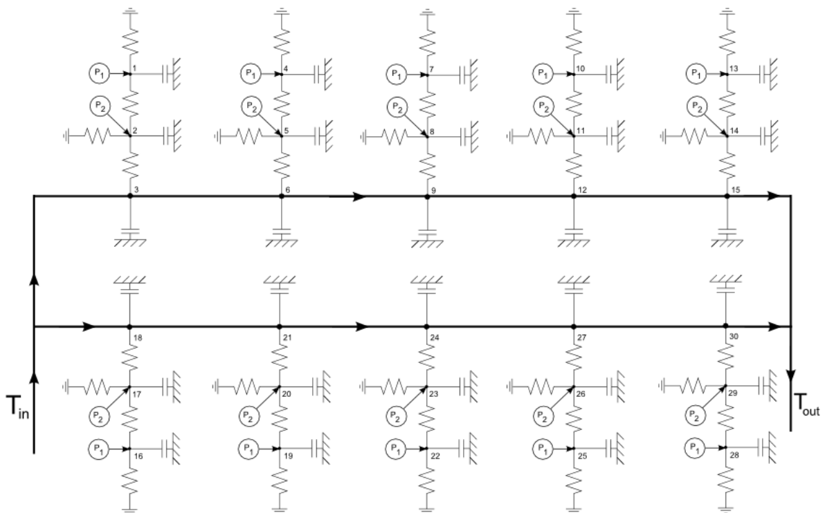
Fig.3. The battery of flat plate collectors in the hybrid system presented as Equivalent Thermal Network.
