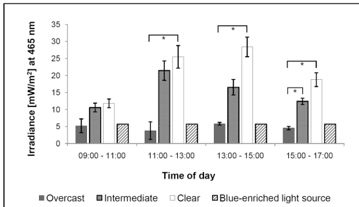
Figure 3: Daylight irradiances ( mW/m^2 ) at 465nm for three sky types between 09:00 and 17:00. * = p<0.05 ; \pm SE, expressed in 2h bins. The irradiance of the artificial blue-enriched light source at 465nm (during night time) is also shown.
