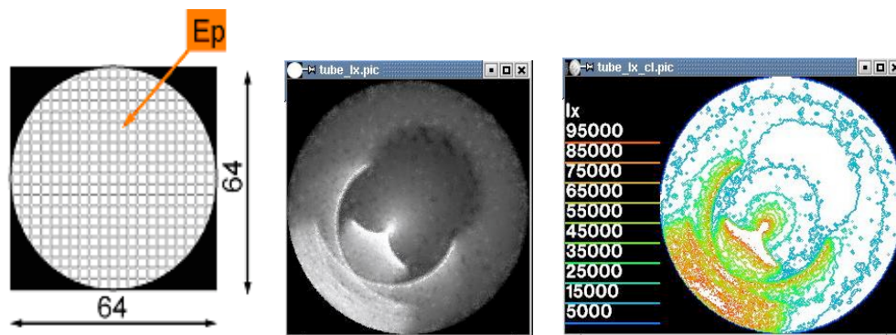
Figure 1: Parallel view of the upper part of the diffuser – scheme of generated picture ( 64 \times 64 pixels) (left), rendered picture (middle) and illuminance isolines (right)
