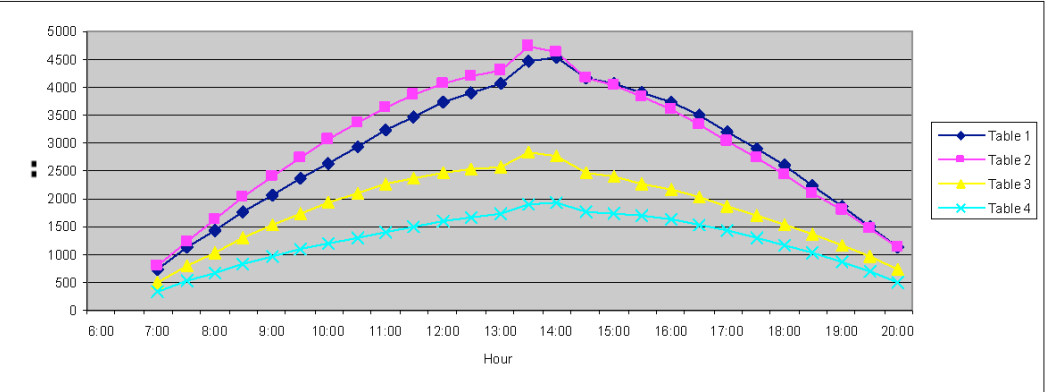
Fig. 6: Hourly illuminance values for 22 nd of June
