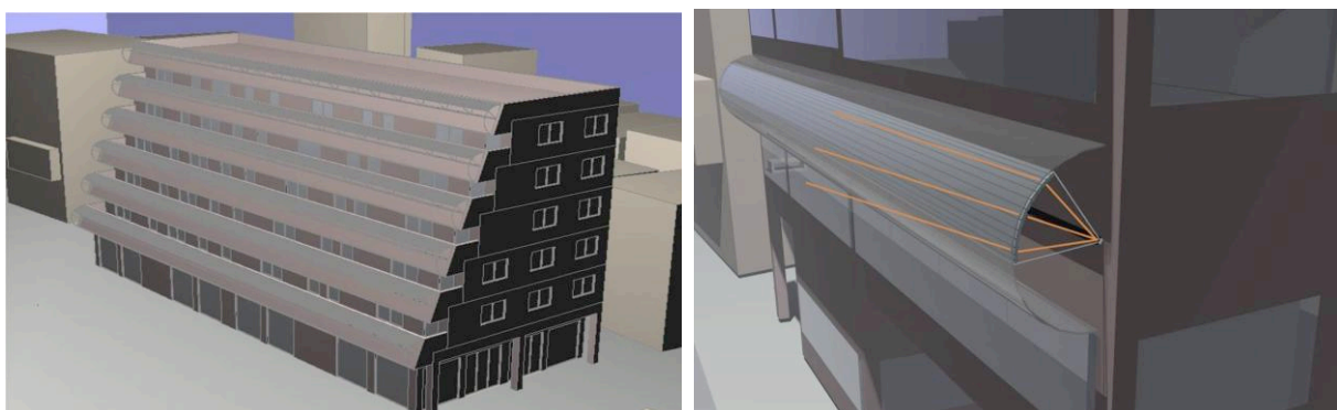
Fig. 8 Building integration of rotating curved Fresnel lenses and stationary PV or PVT absorber
