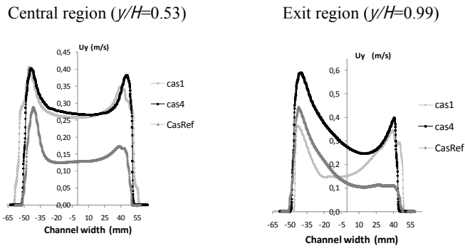
Figure 3: Mean vertical velocity profiles in two regions
