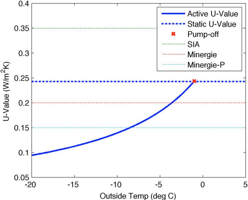
Figure 3: B35 active insulation performance
