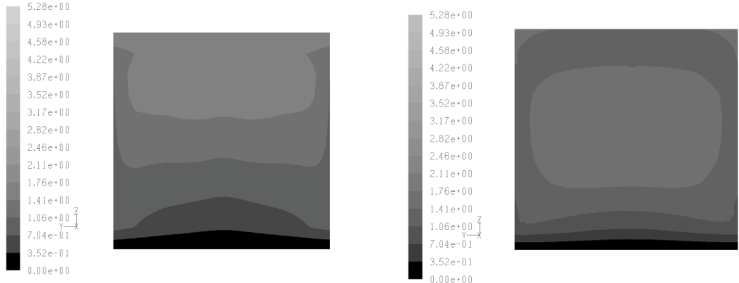
Figure 6. Contours of wind velocity in the vertical plane 0.5m from the east façade (case B, d=2.5\text{m} and case D, d=10\text{m} , east wind direction).
