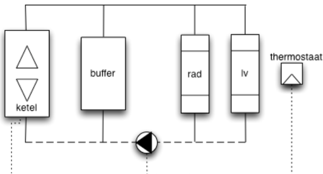
Figure 4: Solution addition of buffer vessel.
