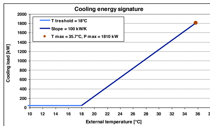
Figure 3: Model of the cooling energy demand of a building based on measurements (data by hour)
