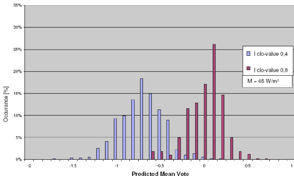
Figure 2: Calculated PMV based on the measurements for the actual I_{clo} of 0,4 and the recalculated PMV for the I_{clo} of 0,8 from the Dutch standard design brief specifications [13]
