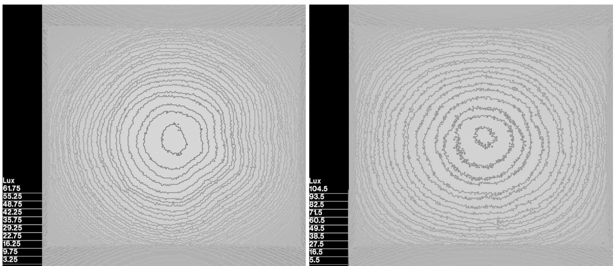
Figure 3: On the left the skylight and on the right the lightpipe isolux on August at 12 p.m..
