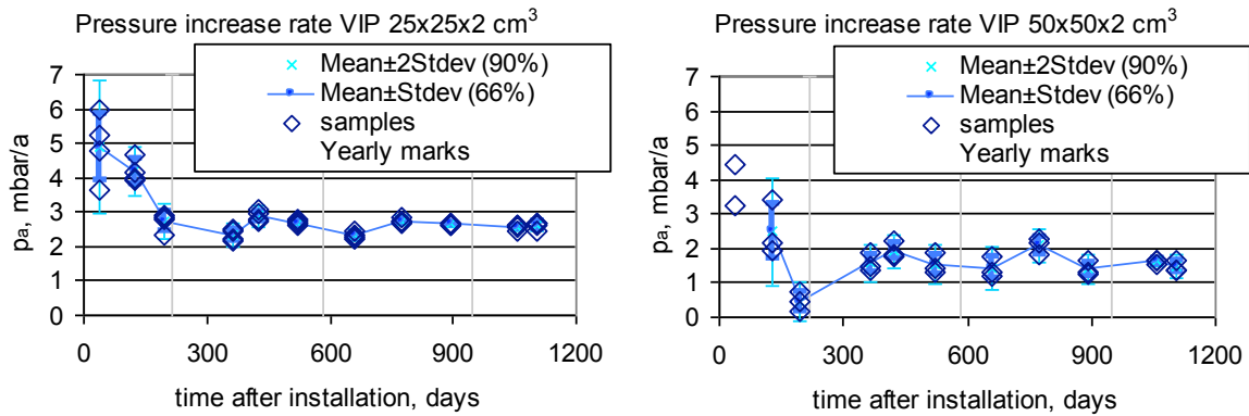
Figure 3: Yearly pressure increase rates as determined for the two VIP sizes on a terrace roof. More than a year is recommended for such kind of measurements as seasonal influences are visible and have to be considered.
