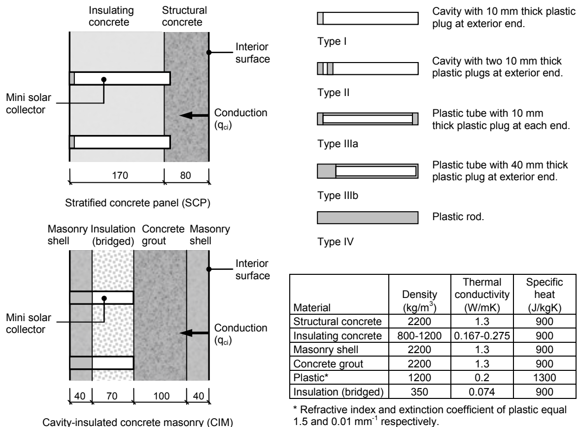
Figure 1: Types of model walls and collectors.
