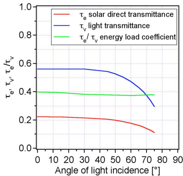
Figure 3: The evolution of the light transmittance \tau_v(\phi) (blue), the solar direct transmittance \tau_e(\phi) (red), and the energy load coefficient \tau_e(\phi)/\tau_v(\phi) (green) for different angles of incidence \phi .
