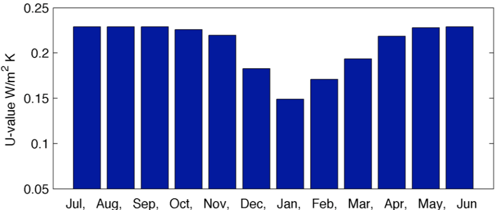
Figure 4: Monthly average U-Value for the active insulation system
