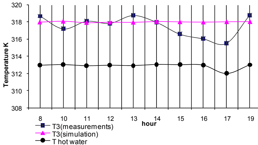
Fig. 4. The comparison graph for simulation and measurements in an exemplary daytime.
