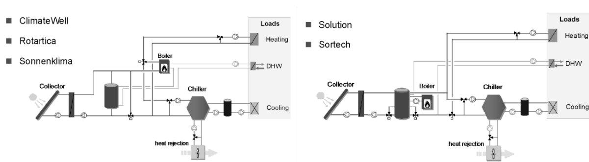
Figure 2 – Solar combi+ layouts selected by the industrial partners.
