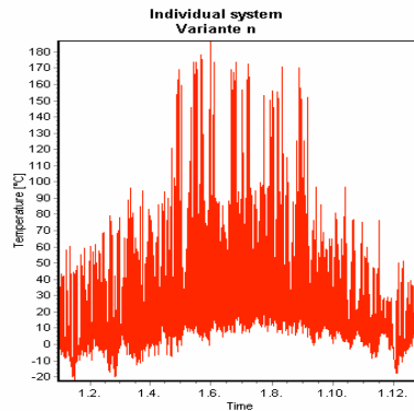
Figure 4: Temperature of glycol in the centre of solar collector (absorber area: 7,4 m 2 ) [10].
