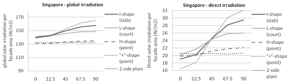
Figure 6: Solar irradiation on building façades per façade area ( W/m^2 ) vs. orientation of principal façade (degrees from south)
