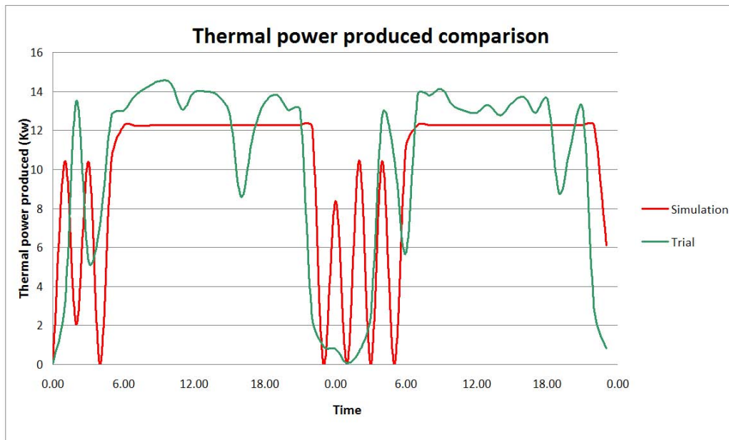
Figure 4: Comparison between thermal productions
