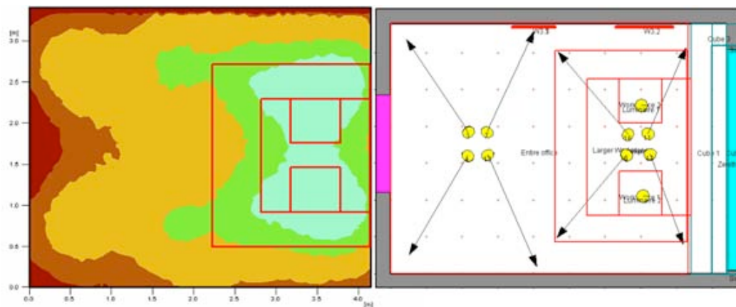
Figure 4: Resulting illuminance distribution for the LED-based lighting design at a reference height of 80 cm above floor level (left) and positioning of the LED luminaires on the office room's ceiling (right).
