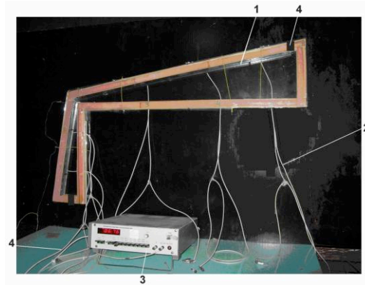
Figure 3: Physical model for a half attic: 1-heating wire; 2-thermocouples; 3-microvoltmeter; 4- air admission; 5- air exit Physical model for a half attic: 1-heating wire; 2-thermocouples; 3-microvoltmeter; 4- air admission; 5- air exit
