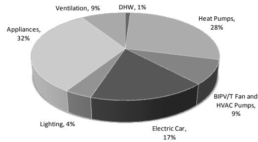
Figure 1: State of construction of Alstonvale Net-Zero House (May 18 th , 2009) and breakdown of the ANZH electrical energy consumption (9.000-9.200 kWh).
