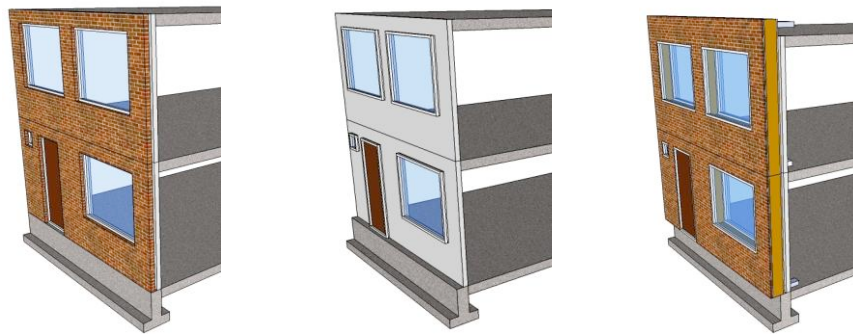
Figure 3: Visualization of the renovation process; the existing structure (left), the stripped structure without the outside layer of the brick cavity wall (middle) and the new facade structure with the +Facade component including the existing windows and new piping for ventilation.
