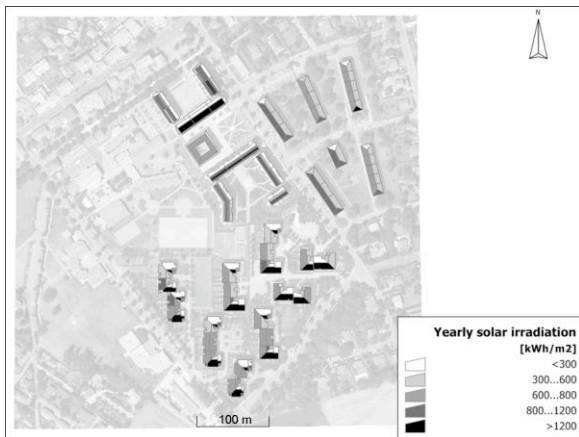
Figure 5: Annual solar irradiance values for the first pilot zone
