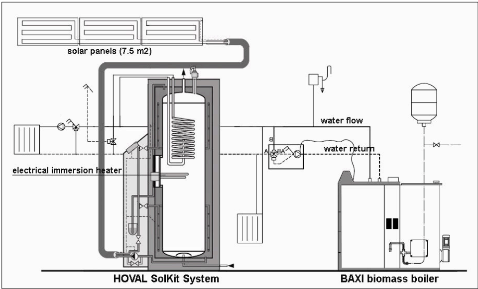
Figure 2 Schematic of Water and Space Heating System installed in the BASF House [5].
