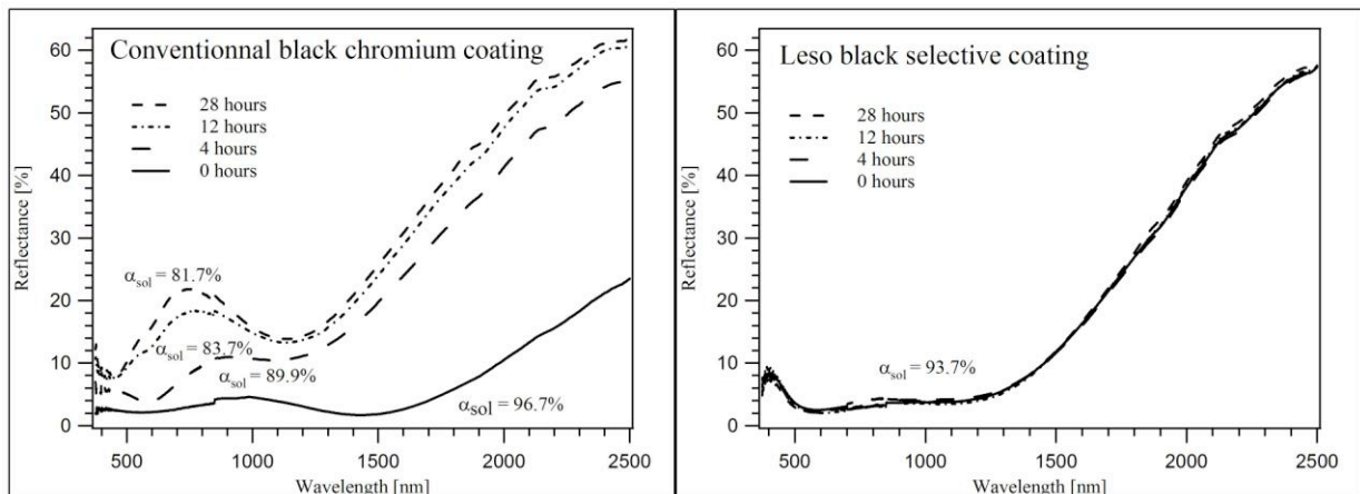
Figure 5: Aging test at 360^\circ\text{C} during 28 hours. On the left, the graph represents the evolution of the reflectance of black chrome coating after 0 hours, 4 hours, 12 hours and 28 hours. On the right, the same evolution for the novel nanocomposite solar absorbing coating is represented.
