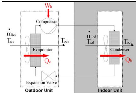
Figure 1-a Heat pump energy balance
