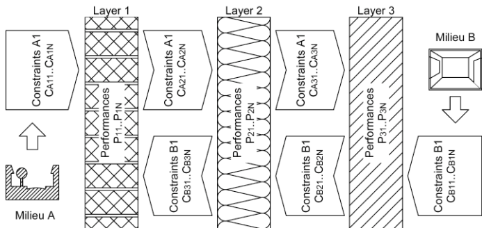
Figure 2: Constraints affect the element from both sides
