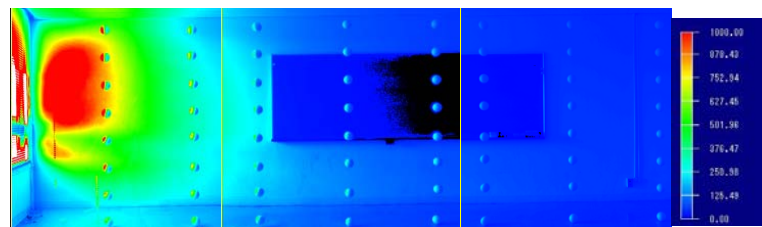
Figure 10: Spatial distribution of radiance of white globe.
