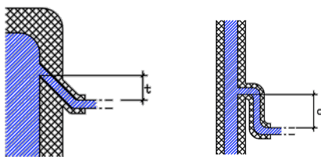
Figure 3: Two examples of heat traps to be installed between a hot water store (left) or a warm distribution line (right) and an end-use distribution line that has to cool down after draw-off. Minimum vertical heat trap extension: t > 7 cm (left), q > 12 cm (right) [6].
