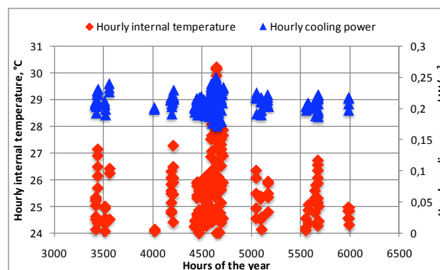
Figure 3: Hourly internal temperature of building and hourly cooling power for whole cooling season (internal temperature of building is equal or increase 24 °C).
