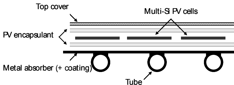
Figure 2: Lamination of PV components on metal absorber.
