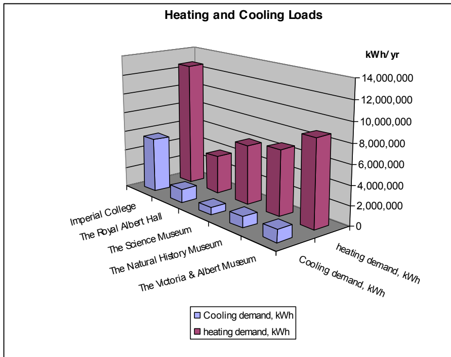
Figure 3: The load profiles show a predominance of heating loads.
