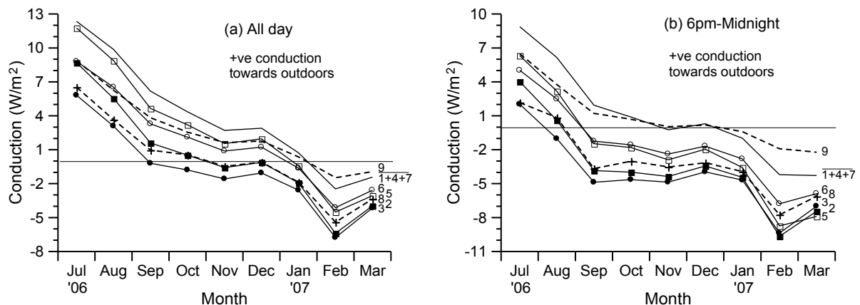
Figure 6: Monthly mean conduction at the interior surfaces of test walls.
