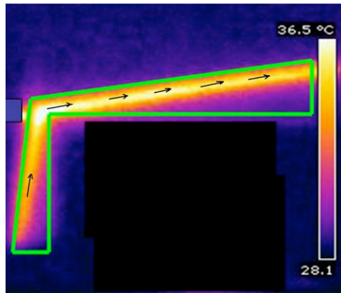
Figure 6: Air flow image with an infrared camera
