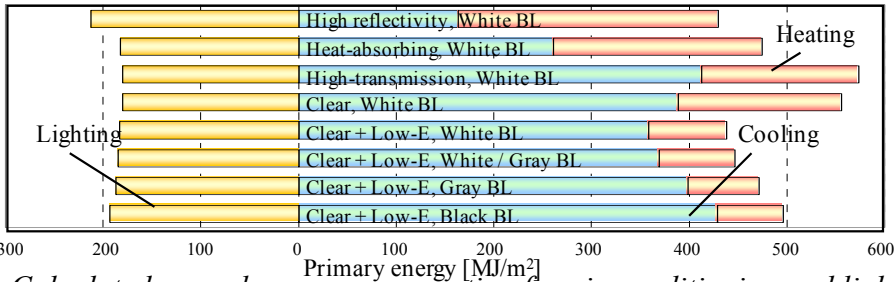
Figure 17: Calculated annual energy consumption for air-conditioning and lighting.
