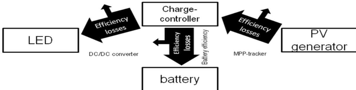
Figure 1: energy balance in an LED/PV system
