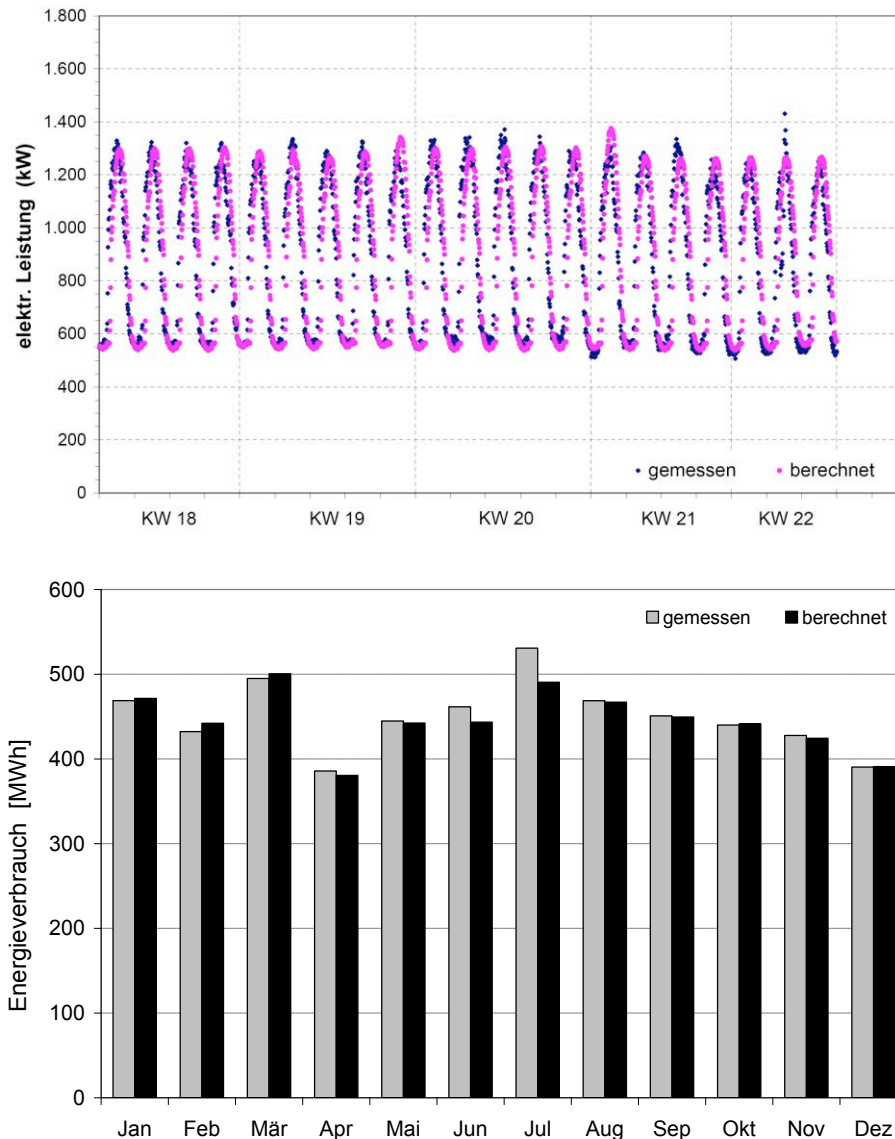
Figure 4: Comparison of measurement data and load prediction (above: hourly power values, below: monthly consumption)
