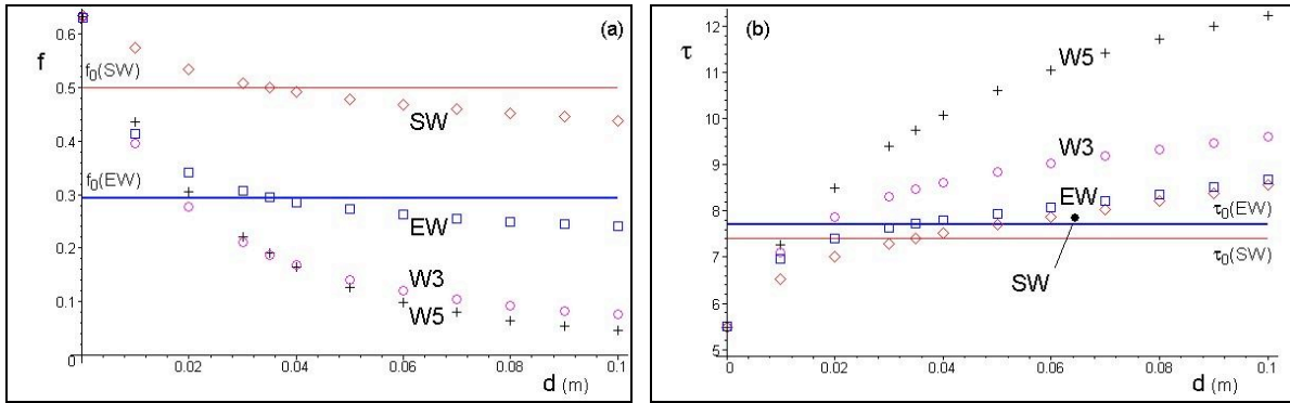
Figure 1 – M=M_{lim} , the trend of the decrement factor f (Fig. 1a) and of the time lag \tau (Fig. 1b) with the insulating thickness d (m), for the four considered walls.
