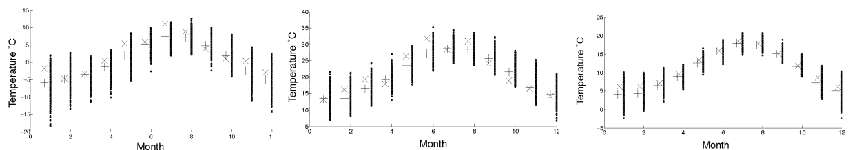
Figure 1: Variation in 1,500 control weather files - minimum (a), maximum (b), and mean (c) monthly temperatures
