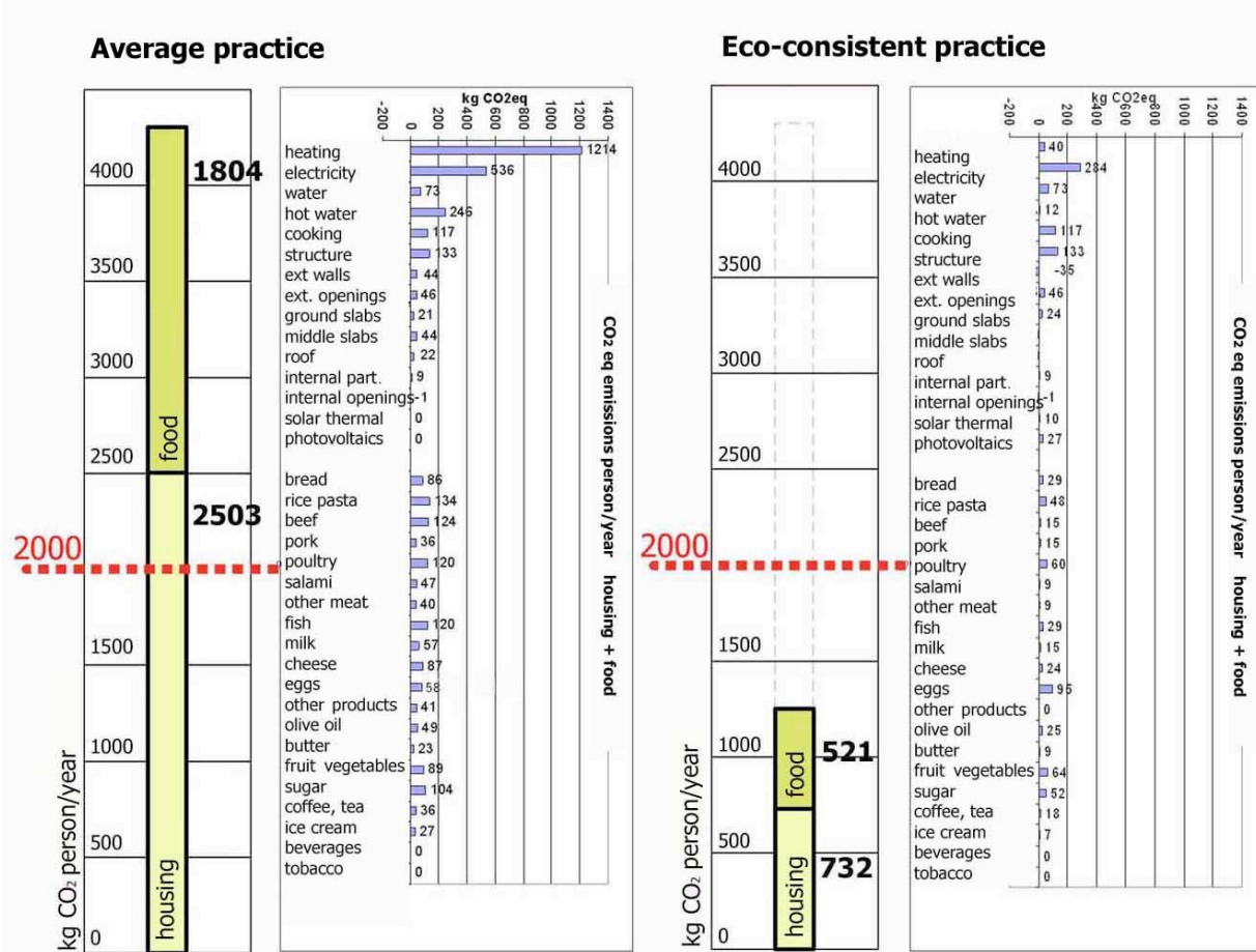
Figure 2: CO 2 eq. emissions/person-year related to housing and food. The dashed line defines the sustainable limit to the annual emissions per capita. The histograms on the left refer to the average practice, the building as it is, those on the right refers to the more eco-consistent one, the upgraded building..
