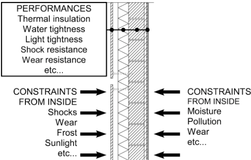
Figure 1: Multi-layer Facade Element - Constraints affecting the element performances
