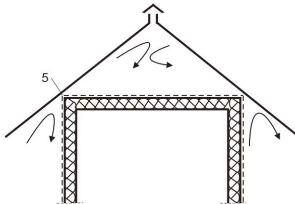
Figure 4: Air flow pattern when the air layer is strangulated in point 5
