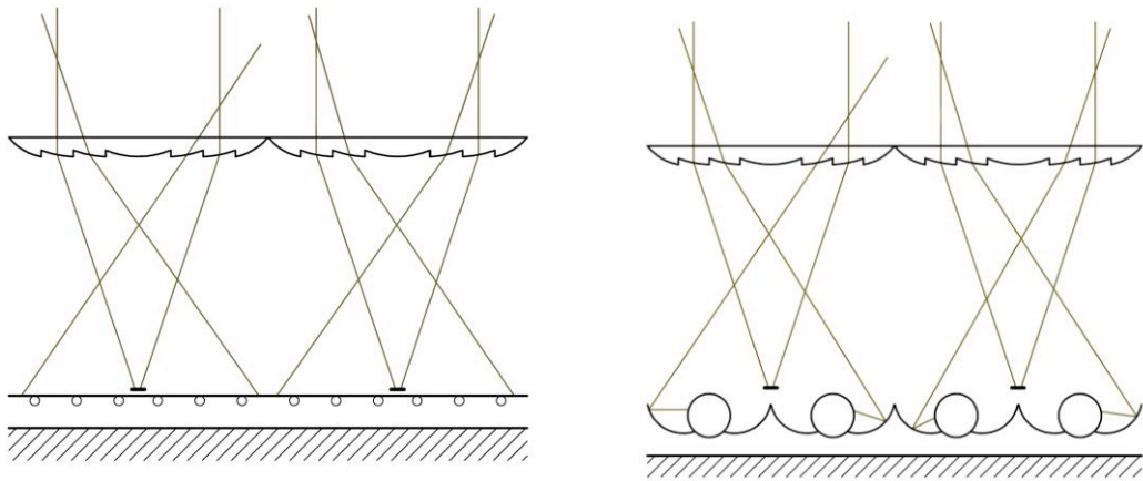
Fig. 3 Fresnel lens/PV strip with flat (left) and tubular (right) thermal absorber
