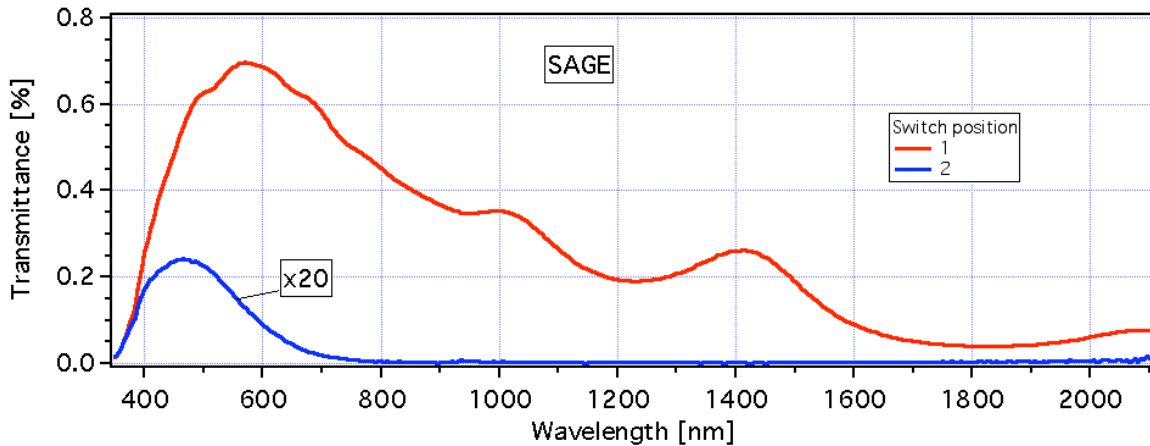
Figure 2: The spectral transmittance of the SAGE glass for the two different switch positions, where 1 corresponds to the uncoloured and 2 to the dark coloured state. The transmittance of the dark state is magnified with a factor of 20.
