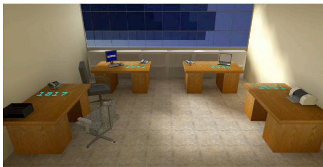
Fig. 10: Sunlight penetration utilizing WALLDOW in the simulated room on November 22 nd , at 11:00 AM
