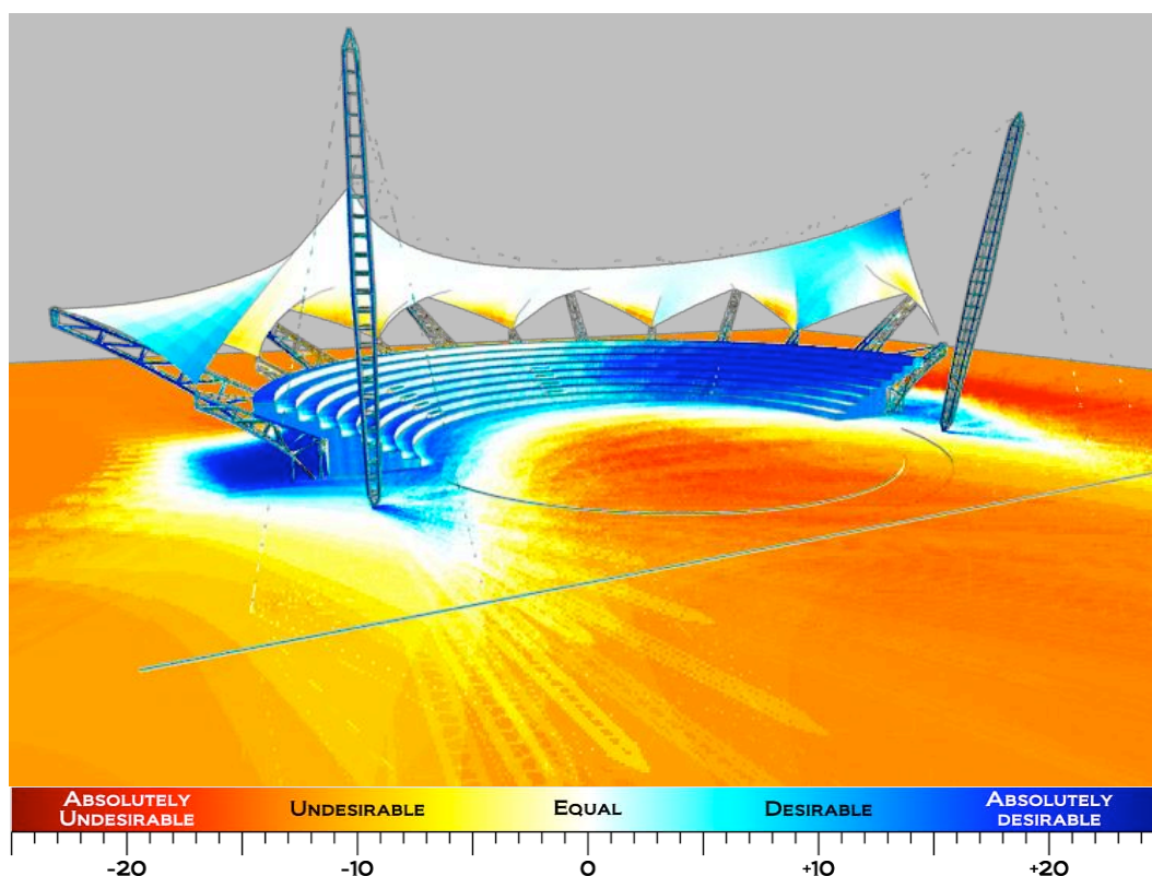
Figure 1: SOLARCHVISION yearly solar analysis diagram in the climate of Tehran.
