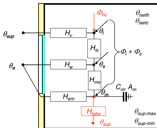
Figure 1: Schematic of the room model from EN ISO 13790 with modification
