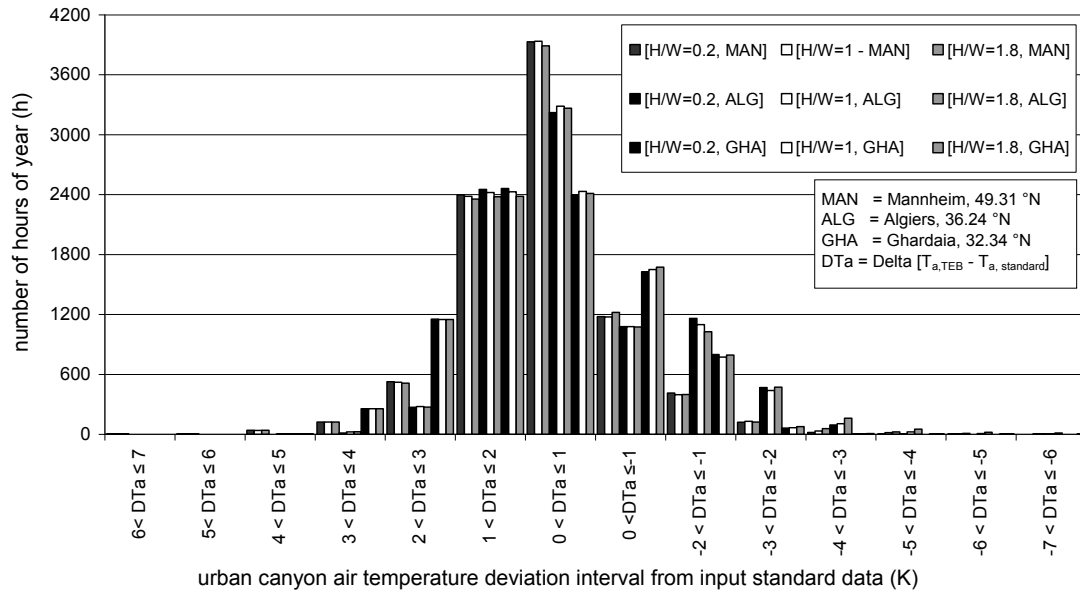
Figure 2: Example of TEB-simulated urban canyon air temperatures deviation from standard climatic data for various vertical profiles and for 3 climate locations. Here, the building is massive with a window ratio of 30% and a high thermal insulation ( U_{wall} = 0.15 ).
