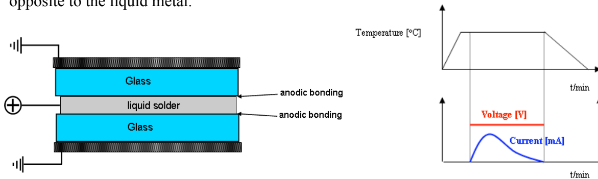
Figure 1a: anodic bonding setup schematic Figure 1b: Temp., voltage & current profile
