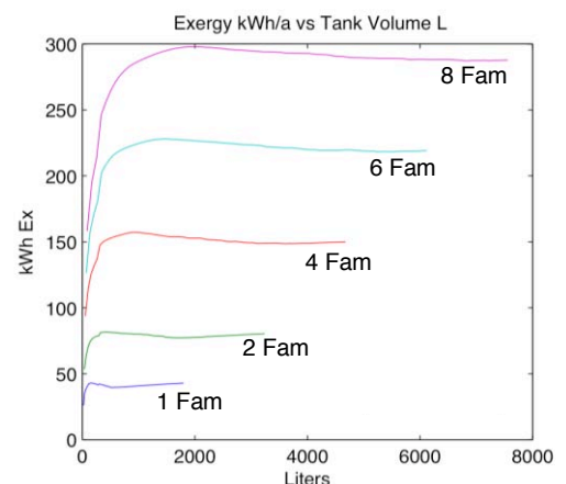
Figure 4: Tank Size exergy recovery optimization for different sizes
