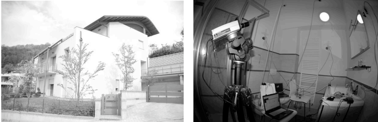
Figure 1: "Leaf House" of LOCCIONI Company and internal measurement set-up
