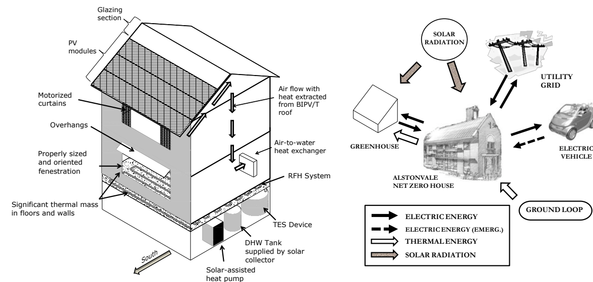
Figure 2. Conceptual representation of the ANZH energy system (solar thermal collectors not shown), and energy exchange possibilities between the house, the greenhouse and the EDV.
