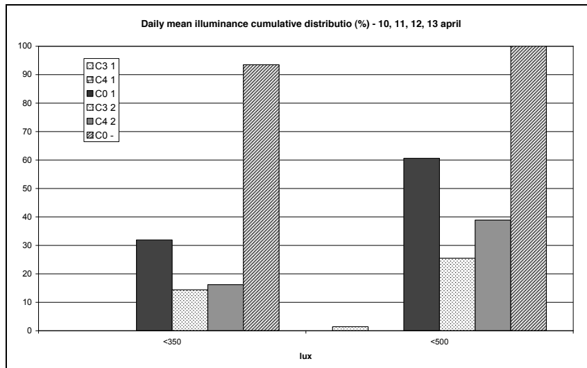
Figure 6: Illuminance cumulative distribution for C0 with blind, C3, C4.
