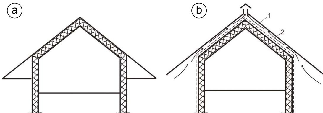
Figure 1: Building attic: a- traditional structure; b- ventilated air layer (1), and thermoreflectant thin metallic sheet (2)
