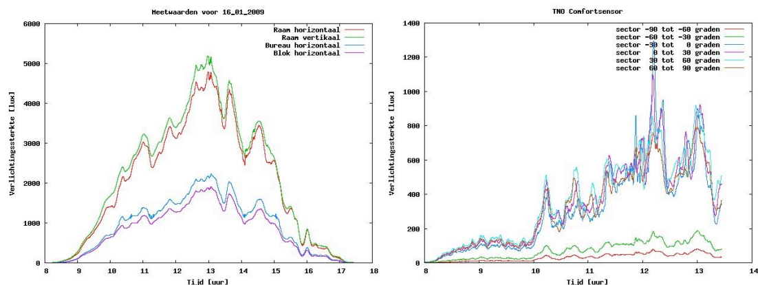
Figure 4. Daylight measurements on an overcast day (January 16 th , 2009), with illuminances on the glass and horizontal work plane (left), and illuminances as measured by the DDD in six viewing directions (right). The levels are much lower with variations due to layers of clouds and variable thickness of clouds, compared to levels on a sunny day. The DDD shows no extreme peaks.
