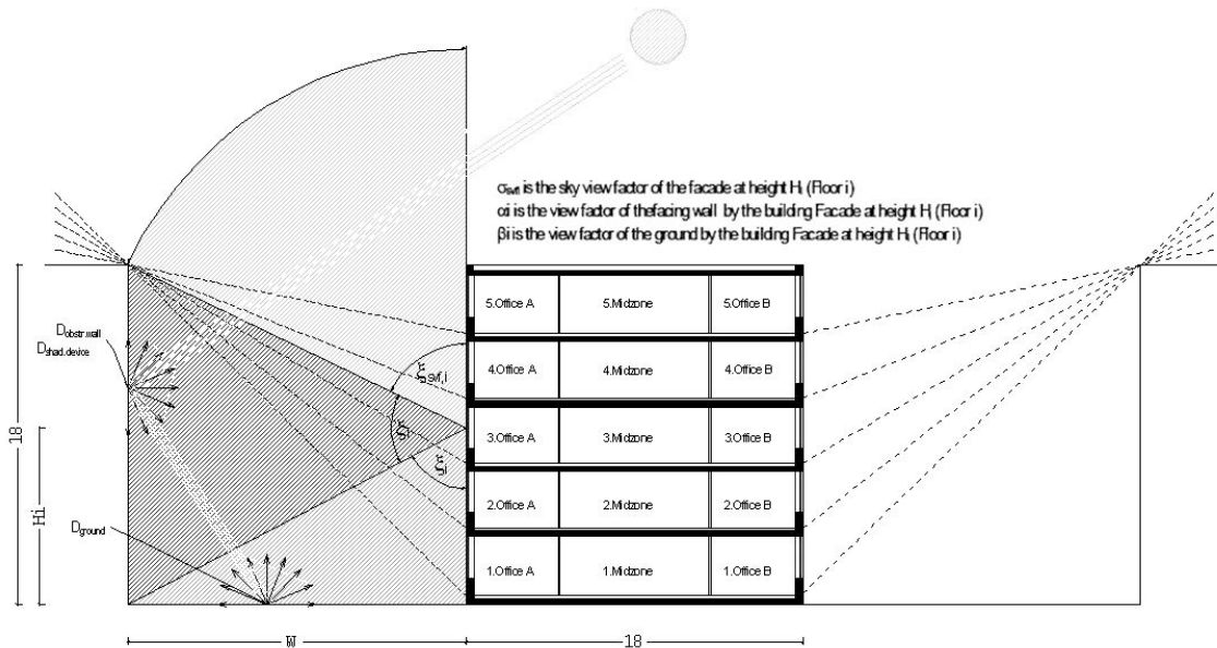
Figure 1: Office Building in a row-type urban structure as simulated with TEB and with TRNSYS 16, including 10 thermal zones with external exposure.
