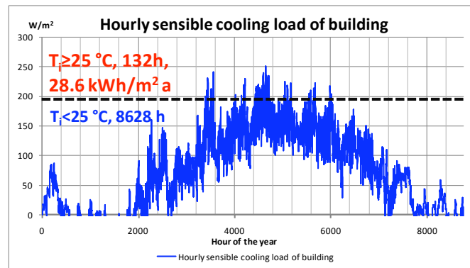
Figure 2: Calculated hourly sensible cooling load of building for whole year and cooling load for cooling season (internal temperature of building is equal or increase 25 °C).
