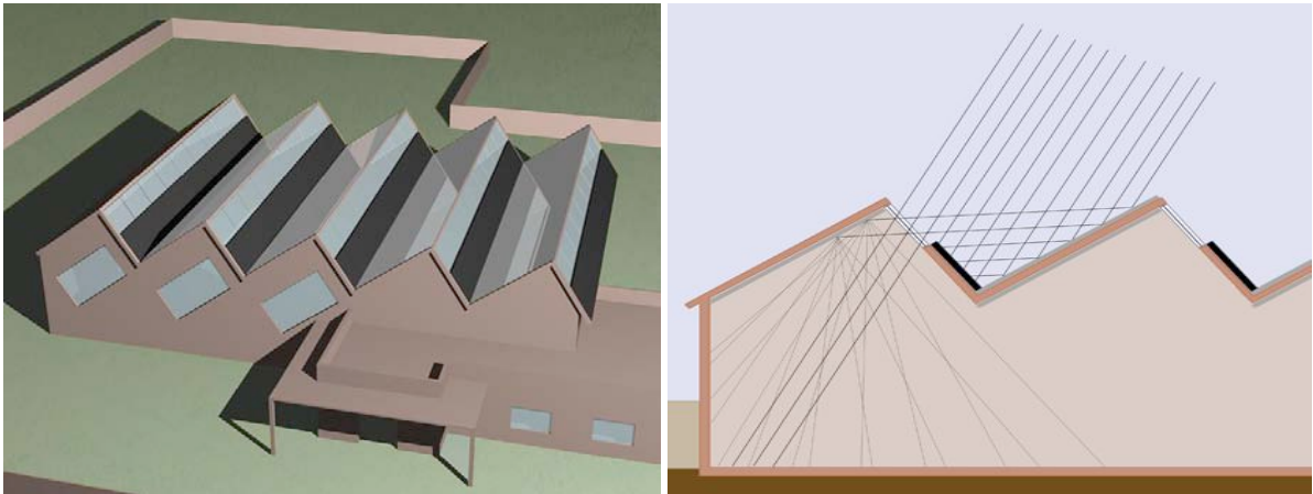
Fig. 1 Architectural design (left) and cross section (right) of building integrated PVT collector combined with booster reflectors and internal space lighting
