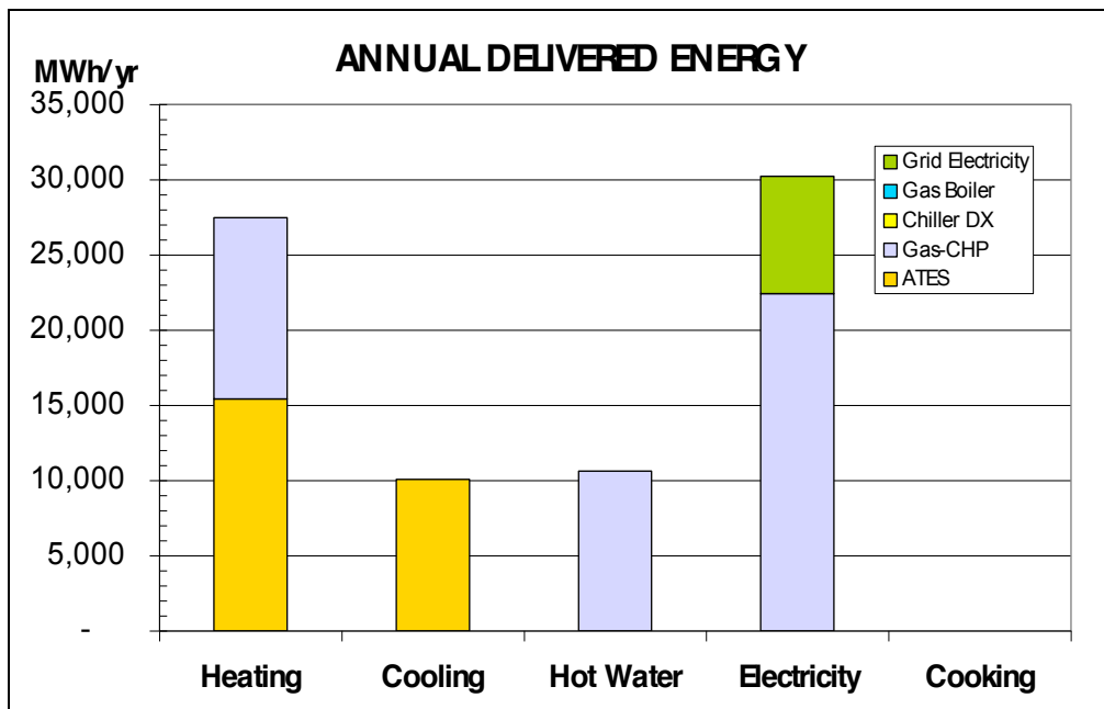
Figure 4: Gas boiler and chiller are replaced entirely by CHP and ATEs.
