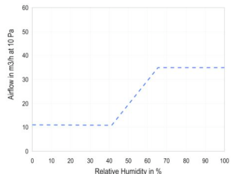
Figure 1: humidity sensitive sensor of an air inlet made of polyamide textile and resulting airflow as a function of relative humidity
