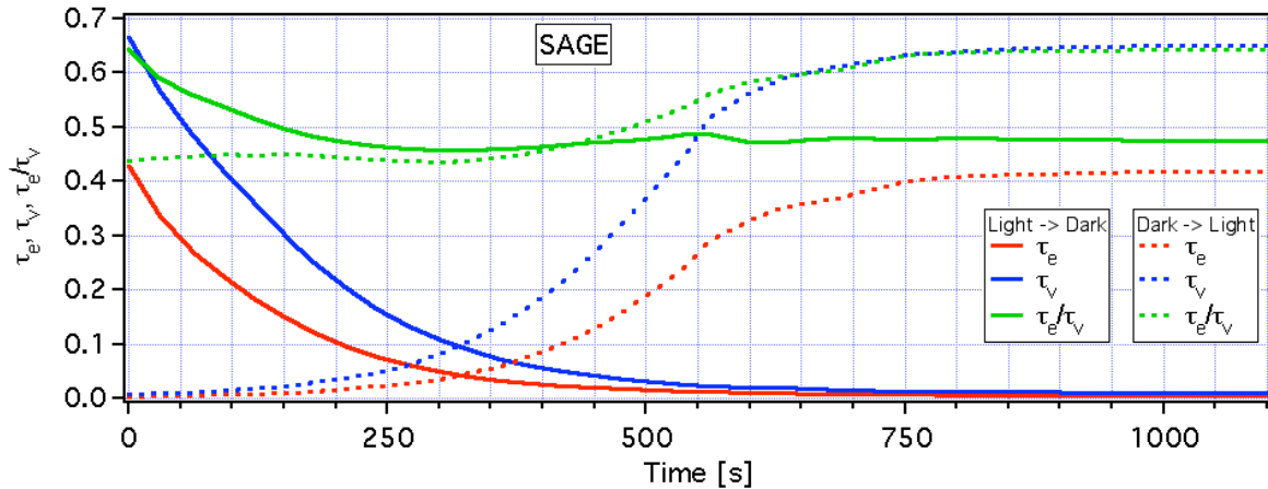
Figure 6: The evolution of the light transmittance \tau_v , the solar direct transmittance \tau_e , and the energy load coefficient \tau_e/\tau_v for the SAGE glass, when switching from bright (1) to dark (2).
