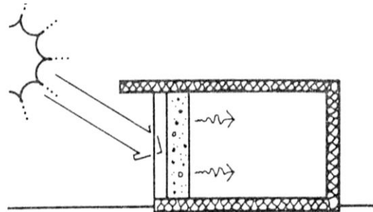
Figure 4: indirect gains, massive wall. Exploitation of solar heat accumulated by an element with high thermal inertia placed between the sun and the environment that needs heating.
