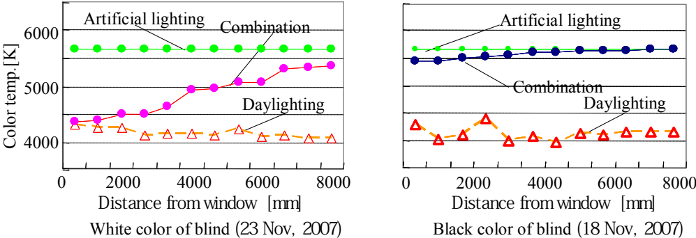
Figure 16: Influence of color of blinds on spatial distribution of color temp.
