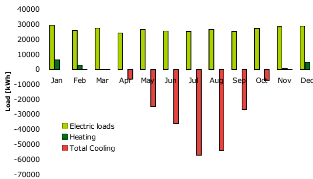
Figure 2: Monthly energy demand for heating, cooling and electricity.
