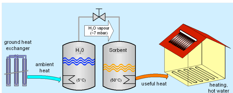
Figure 2: Heating mode. Vapour is absorbed by the sorbent.
