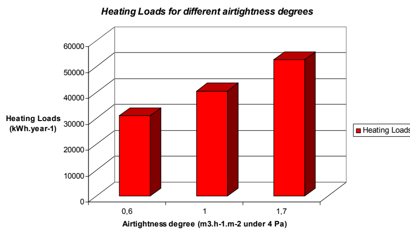
Figure 5: Heating Loads for different air tightness degrees
