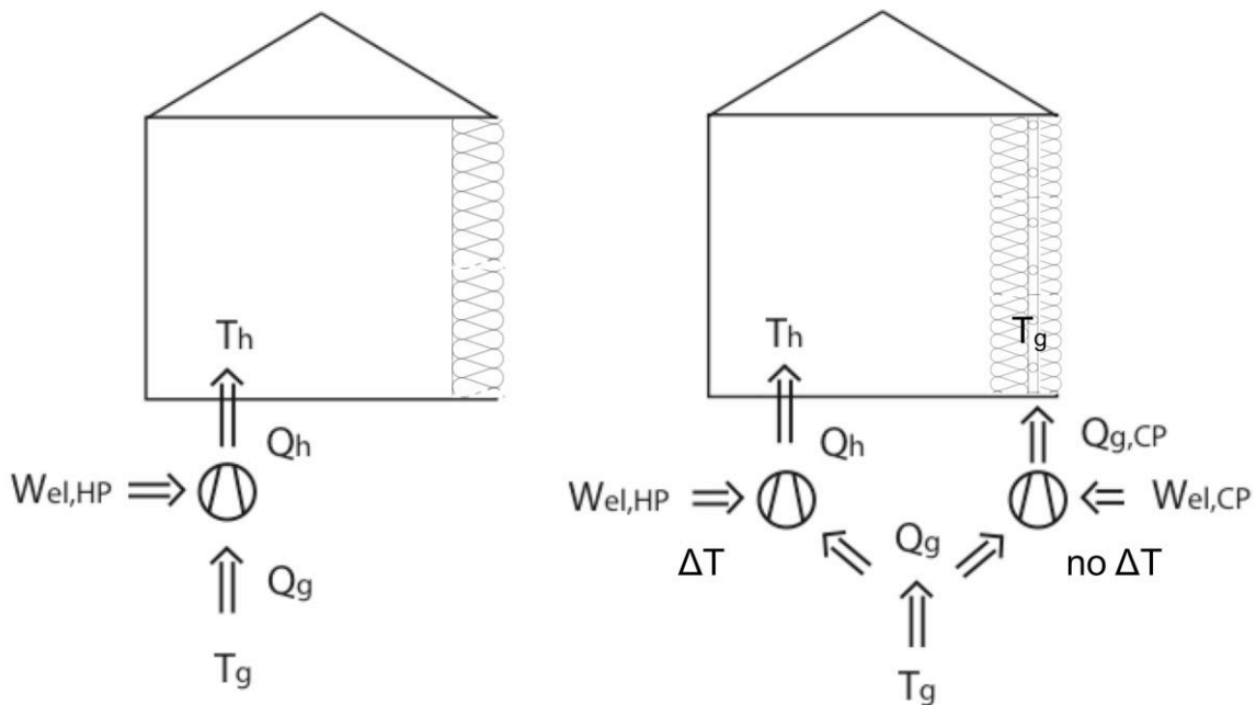
Figure 1: In a standard ground source heat pump setup all the heat, Q_h , must be provided at a higher temperature, T_h , which requires electric heat pump compressor work, W_{el,HP} , to extract the ground heat, Q_g , whereas with the active insulation system part of the ground heat can be used directly without the need for a temperature lift with only a small amount of electric work for the circulation pump, W_{el,CP} .
