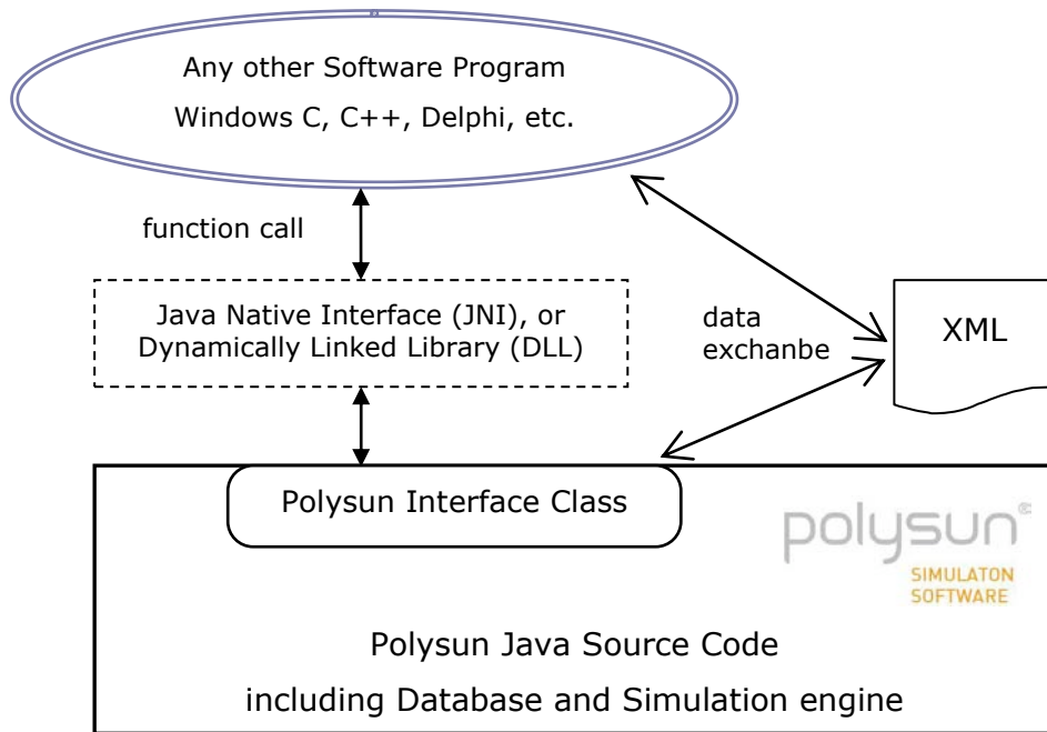
Figure 3: Concept of the software interface to the Polysun kernel.
