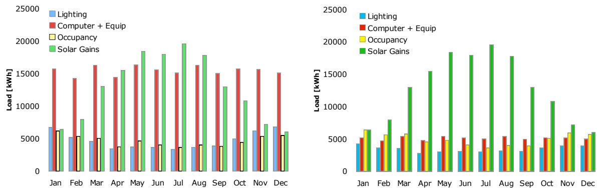
Figure 3: Monthly energy load by int. and solar gains. A) baseline; B) high-efficiency.
