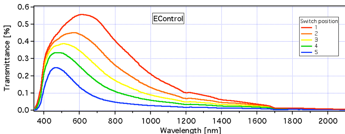
Figure 1: The spectral transmittance of the EControl glass for the five different switch positions, where 1 corresponds to the uncoloured and 5 to the darkest coloured state.
