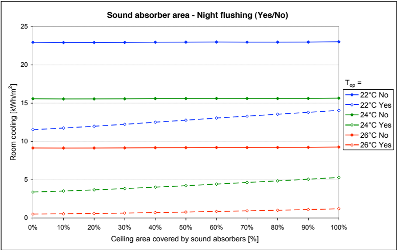
Figure 2: Cooling energy demand for various temperature set-points and with or without night flushing, as function of the ceiling area covered by sound absorbers
