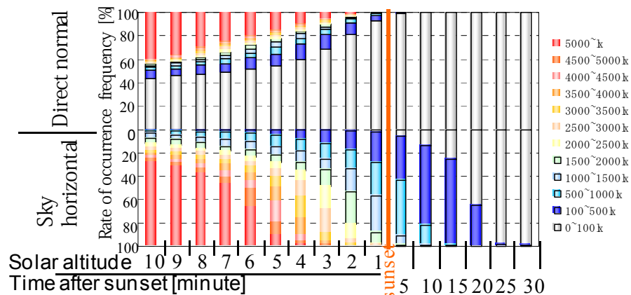
Figure 7: Change of sunlight around sunset.
