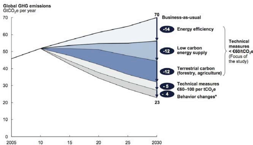
Figure 5: With costs of less than 60€ per ton of \text{CO}_2\text{eq} more than half of the worldwide greenhouse gas emissions (38 Gt of 70 Gt \text{CO}_2\text{eq} ) may be reduced through technical measures by 2030 [5]. The oil price is assumed to be 60$/barrel. The contribution of behavior changes is small because many are already included in the above mentioned measures.
