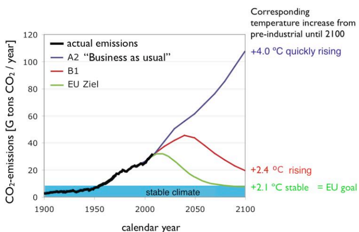
Figure 1: Actual emissions (solid line) increase faster than assumed in the IPCC business as usual scenario, mainly due to the lower energy efficiency in the developing countries. To stabilize the climate requires the global emissions to fall well below 10 G tons of CO 2 . The more carbon we emit into the atmosphere until we reach this goal, the higher will be the corresponding temperature and climate change. [2]
