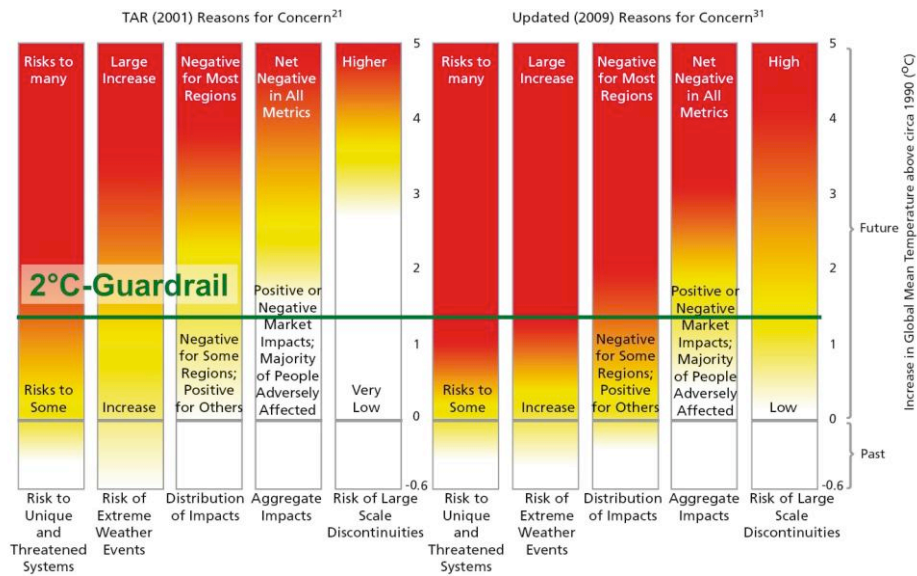
Figure 4: The impact of climate change and thus the reasons for concern are considered higher today as valued by the expert in 2001 in the IPCC Third Assessment Report TAR. Increasing risks are symbolized by the red color for different threats. [4]
