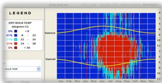
Figure 3: time table plot, extract from Climate Consultant 04 CC04
