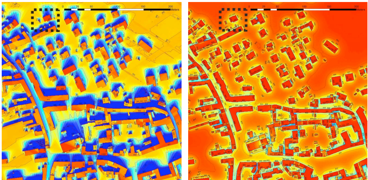
Figure 1: Daily direct and diffuse solar radiation map, average values in January, Wh/sqm. The dotted square shows the building chosen.
