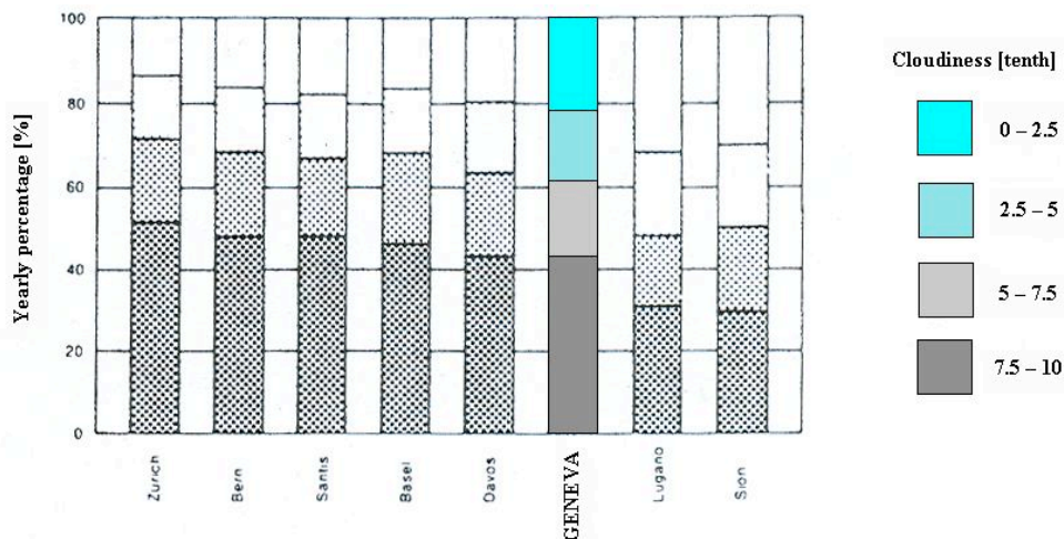
Figure 2: Yearly percentage, in tenths, of the different levels of cloudiness in some Swiss locations, adapted from [5].
