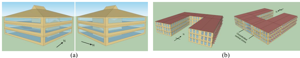
Figure 2: EnergyPlus Building Models viewed in Google SketchUp, (a) light-weight mechanically controlled building and (b) mixed-mode office building
