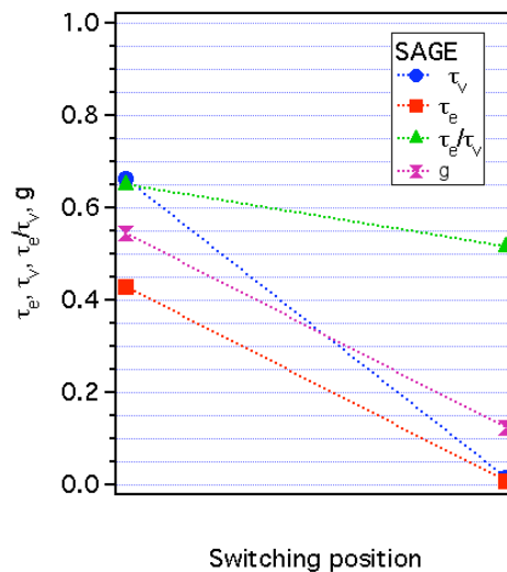
Figure 4: Light transmittance \tau_v , solar direct transmittance \tau_e , energy load coefficient \tau_e/\tau_v , and g -factor for the SAGE glass depending on the colouring state. The markers give the values where as the lines are guides for the eyes.
