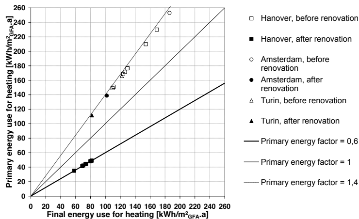
Figure 1: Correlation between primary and final energy use for heating (space heating and domestic hot water)
