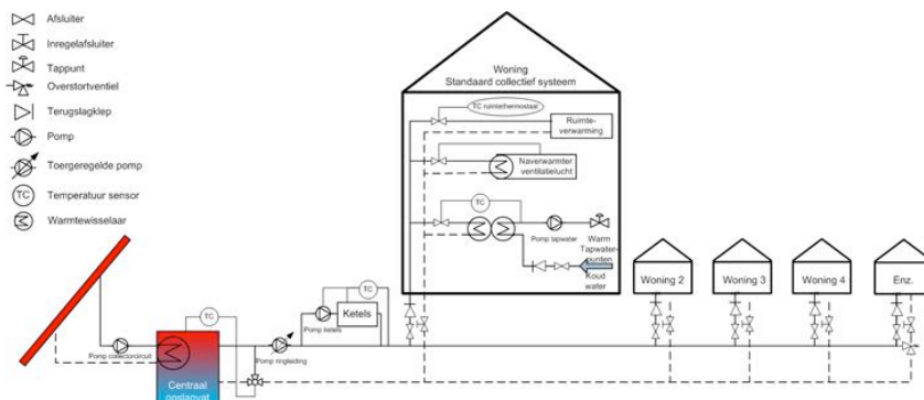
Figure 6 Solution III small distribution network.
