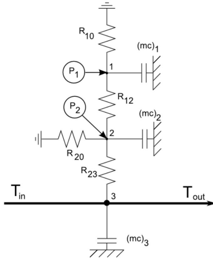
Fig.2. Equivalent Thermal Network for one collector in a transient state.
