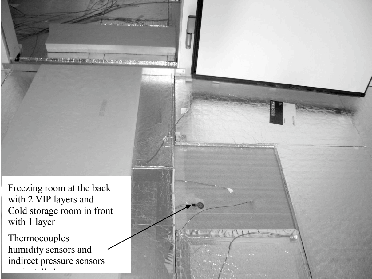
Figure 4: VIP installed in the floor of a cold storage room
