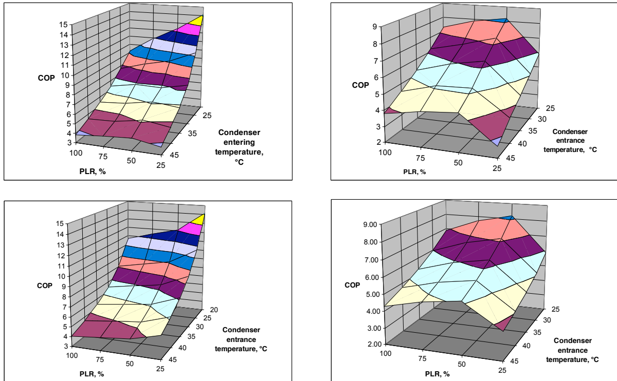
Figure 2: Performance maps of two chiller types: original data (upper row), model generated (lower row) for chiller type 1 (left) and type 2 (right)
