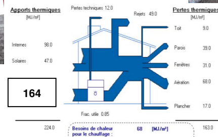
Figure 4: Before refurbishment, the building consumption for heating and hot water is 734 MJ/m 2 (class G). After refurbishment, energy consumption according to standard conditions is reduced to 164 MJ/m 2 . Although after refurbishment airflow is drastically reduced, the part of ventilation losses, according to standard conditions, represents 41% of total losses.
