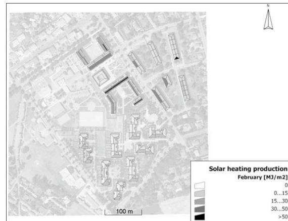
Figure 6: Monthly energy production for heating with glazed collectors
