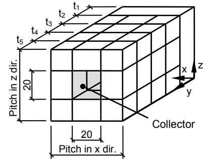
Figure 2: ESP-r model.
