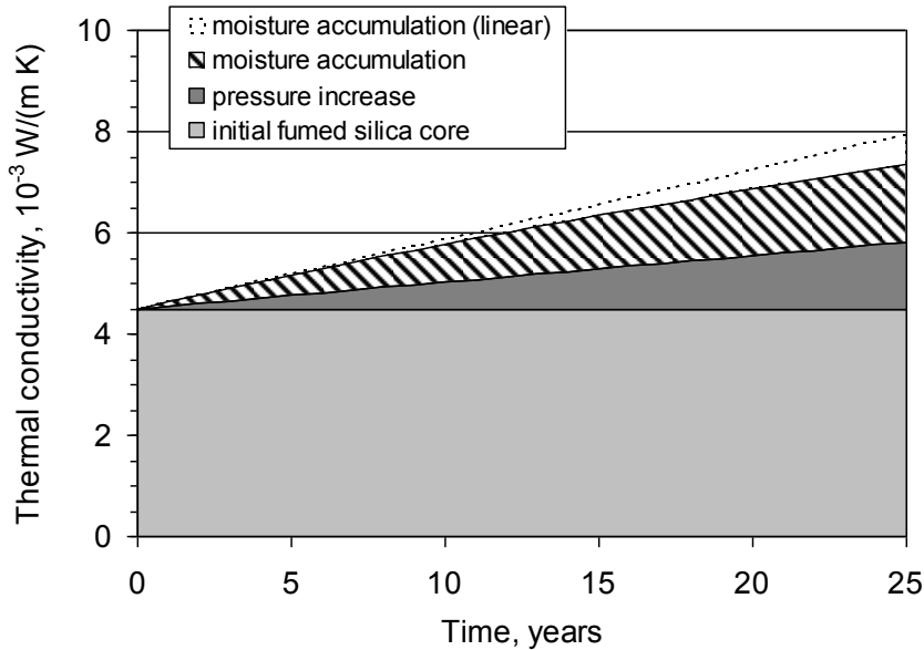
Figure 1: Predicted effect of pressure increase and moisture accumulation on the thermal conductivity of VIP (format 100 \times 60 \times 2 \text{ cm}^2 ) over a period of 25 years. The dotted line indicates the increment omitting moisture saturation [7]
