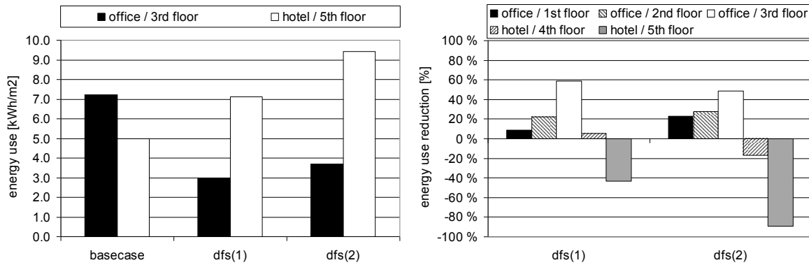
Figure 4: Summed net energy demand for heating in office and hotel room (left) and percentage energy demand for heating compared to base case in all rooms (right).
