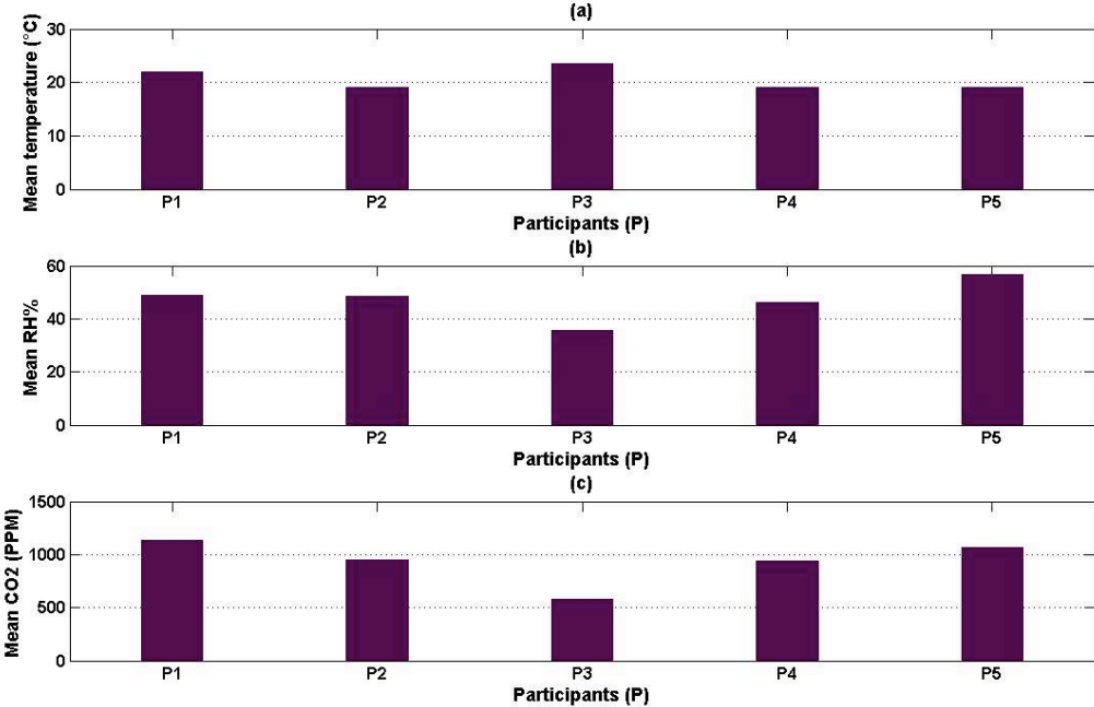
Figure 1: Mean temperature, relative humidity and carbon dioxide for each home
