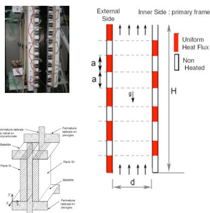
Figure 2 : Experimental Apparatus
