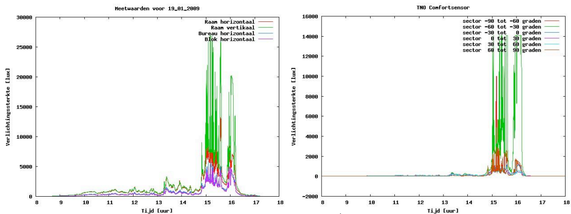
Figure 3. Daylight measurements on a sunny day (January 19 th , 2009), with illuminances on the glass and horizontal work plane (left), and illuminances as measured by the DDD in six viewing directions (right)
