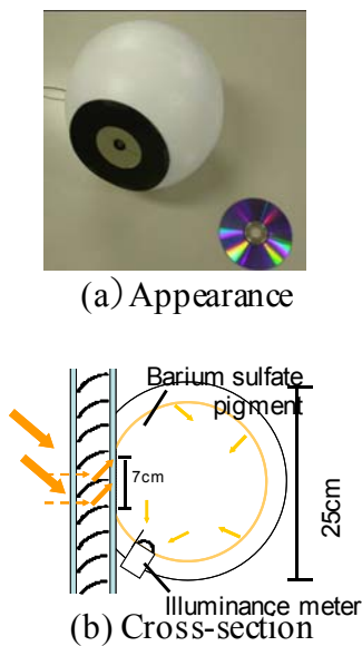
Figure 13: Proposed integral sphere.
