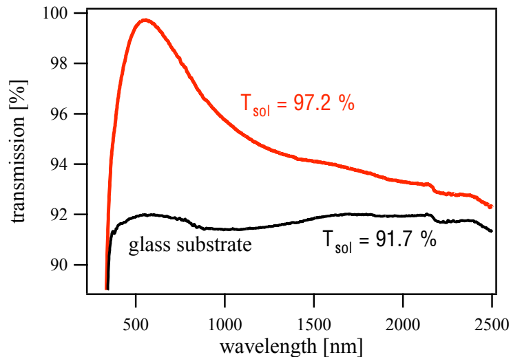
Fig.2: Broad band antireflection of solar collector glazing by novel quaternary Mg-F-Si-O coatings developed at LESO-PB. The solar transmittance can be raised from 91.7% for the uncoated white solar glass to 97.2% for the coated glass. In order to achieve antireflection in the full solar range (UV-VIS-NIR), a low refractive index around 1.22 is necessary. This has been achieved previously only by nanoporous \text{SiO}_2 films, and such coatings are entering the market now. The novel Mg-F-Si-O films might be more resistant towards gradual pore filling by hydrocarbons.
