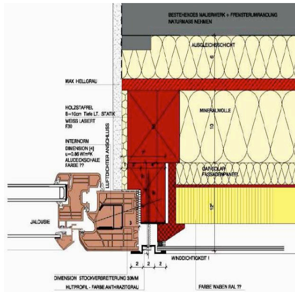
Figure 3: Cross section of the solar insulation system of the Linz apartment building. (Source: Domenig-Meisinger)
