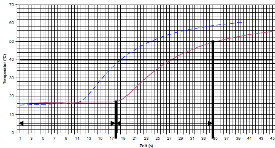
Figure 1: Laboratory measurement of the temperature rise after opening a hot water tap in a hardware configuration that simulates a typical situation in a dwelling. Dashed line: 9 m pipe length. Solid line: 15 m pipe length. Two phases are visible: first, expulsion of the pipe water content at ambient-temperature; second, warming-up of pipe work and fittings. Horizontal solid lines: two possible threshold temperatures for the definition of the draw-off lag. [3]
