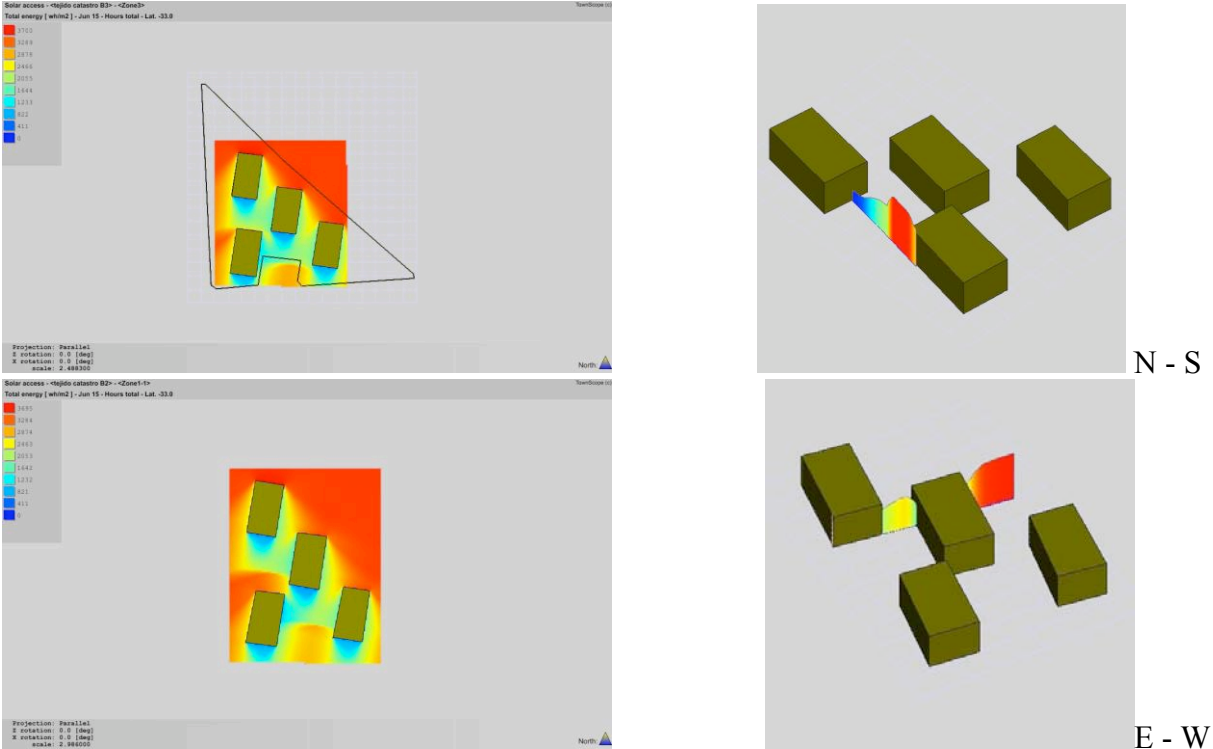
Figure 3: Solar Radiation Modelling on urban fabric: the BC model. (plan and cross-section)
