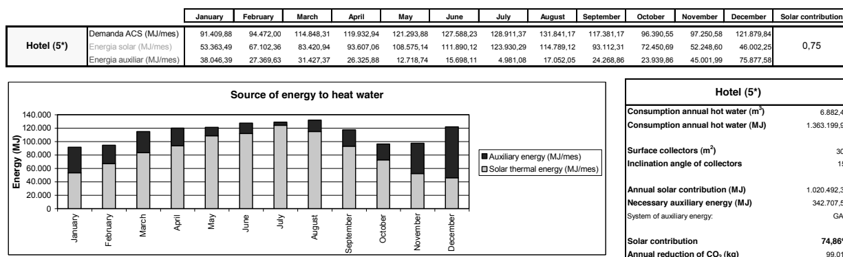
Figure 6: Example of a presentation of results for solar thermal energy. Hotel 5.
