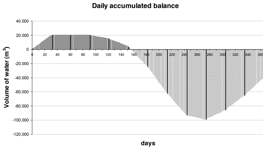
Figure 4: Daily accumulated balance with 20.000 m 3 as a maximum volume of restriction.
