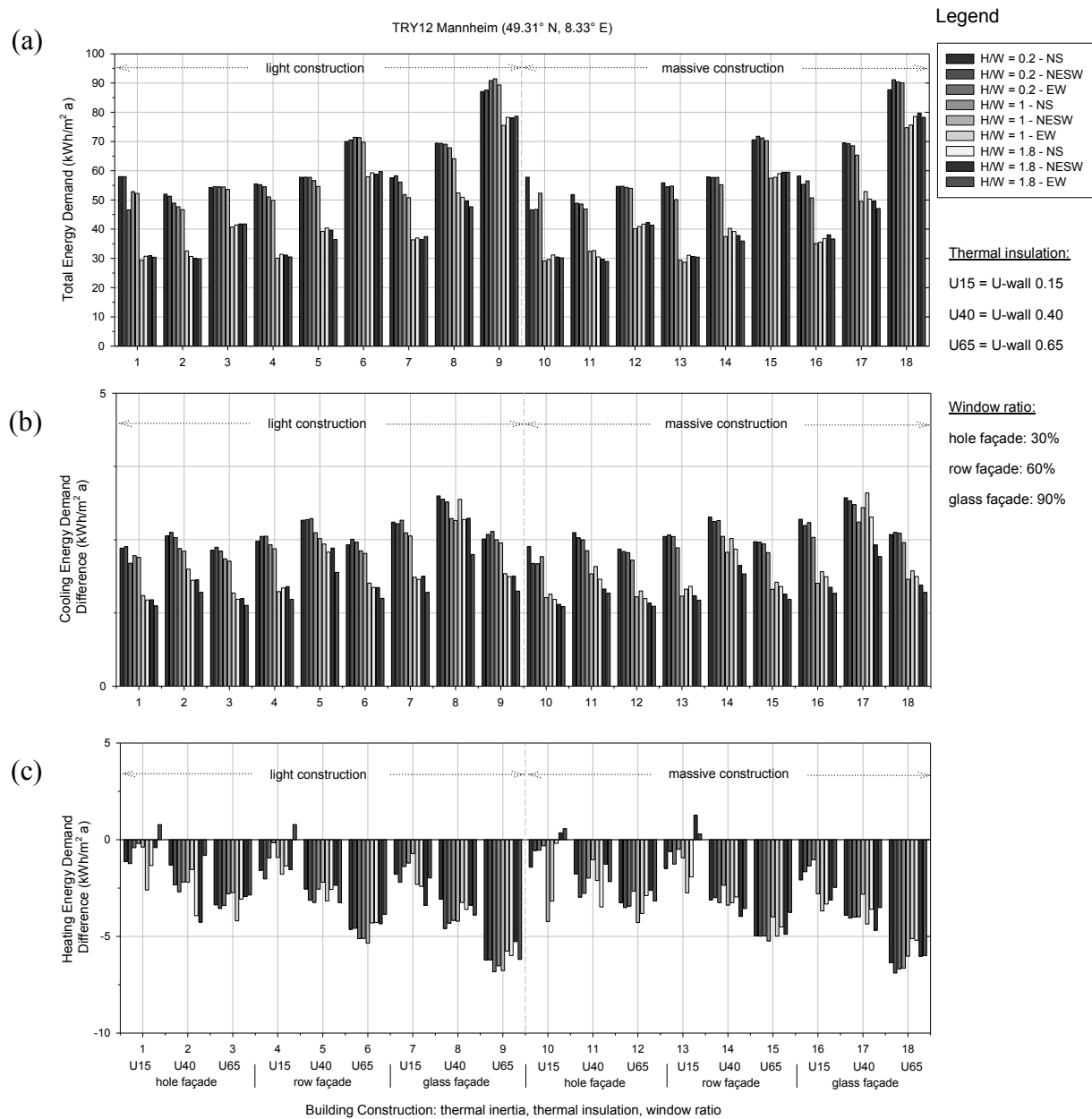
Fig. 3: (a) Total energy demand for Mannheim (49.31 °N) in dependence with urban and building descriptors and a comparison for (b) cooling and (c) heating between urban climate data versus standard data as inputs
