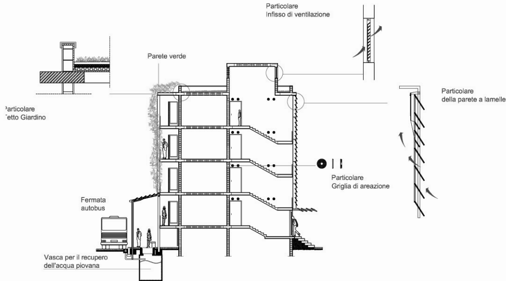
Figure 6 - Technological section of the rehabilitated building
