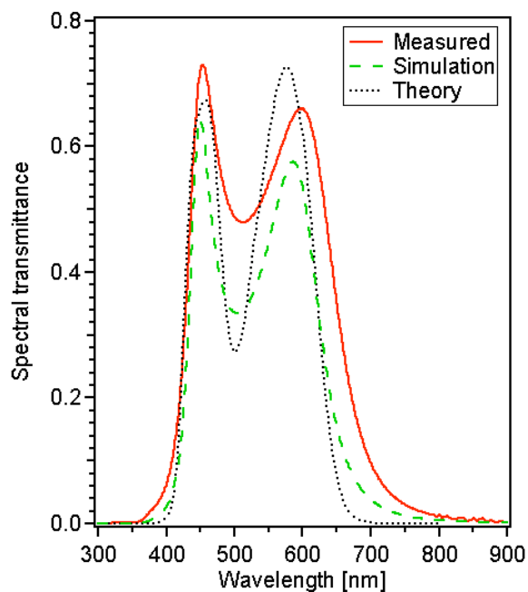
Figure 1: The measured spectral transmittance of the multilayer coating, the simulation used for the deposition, and the theoretical curve of the optimised spectral transmittance for perpendicular light incidence.
