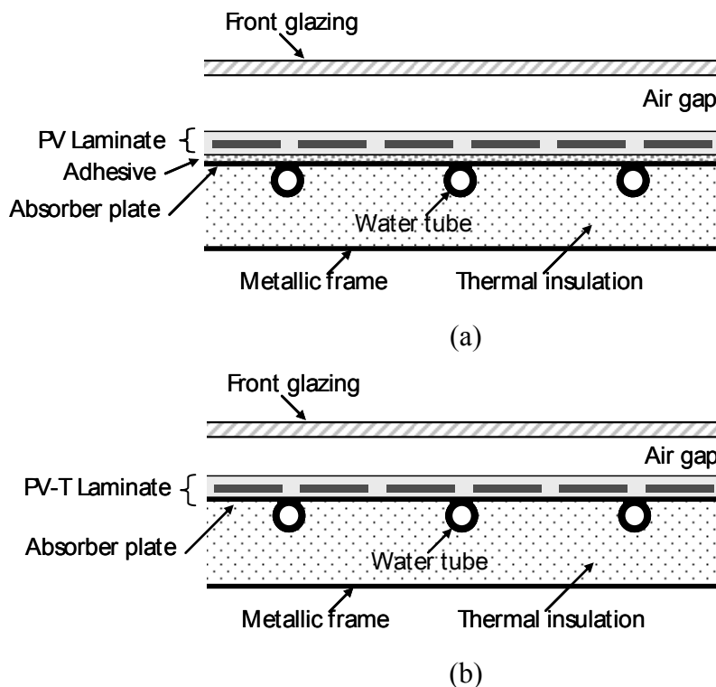
Figure 1: Flat plate PV-T collector. (a) Gluing of pre-laminated PV module on metal absorber. (b) Direct lamination of PV module component on a metal absorber
