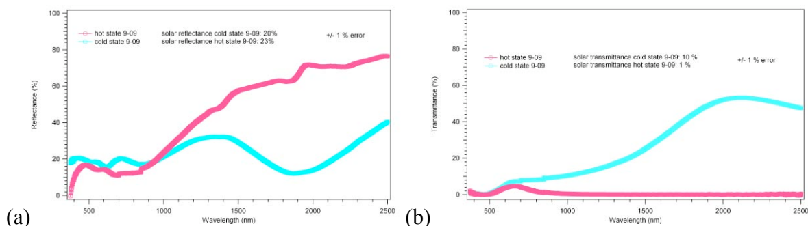
(a) Reflectance of a VO 2 :W sample on glass at ambient temperature and at 90°C. (b) Transmittance of a VO 2 :W sample on glass at ambient temperature and at 90°C. For each curve the respective fraction of transmitted and reflected energy in the range of the solar spectrum is calculated.
