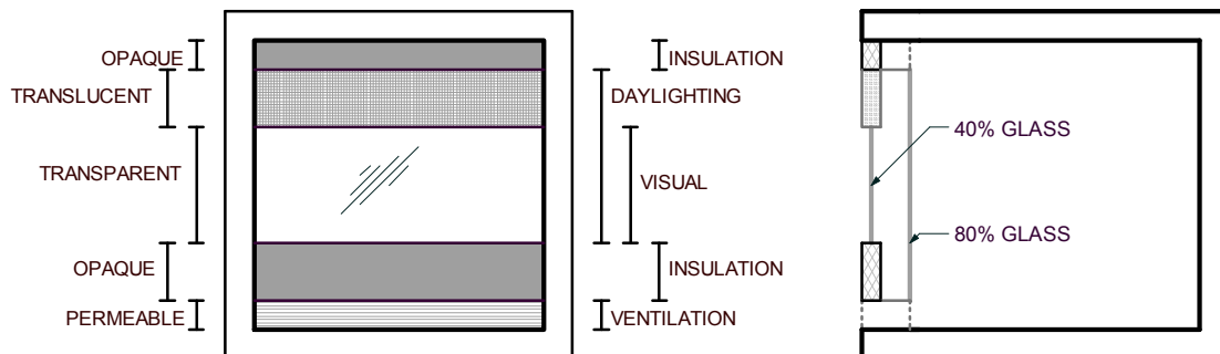
Figure 1. Geometry and construction solution of analysed façade – base case.
