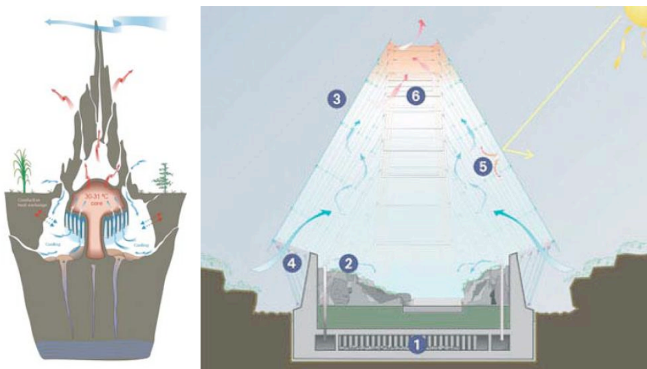
Figure 3: The working principle of the nest of the Barossa termite (Bellew 2006) and climatic principle of the Alpine house (Spring 2006).
