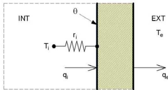
Figure 1 – External wall schematization.
