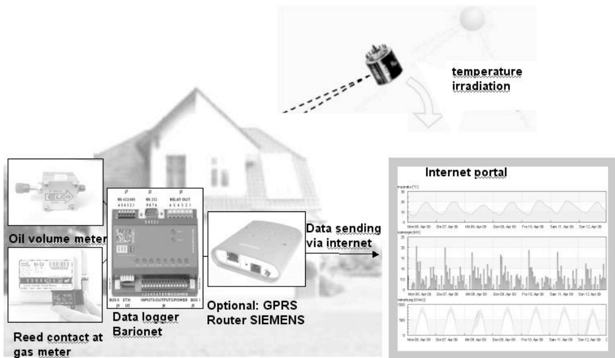
Figure 1: Principle of the system, including hardware on-site and a central internet portal
