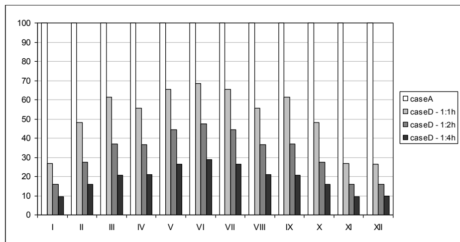
Figure 5. Comparison of solar direct radiation for different building height in case D.
