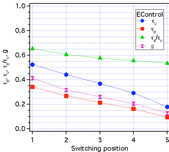
Figure 3: Light transmittance \tau_v , solar direct transmittance \tau_e , energy load coefficient \tau_e/\tau_v , and g -factor for the EControl glass depending on the colouring state. The markers give the values where as the lines are guides for the eyes.
