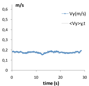
Figure 5 : Velocity fluctuations along the channel
