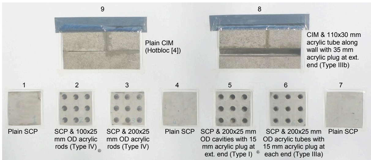
Figure 5: 250 mm thick stratified concrete panel (SCP) and 240 mm thick cavity-insulated masonry (CIM) north-facing test walls at Christchurch (43.5°S). Collectors cover 15-16% of walls 2, 3, 5, 6, and 8.
