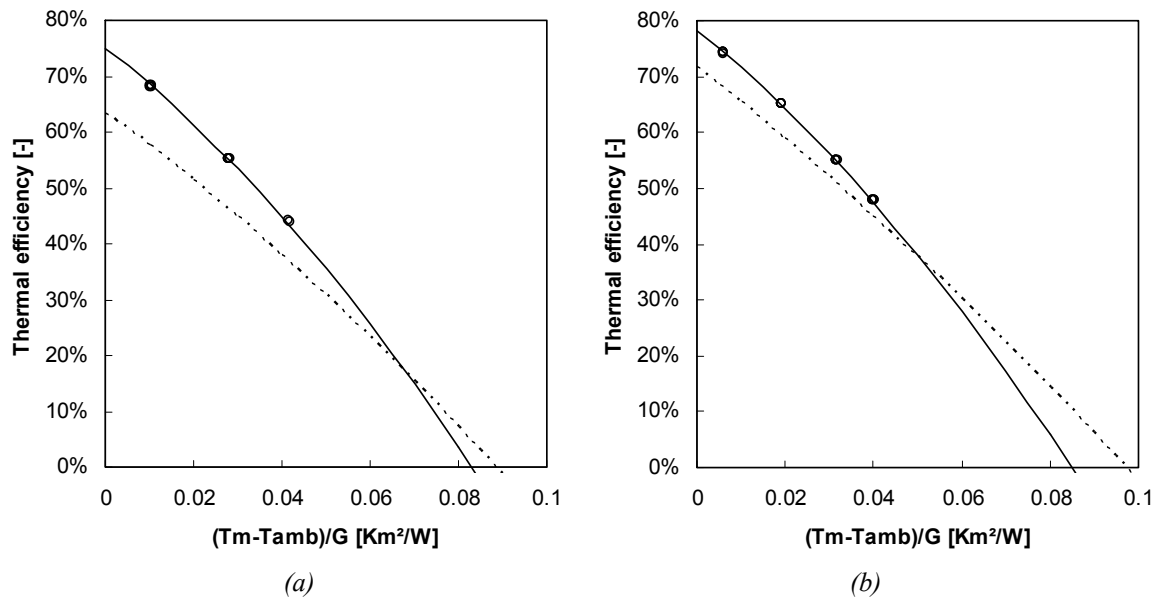
Figure 3: Thermal efficiency curve (a) with PV extraction (Maximum Power Point) ; (b) without PV extraction (open-circuit). Dashed line: commercially available sheet and tube PV-T collector, dots: measurements point for small laminated experimental PV-T collector, full line : corresponding polynomial fit.
