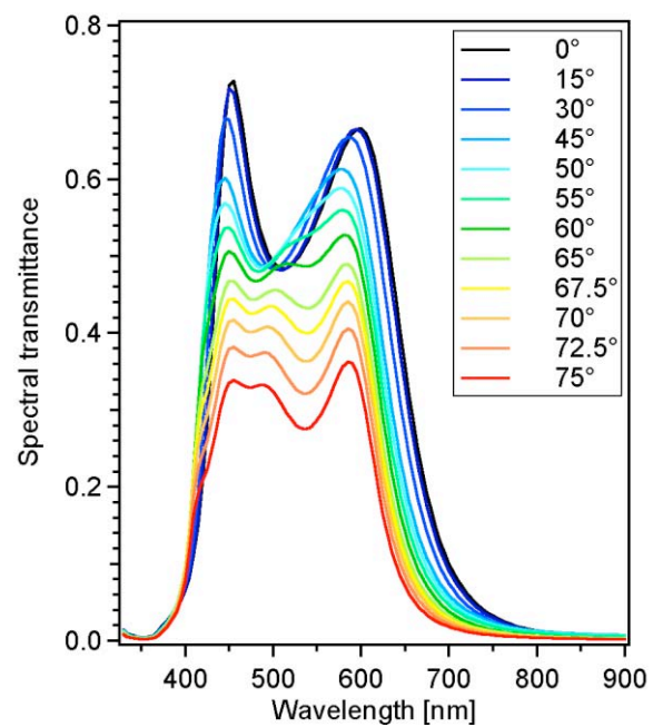
Figure 2: The measured spectral transmittance for different angles of light incidence.
