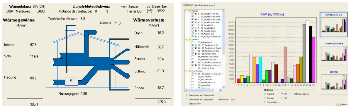
Figure 2: Typical output generated by Lesosai include Sankey diagrams (left) and detailed environmental impact calculations (right).
