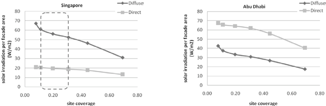
Figure 4: Solar irradiation (W/m²) on building facades of the central block vs. site coverage
