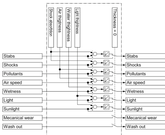
Figure 4: Illustration of constraints propagation
