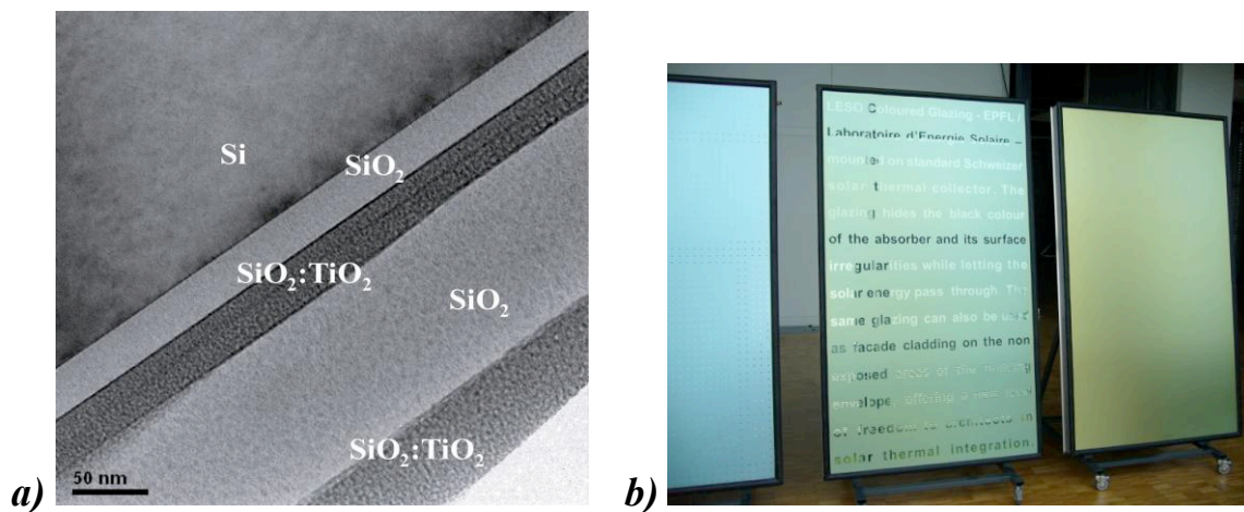
Fig.3: Coatings for colored solar thermal facades, developed at LESO-PB. The energy losses due to the coloration can be kept below 5%.
