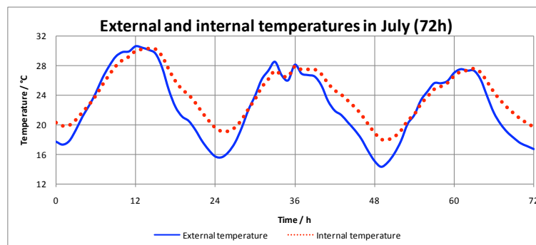
Figure 1: Dynamics of external and calculated internal temperature of building
