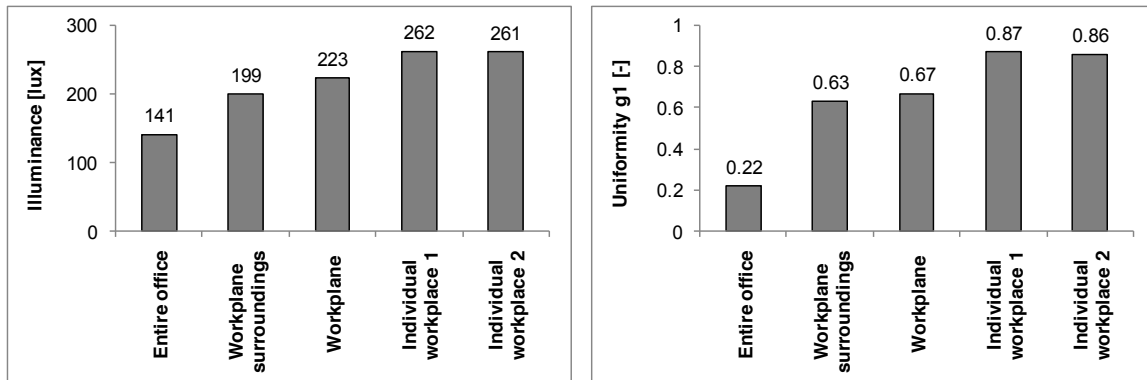
Figure 5: Resulting average illuminances and uniformities g_1 (i.e. the lowest illuminance value measured on a particular reference plane divided by the corresponding mean illuminance) for the LED lighting design (cf. Figure 4).
