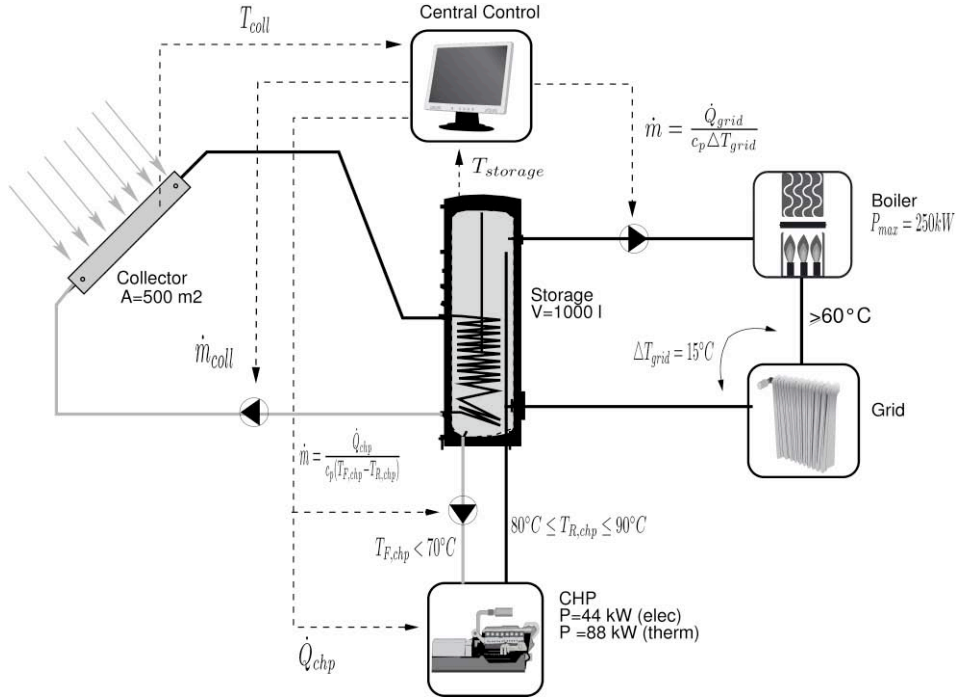
Figure 2: Hydraulic schematic and control schematic of the heating system.
