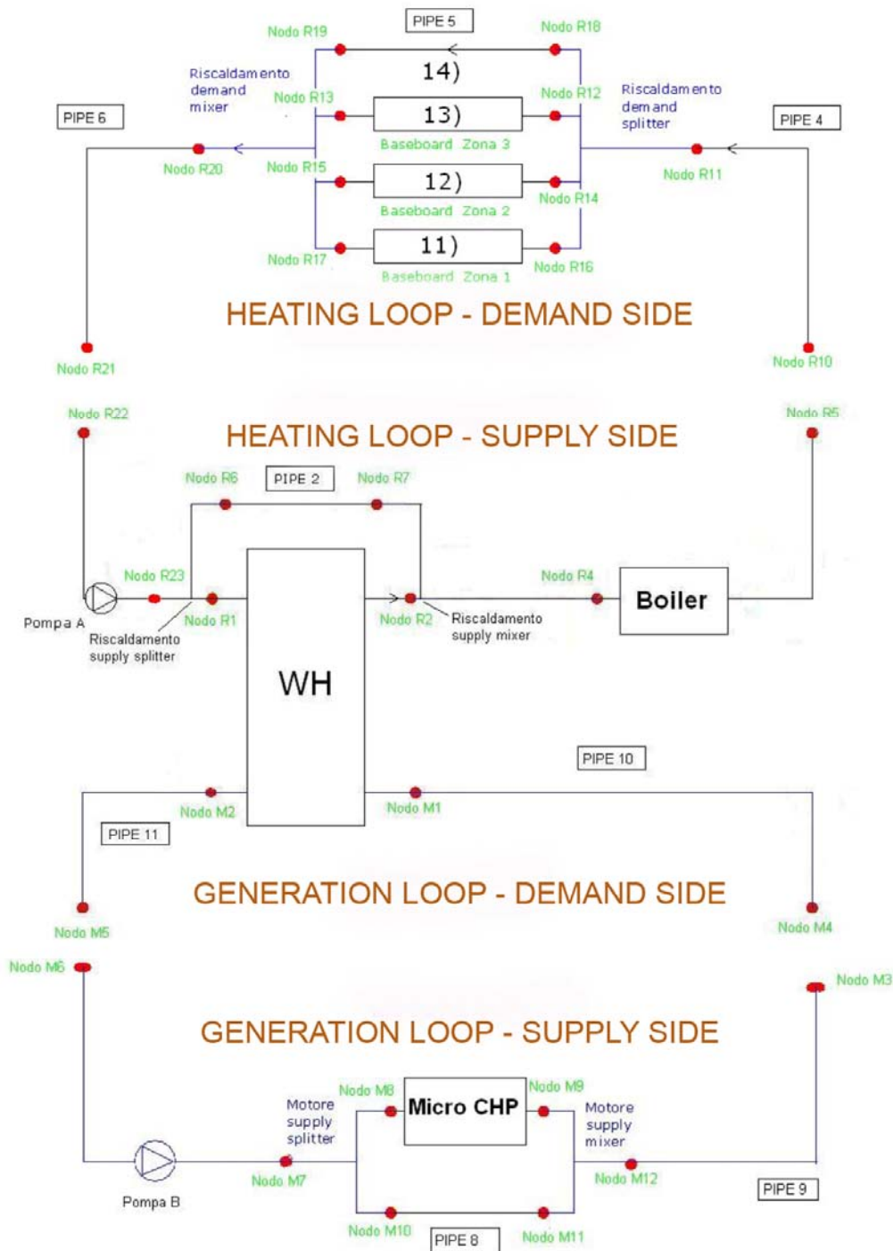
Figure 2: Model's heating plant scheme
