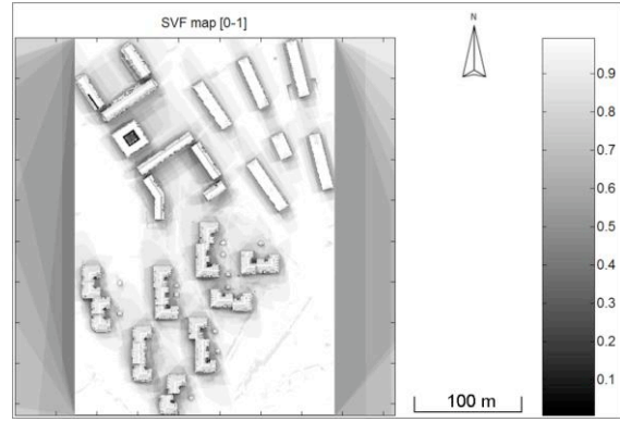
Figure 2: The sky view factor. The average SVF on the roofs is 0,83
