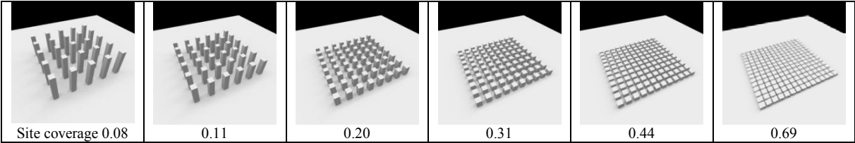
Figure 3: Regular urban arrays with different levels of site coverage
