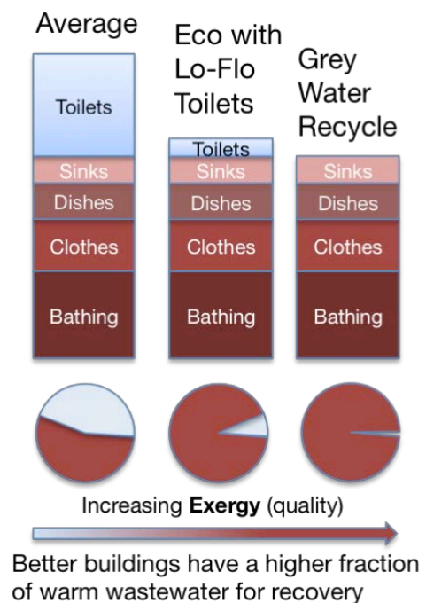
Figure 2: Exergy available in building wastewater streams
