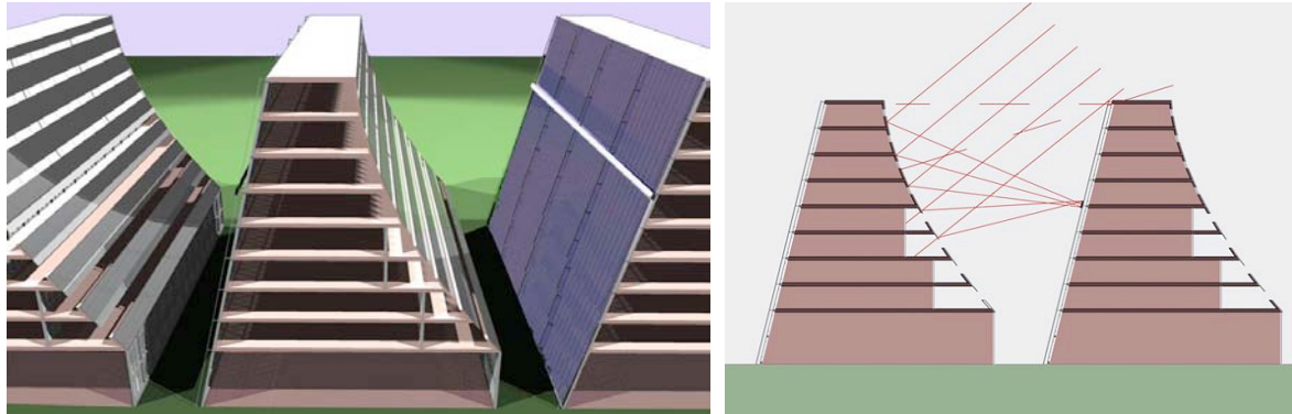
Fig. 6 Building integration of stationary reflectors with tracking PV or PVT absorber
