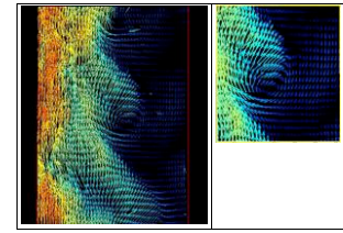
Figure 6: Vortex at exit region
