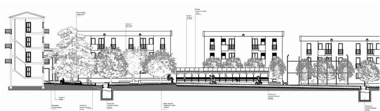
Figure 2 - Longitudinal section of the pedestrian area
