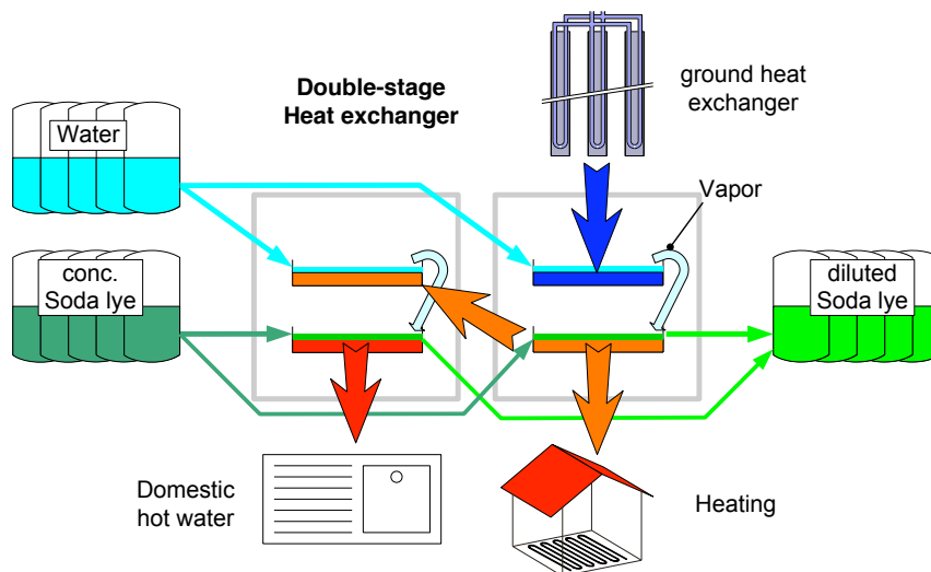
Figure 4: Discharging mode. The produced heat of the first stage is used for heating and for evaporating water in the second stage. High temperature heat produced in the second stage is used for domestic hot water.
