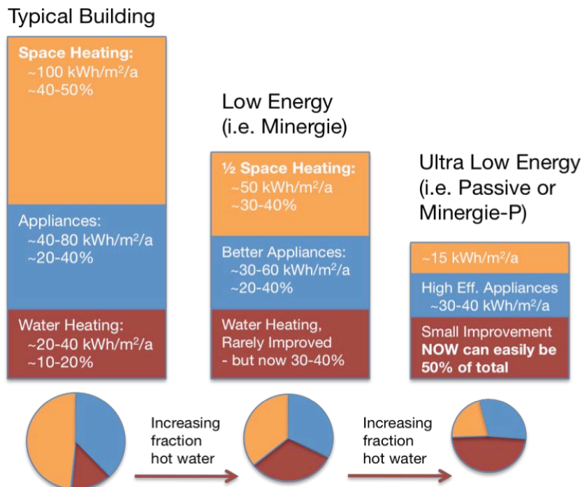
Figure 1: As building performance levels increase the focus is primarily on space heating because it was the largest part in the beginning, but now further advancements must start to address the issue of warm water energy demand.
