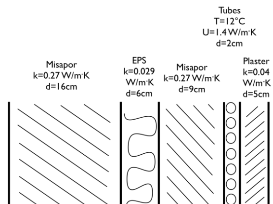
Figure 2: B35 wall construction layers and piping outside piping system
