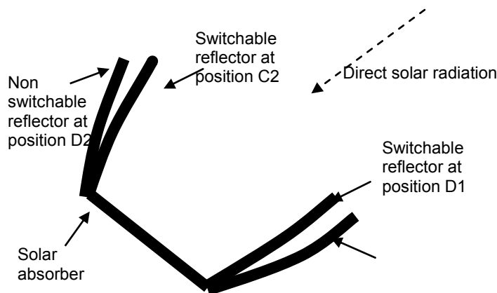
Figure 2: A switchable CPC device
