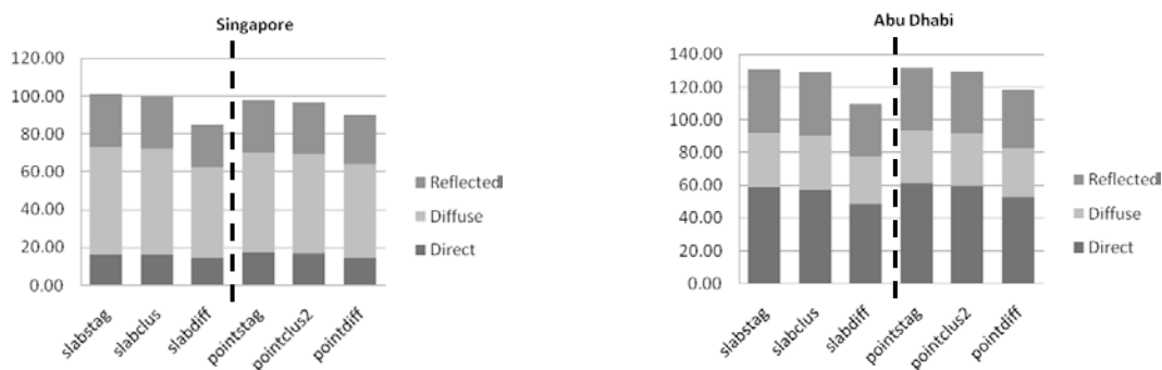
Figure 9: Solar irradiation ( W/m^2 ) on building facades of the central block of generic forms with different clustering conditions (dash line: change in base case)
