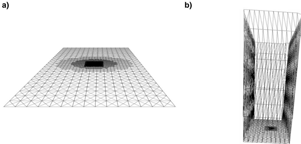
Figure S1-1: a) Used grid for the substrates corresponding to 1600 \mu\text{m} \times 1600 \mu\text{m} . The size of the elements is reduced under the active electrode area. The total number of elements is 3484 (conducting sample) and 7725 (insulating sample). b) Grid of the lower part of the soft stylus probe with a height equal to 520 \mu\text{m} . The polished cross section corresponds to 480 \mu\text{m} \times 200 \mu\text{m} . The electrode body and the active area is represented by 1482 triangles (conducting sample) or 3768 triangles (insulating sample).
