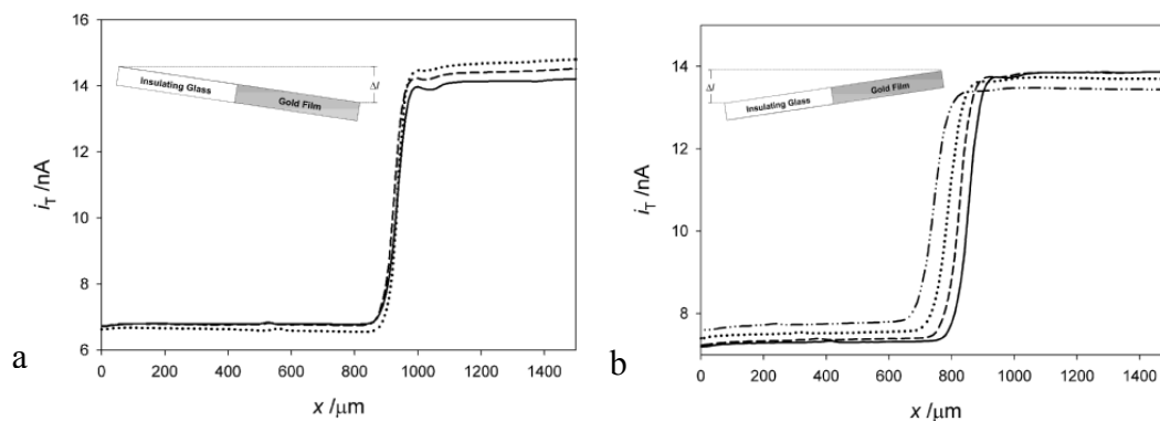
Figure S3-1. Lateral SECM line scans in feedback mode with a polished soft stylus probe over a glass partially covered by gold in 2.4 mM \text{FcCH}_2\text{OH} , 0.1 M \text{KNO}_3 . The sample was tilted from the glass towards the gold region a) downhill b) uphill. The height difference ( \Delta l ) between the starting (over glass) and final (over gold) points was varied; 20 \mu\text{m} (continuous line), 30 \mu\text{m} (dashed line), 50 \mu\text{m} (dotted line) and 90 \mu\text{m} (dashed-dotted line). E_T = 0.3 V, step size = 10 \mu\text{m} and v_T = 10 \mu\text{m/s} , h_P = -75 \mu\text{m} .
