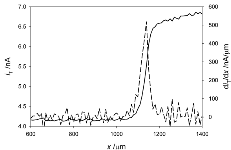
Figure S4-1. Lateral SECM line scan in feedback mode (continuous line) with a soft stylus probe prepared by mechanical polishing over a glass-gold boundary in 2.1 mM \text{FcCH}_2\text{OH} , 0.1 M \text{KNO}_3 . Numerical differentiation of the line scan presented (dashed line). h_p = -5 \mu\text{m} , E_T = 0.3 \text{ V} , step size = 10 \mu\text{m} and translation rate v_T = 10 \mu\text{m/s} .
