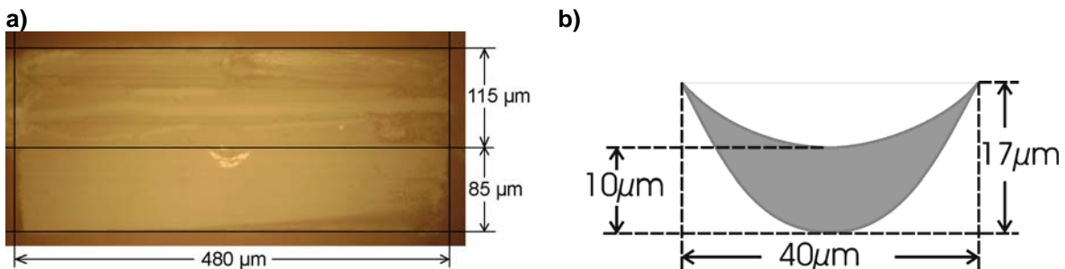
Figure S1-2: a) Optical microphotograph of the polished cross section of the soft stylus probe. b) Shape and extension of the active electrode area considered for the BEM simulation.
