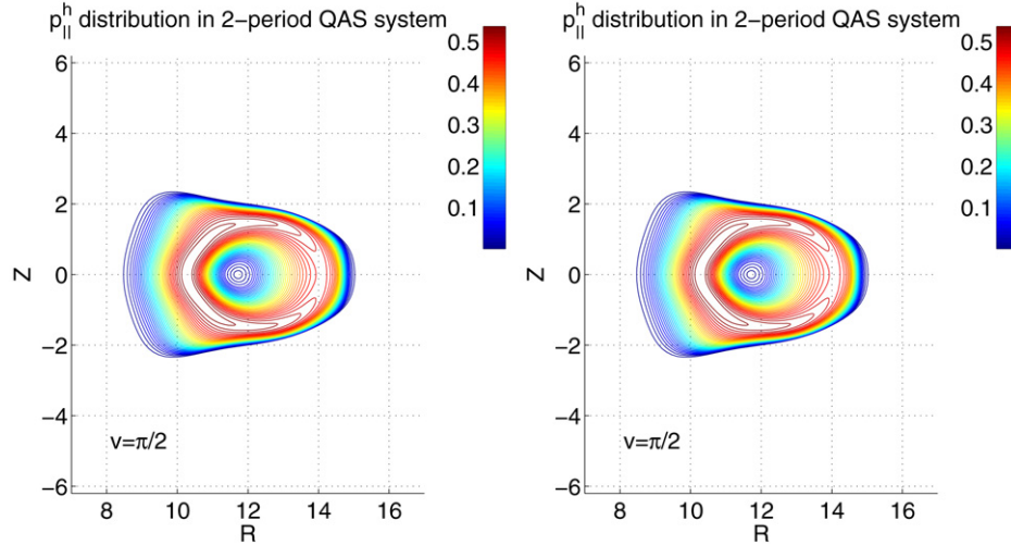
Fig. 16. The hot particle parallel pressure p_{\parallel}^h contours for p_{\parallel} > p_{\perp} HF side deposition ( B_c = 4.9T ; \langle \beta_{\perp}^h \rangle / \langle \beta_{\parallel}^h \rangle \simeq 1/3.4 ) (left) and p_{\parallel} > p_{\perp} LF side deposition ( B_c = 4.2T ; \langle \beta_{\perp}^h \rangle / \langle \beta_{\parallel}^h \rangle \simeq 1/3.4 ) (right) at midperiod in a 2-field period quasiaxisymmetric stellarator reactor at \langle \beta \rangle \simeq 4.5\% .
