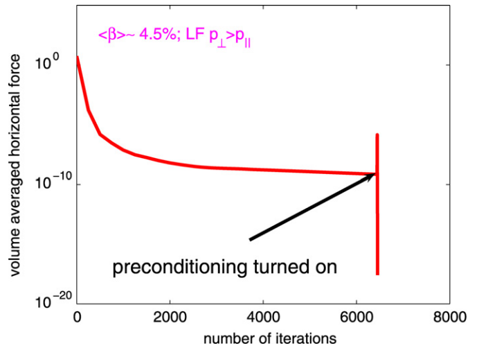
Fig. 6. The volume average of the residual horizontal force F_R as a function of the number of iterations for the case at \langle\beta\rangle \approx 4.5\% corresponding to B_c = 4.2T and \langle\beta_{\perp}^h\rangle/\langle\beta_{\parallel}^h\rangle \approx 3.4 in a 2-field period quasisymmetric stellarator reactor. The preconditioning algorithm is turned on after 6440 iterations.
