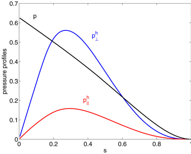
Fig. 2. The flux surface averaged thermal pressure p , the hot particle parallel pressure p_{\parallel}^h and the hot particle perpendicular pressure p_{\perp}^h profiles as a function of the radial variable s (roughly proportional to volume enclosed).
