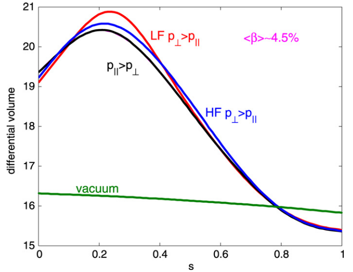
Fig. 11. The vacuum (green line) and the finite \langle \beta \rangle \simeq 4.5\% differential volume profiles in a 2-field period quasisymmetric stellarator system with off-axis energetic particle deposition. The finite \beta cases investigated have (a) B_c = 4.9T ; \langle \beta_{\perp}^h \rangle / \langle \beta_{\parallel}^h \rangle \simeq 3.4 (HF side hot particle deposition with p_{\perp} > p_{\parallel} ) (blue curve), (b) B_c = 4.2T ; \langle \beta_{\perp}^h \rangle / \langle \beta_{\parallel}^h \rangle \simeq 3.4 (LF side hot particle deposition with p_{\perp} > p_{\parallel} ) (red curve), (c) B_c = 4.9T ; \langle \beta_{\perp}^h \rangle / \langle \beta_{\parallel}^h \rangle \simeq 1/3.4 (HF side hot particle deposition with p_{\parallel} > p_{\perp} ) (black curve), (d) B_c = 4.2T ; \langle \beta_{\perp}^h \rangle / \langle \beta_{\parallel}^h \rangle \simeq 1/3.4 (LF side hot particle deposition with p_{\parallel} > p_{\perp} ) (magenta curve). The curves with p_{\parallel} > p_{\perp} lay approximately on top of one another. (For interpretation of the references to colour in this figure legend, the reader is referred to the web version of this article.)
