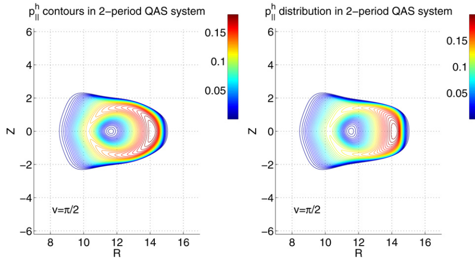
Fig. 14. The hot particle parallel pressure p_{\parallel}^h contours for p_{\perp} > p_{\parallel} HF side deposition ( B_c = 4.9T ; \langle\beta_{\perp}^h\rangle/\langle\beta_{\parallel}^h\rangle \simeq 3.4 ) (left) and p_{\perp} > p_{\parallel} LF side deposition ( B_c = 4.2T ; \langle\beta_{\perp}^h\rangle/\langle\beta_{\parallel}^h\rangle \simeq 3.4 ) (right) at midperiod in a 2-field period quasiaxisymmetric stellarator reactor at \langle\beta\rangle \simeq 4.5\% .
