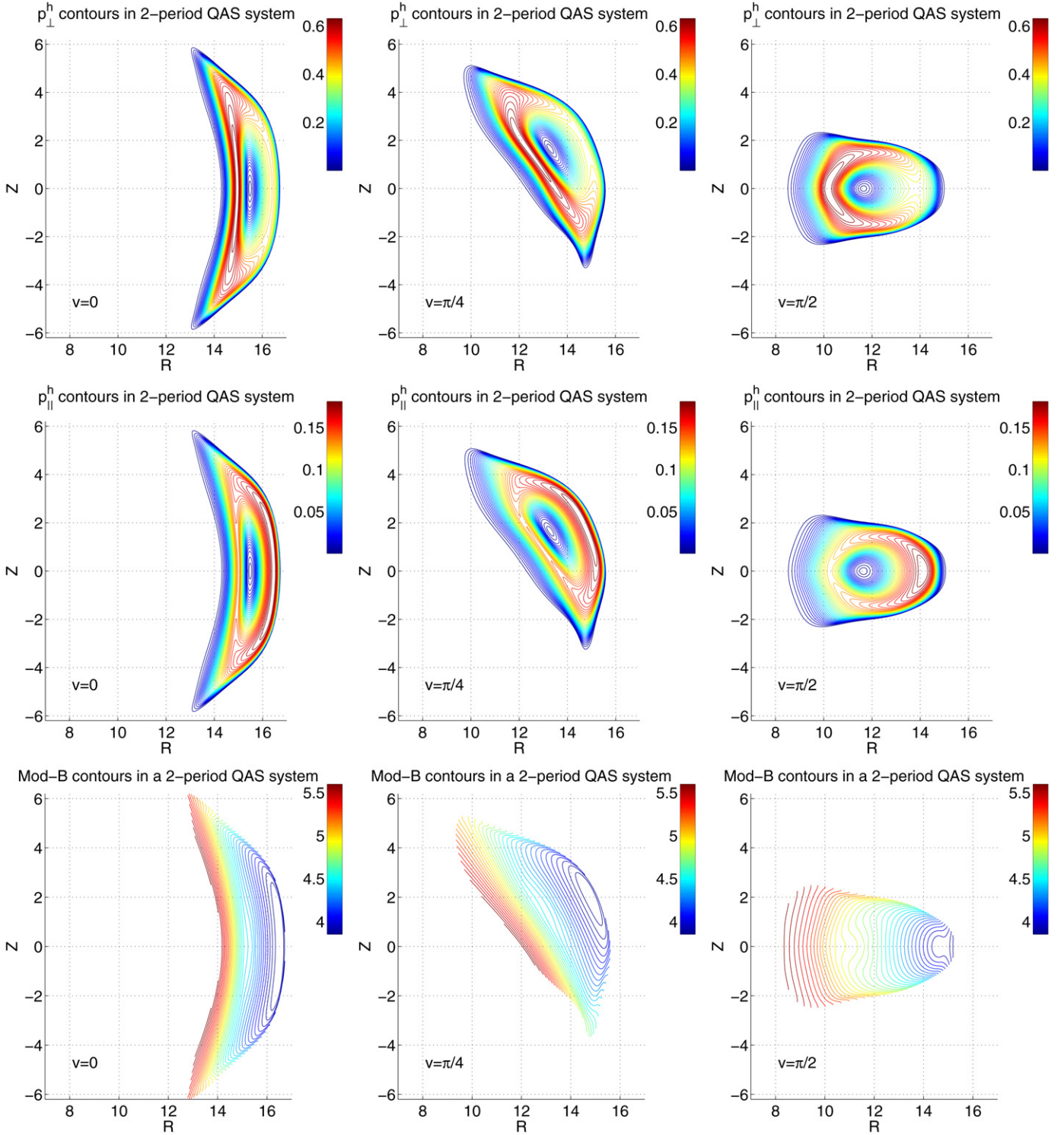
Fig. 12. The contours of constant hot particle perpendicular pressure p_{\perp}^h (top row), hot particle parallel pressure p_{\parallel}^h (middle row) and the mod-B (bottom row) in a 2-field period quasiaxisymmetric stellarator reactor system with high field side energetic particle deposition at \langle \beta \rangle \simeq 4.5\% with large perpendicular anisotropy ( p_{\perp} > p_{\parallel} ) corresponding to \langle \beta_{\perp}^h \rangle / \langle \beta_{\parallel}^h \rangle \simeq 3.4 on three cross sections spanning half of a field period.
