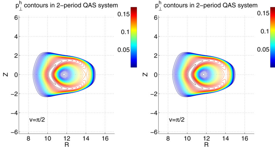
Fig. 15. The hot particle perpendicular pressure p_{\perp}^h contours for p_{\parallel} > p_{\perp} HF side deposition ( B_c = 4.9T ; \langle \beta_{\perp}^h \rangle / \langle \beta_{\parallel}^h \rangle \simeq 1/3.4 ) (left) and p_{\parallel} > p_{\perp} LF side deposition ( B_c = 4.2T ; \langle \beta_{\perp}^h \rangle / \langle \beta_{\parallel}^h \rangle \simeq 1/3.4 ) (right) at midperiod in a 2-field period quasiaxisymmetric stellarator reactor at \langle \beta \rangle \simeq 4.5\% .
