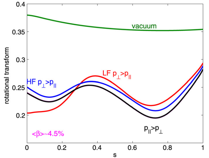
Fig. 10. The vacuum (green curve) and the finite \langle \beta \rangle \simeq 4.5\% rotational transform profiles in a 2-field period quasisymmetric stellarator system with off-axis energetic particle deposition. The finite \beta cases investigated have (a) B_c = 4.9T ; \langle \beta_{\perp}^h \rangle / \langle \beta_{\parallel}^h \rangle \simeq 3.4 (HF side hot particle deposition with p_{\perp} > p_{\parallel} ) (blue curve), (b) B_c = 4.2T ; \langle \beta_{\perp}^h \rangle / \langle \beta_{\parallel}^h \rangle \simeq 3.4 (LF side hot particle deposition with p_{\perp} > p_{\parallel} ) (red curve), (c) B_c = 4.9T ; \langle \beta_{\perp}^h \rangle / \langle \beta_{\parallel}^h \rangle \simeq 1/3.4 (HF side hot particle deposition with p_{\parallel} > p_{\perp} ) (black curve), (d) B_c = 4.2T ; \langle \beta_{\perp}^h \rangle / \langle \beta_{\parallel}^h \rangle \simeq 1/3.4 (LF side hot particle deposition with p_{\parallel} > p_{\perp} ) (magenta curve). The curves with p_{\parallel} > p_{\perp} lay approximately on top of one another. (For interpretation of the references to colour in this figure legend, the reader is referred to the web version of this article.)
