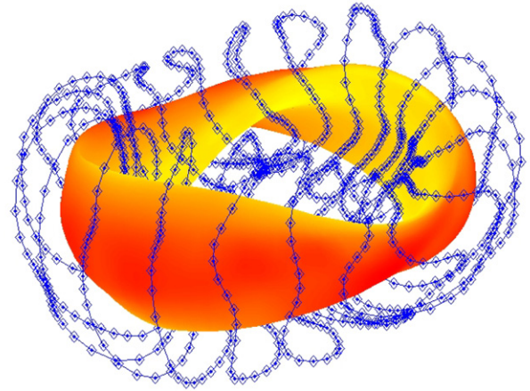
Fig. 3. Filament coil model for a 2-field period quasisymmetric stellarator reactor and the last closed vacuum magnetic flux surface depicting the mod- B distribution. The low magnetic field side is presented in dark shade, the high magnetic field side in lighter shade.
