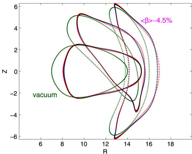
Fig. 5. The shape of the plasma–vacuum interface boundary under vacuum conditions (green curve) and at \langle\beta\rangle \approx 4.5\% for four cases (a) B_c = 4.9T ; \langle\beta_{\perp}^h\rangle/\langle\beta_{\parallel}^h\rangle \approx 3.4 (HF side hot particle deposition with p_{\perp} > p_{\parallel} ) (blue curve), (b) B_c = 4.2T ; \langle\beta_{\perp}^h\rangle/\langle\beta_{\parallel}^h\rangle \approx 3.4 (LF side hot particle deposition with p_{\perp} > p_{\parallel} ) (red curve), (c) B_c = 4.9T ; \langle\beta_{\perp}^h\rangle/\langle\beta_{\parallel}^h\rangle \approx 1/3.4 (HF side hot particle deposition with p_{\parallel} > p_{\perp} ), (d) B_c = 4.2T ; \langle\beta_{\perp}^h\rangle/\langle\beta_{\parallel}^h\rangle \approx 1/3.4 (LF side hot particle deposition with p_{\parallel} > p_{\perp} ) (black curve) on three cross sections spanning half a field period of the quasisymmetric stellarator reactor. The boundaries in cases (c) and (d) are virtually indistinguishable and also very close to case (a). Case (b) bulges out at the elongated up-down symmetric cross section. (For interpretation of the references to colour in this figure legend, the reader is referred to the web version of this article.)
