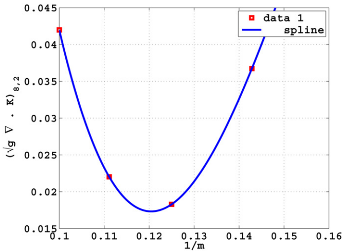
Fig. 9. Convergence of the m_B = 8 , n_B = 2 Fourier component of \sqrt{g}(\nabla \cdot \mathbf{K}) in the Boozer coordinate frame as a function of the inverse of the maximum value of the poloidal mode number m used in the equilibrium computation for the case B_c = 4.9T ; \langle \beta_{\perp}^h \rangle / \langle \beta_{\parallel}^h \rangle \simeq 3.4 (HF side hot particle deposition with p_{\perp} > p_{\parallel} ) in a 2-period quasisymmetric stellarator. The ordinate has not been normalised so its units are A/m .
