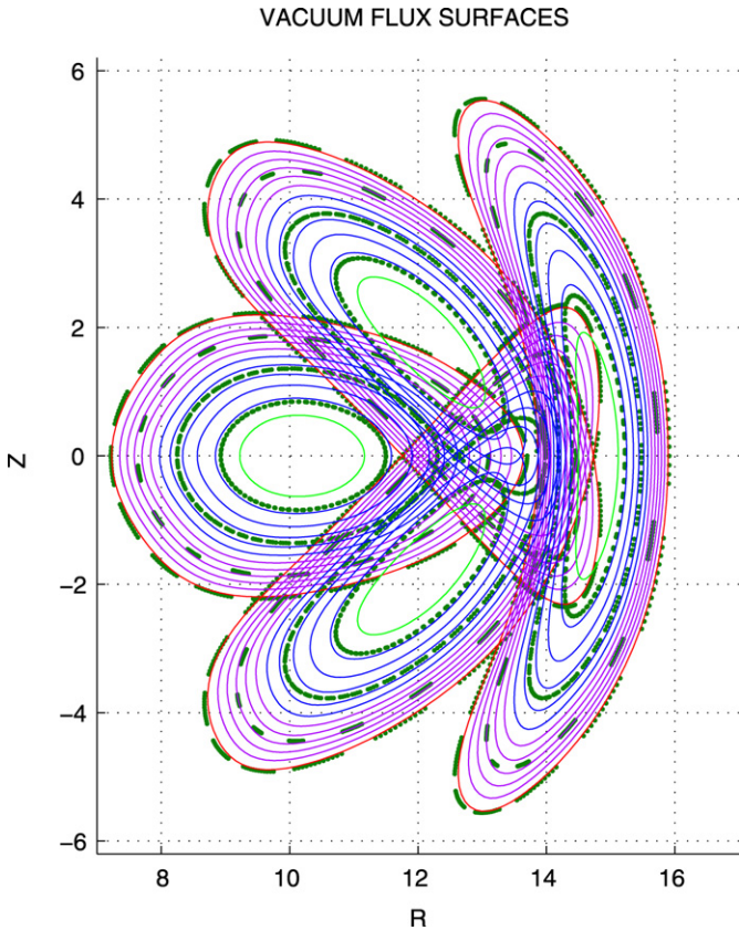
Fig. 4. A Poincaré plot computed with a magnetic field line tracing solver (green dots) and the vacuum magnetic flux surfaces calculated with the ANIMEC code on four cross section spanning three fourths of a field period in the quasisymmetric stellarator. (For interpretation of the references to colour in this figure legend, the reader is referred to the web version of this article.)
