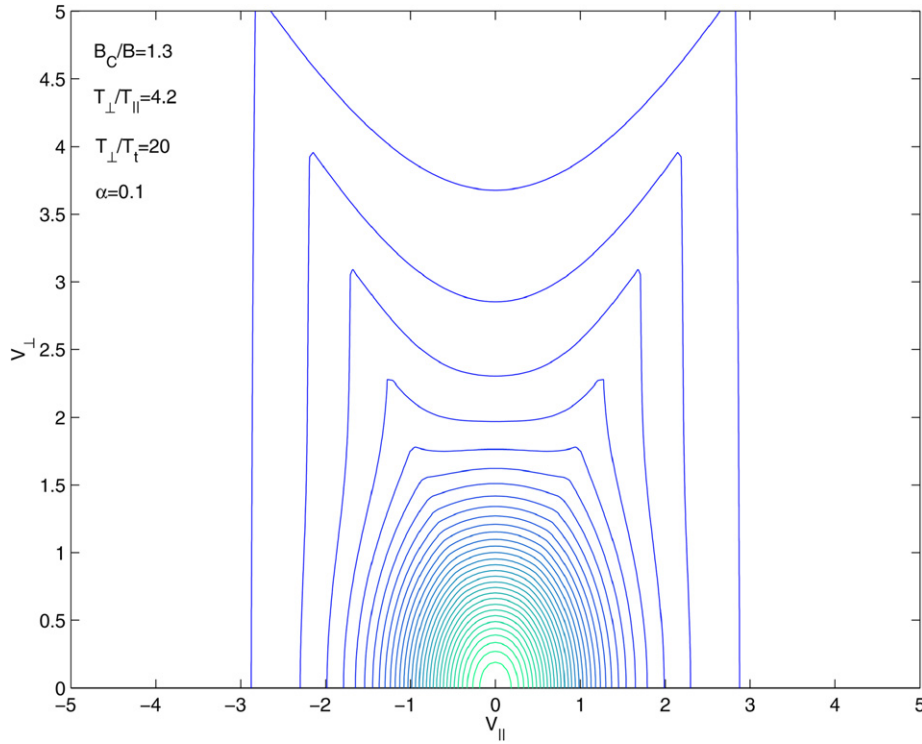
Fig. 1. Contours of constant hot particle distribution in v_{\perp} versus v_{\parallel} space. The distribution function plotted corresponds to \mathcal{N}(m_h/2\pi T_{\perp})^{3/2}[\alpha(T_{\perp}/T_t)^{3/2} \exp(-m_h \mathcal{E}/T_t) + (1-\alpha) \exp(-\mu B_C/T_{\perp} - |\mathcal{E} - \mu B_C|/T_{\parallel})] where the thermal, hot particle perpendicular and hot particle parallel temperatures are T_t , T_{\perp} and T_{\parallel} , respectively. The parameters required are given by \alpha = 0.1 , T_{\perp}/T_t = 20 , T_{\perp}/T_{\parallel} = 4.2 and B_C/B = 1.3 .
