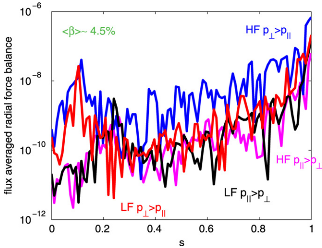
Fig. 8. The absolute values of the flux surface averaged radial force balance profiles for a 2-field period quasisymmetric stellarator reactor system with off-axis hot particle deposition at \langle \beta \rangle \simeq 4.5\% . The cases investigated have (a) B_c = 4.9T ; \langle \beta_{\perp}^h \rangle / \langle \beta_{\parallel}^h \rangle \simeq 3.4 (HF side hot particle deposition with p_{\perp} > p_{\parallel} ) (blue curve), (b) B_c = 4.2T ; \langle \beta_{\perp}^h \rangle / \langle \beta_{\parallel}^h \rangle \simeq 3.4 (LF side hot particle deposition with p_{\perp} > p_{\parallel} ) (red curve), (c) B_c = 4.9T ; \langle \beta_{\perp}^h \rangle / \langle \beta_{\parallel}^h \rangle \simeq 1/3.4 (HF side hot particle deposition with p_{\parallel} > p_{\perp} ) (magenta curve), (d) B_c = 4.2T ; \langle \beta_{\perp}^h \rangle / \langle \beta_{\parallel}^h \rangle \simeq 1/3.4 (LF side hot particle deposition with p_{\parallel} > p_{\perp} ) (black curve). (For interpretation of the references to colour in this figure legend, the reader is referred to the web version of this article.)
