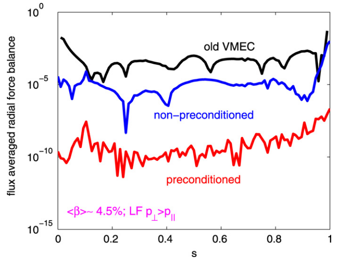
Fig. 7. The absolute values of the flux surface averaged radial force balance profiles for a 2-field period quasisymmetric stellarator reactor system with off-axis hot particle deposition at \langle\beta\rangle \approx 4.5\% corresponding to B_c = 4.2T ; \langle\beta_{\perp}^h\rangle/\langle\beta_{\parallel}^h\rangle \approx 3.4 (LF side hot particle deposition with p_{\perp} > p_{\parallel} ), computed with an old version of VMEC (black curve), with ANIMEC without matrix preconditioning (blue curve) and with the preconditioned ANIMEC code (red curve). (For interpretation of the references to colour in this figure legend, the reader is referred to the web version of this article.)
