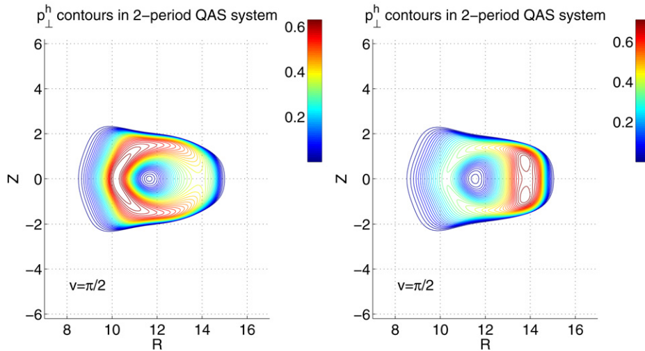
Fig. 13. The hot particle perpendicular pressure p_{\perp}^h contours for p_{\perp} > p_{\parallel} HF side deposition ( B_c = 4.9T ; \langle\beta_{\perp}^h\rangle/\langle\beta_{\parallel}^h\rangle \simeq 3.4 ) (left) and p_{\perp} > p_{\parallel} LF side deposition ( B_c = 4.2T ; \langle\beta_{\perp}^h\rangle/\langle\beta_{\parallel}^h\rangle \simeq 3.4 ) (right) at midperiod in a 2-field period quasiaxisymmetric stellarator reactor at \langle\beta\rangle \simeq 4.5\% .
