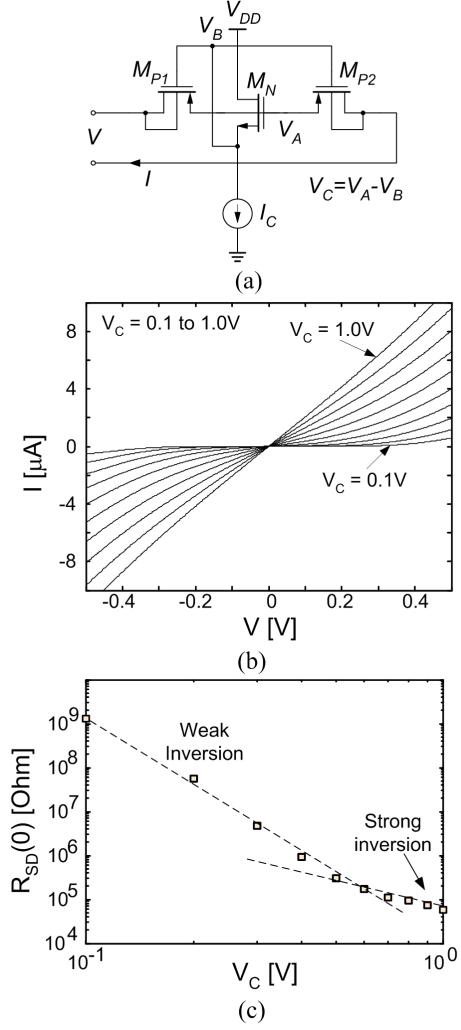
Fig. 3. Proposed floating resistance: (a) circuit schematic, (b) measured I-V characteristics of the proposed configuration for different V_C values, (c) measured resistance of the proposed floating resistor with respect to the gate-source voltage of MN ( V_C = V_{GS,MN} = V_{SG,MP1,2} ).
