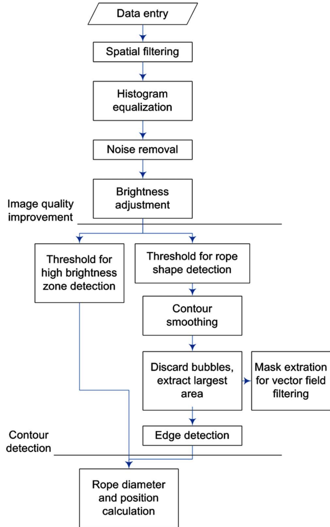
Fig. 5 Image-processing flowchart
