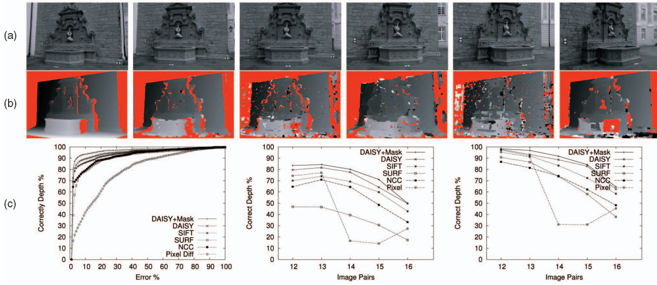
Fig. 11. Comparing different descriptors: Fountain Sequence [28]. (a) In our tests, we match the leftmost image against each one of the other five. (b) The laser-scan depth map we use as a reference and five depth maps computed from the first and third images. From left to right, we used DAISY, SIFT, SURF, NCC, and Pixel Difference. (c) The leftmost plot shows the corresponding distributions of deviations from the laser-scan data, expressed as a fraction of the scene’s depth range. The other plots summarize these distributions for the five stereo pairs of increasing baseline with discrete error thresholds set to be 1 and 5 percent of the scene’s depth range, respectively. Each data point represents a pair where the baseline increases gradually from left to right and individual curves correspond to DAISY with masks, DAISY without masks, SIFT, SURF, NCC, and Pixel Difference. In all cases, DAISY does better than the others and using masks further improves the results.
