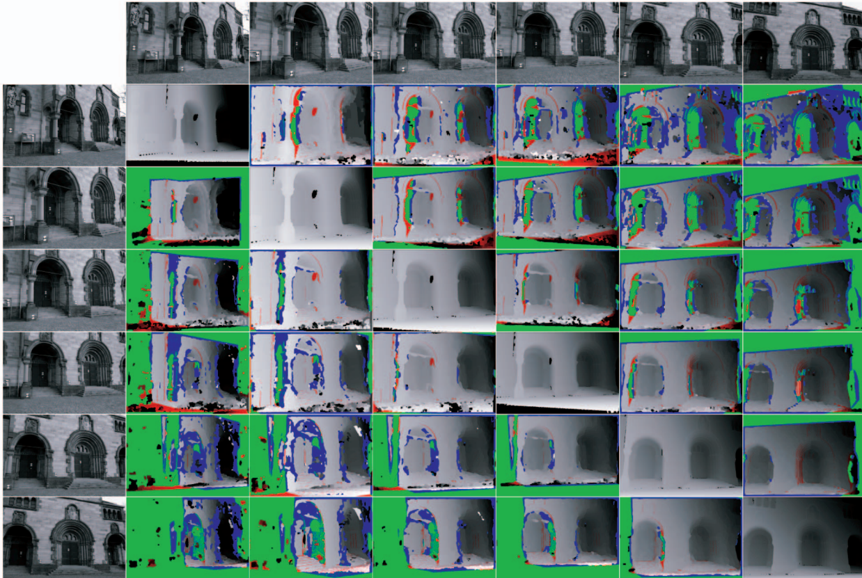
Fig. 14. HerzJesu Grid: By using two images, one from the leftmost column and one from the upper row, we compute depth and occlusion maps from the viewpoint of the row image. In the diagonal, we display the ground truth depth maps. We marked the correctly detected occlusions with green, incorrectly detected ones with blue, and the missed ones with red. From this figure, it is apparent that DAISY can handle quite large baselines without losing too much from its accuracy, as can be seen from Table 3.
