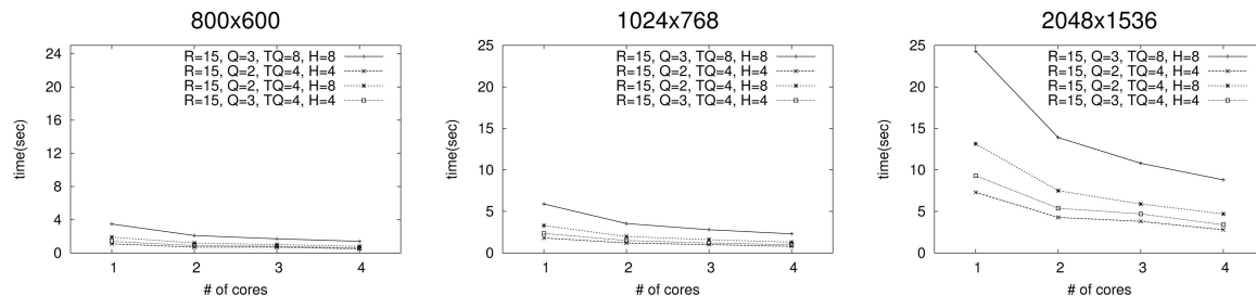
Fig. 7. DAISY Computation Times: Computation times of the DAISY descriptor for all the pixels of an image with various settings on three different sized images. We present the change of the computation time with respect to the number of cores used in parallel.
