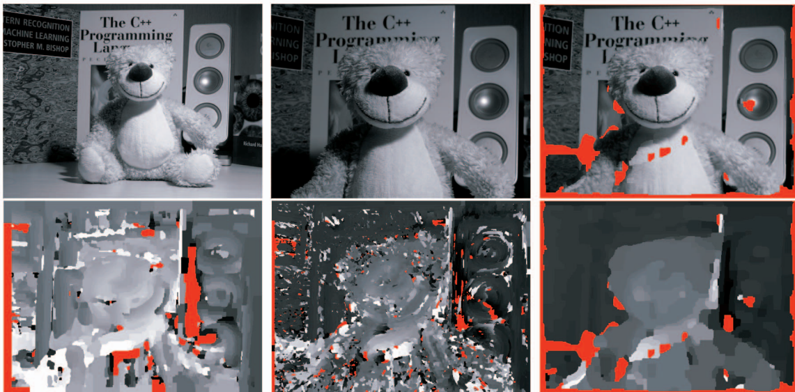
Fig. 2. Scale Change: We used the first two images of the upper row for computing the depth map from the second image's point of view. The depth maps are computed using NCC, SIFT, and DAISY, and they are displayed in the lower row in that order. The last image in the first row shows the resynthesized image using the DAISY's depth estimate. Although scale change is not explicitly addressed in any way and we used the same parameters for the descriptors of two images, we obtain a very acceptable depth map.
