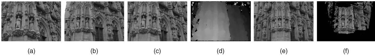
Fig. 20. Results on low-resolution versions of the Rathaus images [27]: (a)-(c) Three input images of size 768 \times 512 instead of the 3,072 \times 2,048 versions that were used in [26]. (d) Depth map computed using all three images. (e) A fourth image not used for reconstruction. (f) Image synthesized using the depth map and the image texture in (a) with respect to the view point of (e). Note how similar it is to (e). The holes are caused by the fact that a lot of the texture in (e) is not visible in (a).
