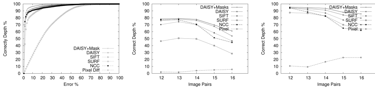
Fig. 13. Quantitative comparison results for Fig. 12: The leftmost plot shows the corresponding distributions of deviations from the laser-scan data, expressed as a fraction of the scene's depth range. The other plots summarize these distributions for the five stereo pairs of increasing baseline with discrete error thresholds set to be 1 and 5 percent of the scene's depth range, respectively. Each data point represents a pair where the baseline increases gradually from left to right and individual curves correspond to DAISY with masks, DAISY without masks, SIFT, SURF, NCC, and Pixel Difference. In all cases, DAISY does better than the others and using masks further improves the result.
