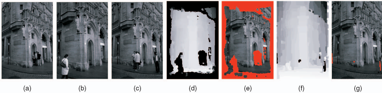
Fig. 21. Low-resolution versions of the Brussels images [26]: (a)-(c) Three 768 \times 510 versions of the original 2,048 \times 1,360 images. (d) and (e) The depth map computed using images (a) and (b) seen in the perspective of image (c) and the corresponding resynthesized image. Note that the locations where there are people in one image and not in the other are correctly marked as occlusions. (f) and (g) The depth map and synthetic image generated using all three images. Note that the previously occluded areas are now filled and that the people have been erased from the synthetic image.
