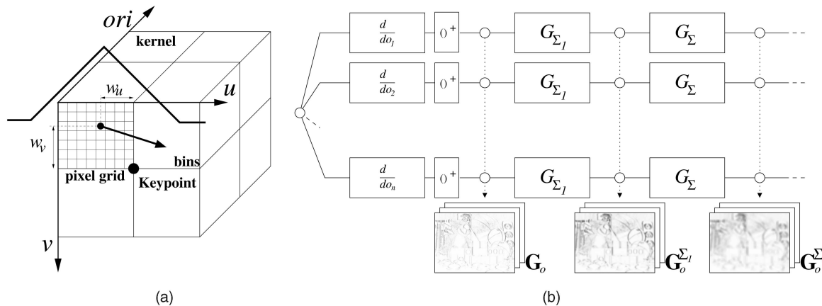
Fig. 5. Relationship between SIFT and DAISY: (a) SIFT is a 3D histogram computed over a local area where each pixel location contributes to bins depending on its location and the orientation of its image gradient, the importance of the contribution being proportional to the norm of the gradient. Each gradient vector is spread over 2 \times 2 \times 2 bins to avoid boundary effects, and its contribution to each bin is weighted by the distances between the pixel location and the bin boundaries. (b) DAISY computes similar values but in a dense way. Each gradient vector also contributes to several of the elements of the description vector, but the sum of the weighted contributions is computed by convolution for better computation times. We first compute orientation maps from the original images, which are then convolved to obtain the convolved orientation maps G_o^{\Sigma_1} . The values of the G_o^{\Sigma_1} correspond to the values in the SIFT bins, and will be used to build DAISY. By chaining the convolutions, the G_o^{\Sigma_2} can be obtained very efficiently.
