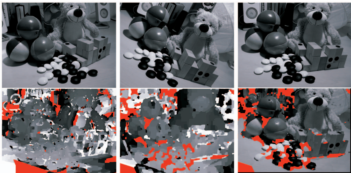
Fig. 4. Rotation around a point: We used the first two images of the upper row for computing the depth map from the third image's point of view. The depth maps are computed using NCC and DAISY, and they are displayed in the lower row in that order. The last image in the second row shows the resynthesized image using the DAISY's depth estimate.
