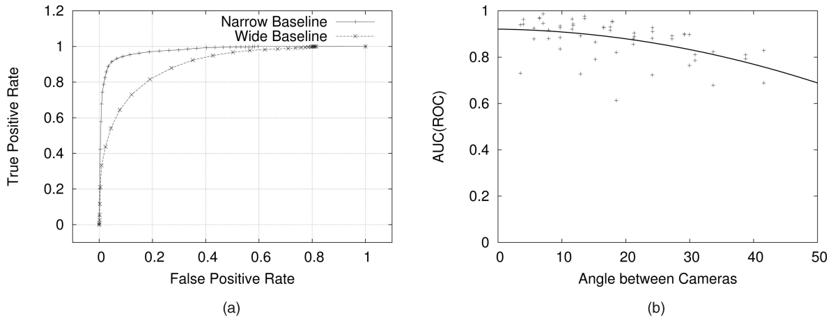
Fig. 16. ROC for occlusion threshold: We plot ROC curves for the selection of the occlusion threshold for all of the image pairs of Fig. 14. (a) The ROC curves of the narrow-baseline image pair \{4, 5\} and the wide-baseline image pair \{1, 5\} . (b) The area under the curve (AUC) of the ROC graphs of the image pairs with respect to the angle between the principal axes of the cameras. The result of each such pair is represented with a data point and the curve shows the fitted line to these.
