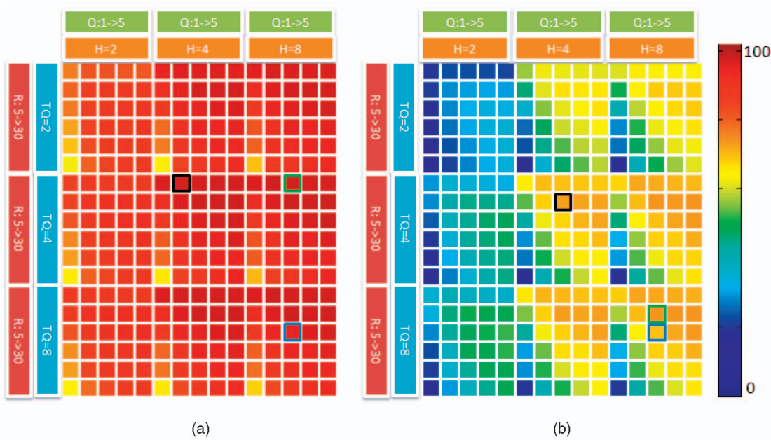
Fig. 10. Parameter sweep test for narrow- and wide-baseline cases: As described by Table 1, there are four parameters that specify the shape and size of DAISY: radius ( R ), radius quantization ( Q ), angular quantization ( T ), and number of bins of the histogram ( H ). The above figures depict the results of a 4D sweep of these parameters and the color of each square represents the percentage of depths that are correctly estimated. The value associated to a color is given by the color scale on the right. To assess the correctness of an estimated depth, we used laser-scanned depth maps and assumed an estimate as correct if the estimate error is within 1 percent of the scene's depth range. (a) The averaged result for five narrow-baseline image pairs of the Fountain sequence of Fig. 11. The green rectangle denotes the best parameter set for this configuration which is R = 5, Q = 3, T = 4, H = 8 , resulting in a descriptor of size 104 with a 81.2 percent correct depth estimates. However, upon closer inspection, we see that many other configurations produce similar results (80+ percent). Among these, the configuration R = 5, Q = 2, T = 4, H = 4 produces the shortest descriptor length of 36. It is denoted by the black rectangle. (b) The averaged result for three wide-baseline image pairs of the Fountain sequence. The best result, again denoted by a green rectangle, 73 percent correct depth estimate is achieved with R = 10, Q = 3, T = 8, H = 8 which yields a 200 length descriptor. However, as in the narrow-baseline case, there are many other configurations that produce a very similar performance (71+ percent) with shorter descriptor sizes. The shortest one (black rectangle) is R = 10, Q = 3, T = 4, H = 4 with 52 length. Having multiple configurations that result in similarly high performance shows that we don't really need to change our descriptor parameters depending on the baseline to improve performance, but we can change to meet speed or memory requirements. The configuration we used ( R = 15, Q = 3, T = 8, H = 8 ) in all of the other experiments presented in this paper is outlined in blue.
