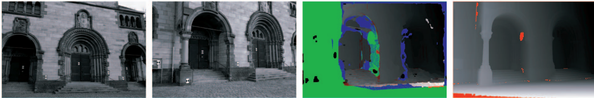
Fig. 15. HerzJesu Close-up: Depth map is computed from the second image's point of view using DAISY. Correctly detected occlusions are shown in green, incorrectly detected ones with blue, and the missed ones with red. The last image is the laser-scanned ground truth depth map.
