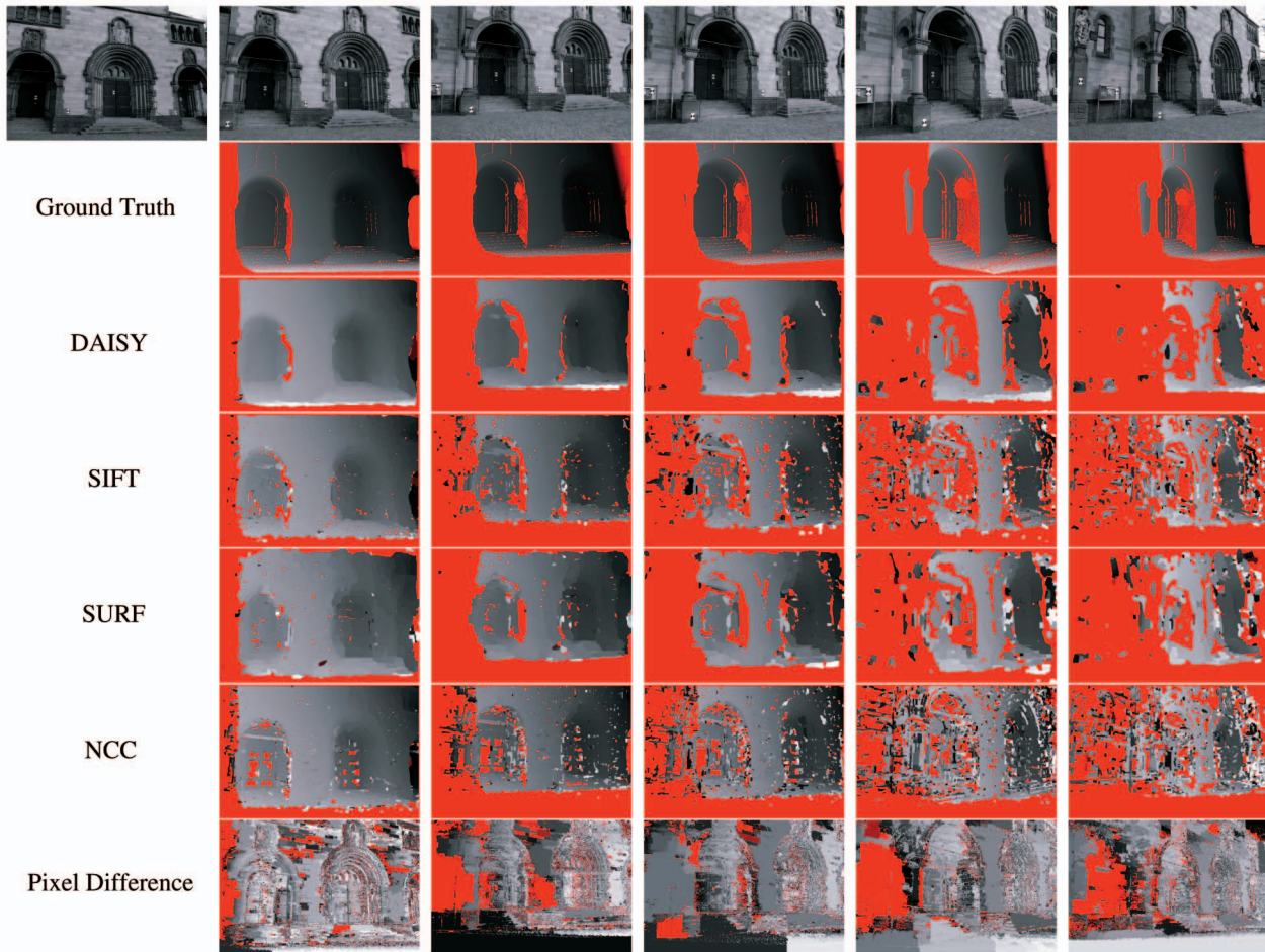
Fig. 12. Comparing different descriptors: HerzJesu Sequence [28]. As in the Fountain sequence of Fig. 11, we use different descriptors to match the leftmost images with each one of the other images. We compute the depth map in the reference frame of these. Second row: Ground truth depth maps with overlaid occlusion masks. Remaining rows: Depth maps computed using DAISY, SIFT, SURF, NCC, and Pixel differencing, in that order.
