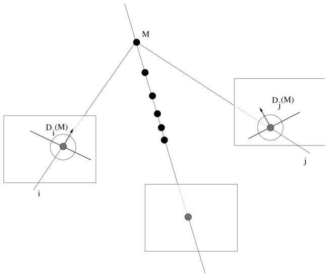
Fig. 8. Problem Definition: The inverse depth is discretized uniformly and the matching score is computed using neighborhoods centered around the projected locations. These neighborhoods are rotated to conform to the orientation of the epipolar lines.
