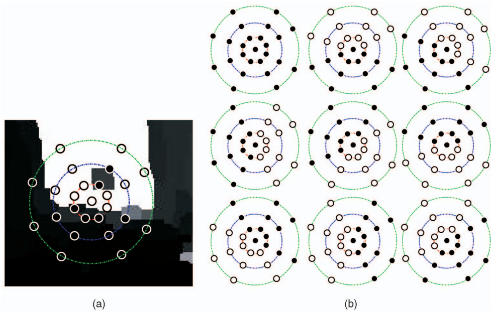
Fig. 9. Binary masks for occlusion handling: We use binary masks over the descriptors to estimate location similarities even near occlusion boundaries. In this figure, a black disk with a white circumference corresponds to “on” and a white disk to “off.” In (a), we use the occlusion map to define the masks and, in (b), predefined masks make it easy to enforce spatial coherence and to speed up the convergence of EM estimation.
