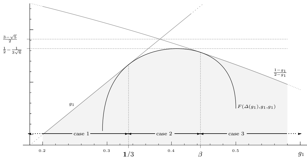
Fig. 1. How the approximation factor depends on g_1 .
