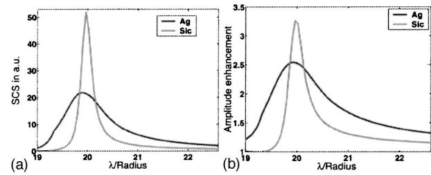
Fig. 17. Comparison of the SCS and the near-field amplitude enhancement of a circular cylinder made of Ag and SiC.
