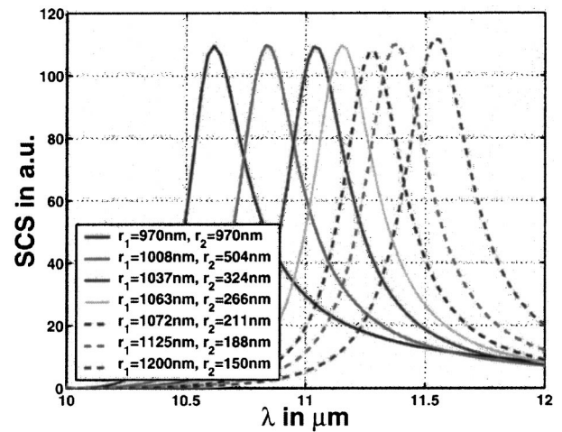
Fig. 9. SCS of an elliptical cylinder as a function of the radii.
