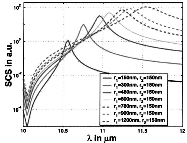
Fig. 7. SCS of an elliptical cylinder as a function of the axis ratio (from 1 to 8).
