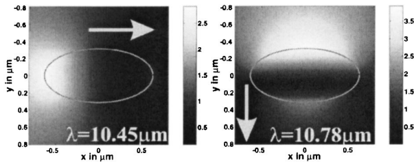
Fig. 4. Near-field amplitude around an elliptical cylinder ( r_1 = 630 \text{ nm} , r_2 = 315 \text{ nm} ) at the resonance wavelengths.
