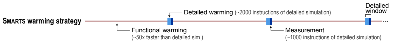
Figure 1. SMARTS two-tier warming strategy. Functional warming dominates runtime because it must cover billions of instructions.
