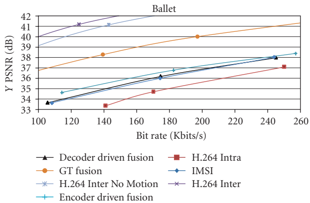
FIGURE 36: RD performance for Ballet .
