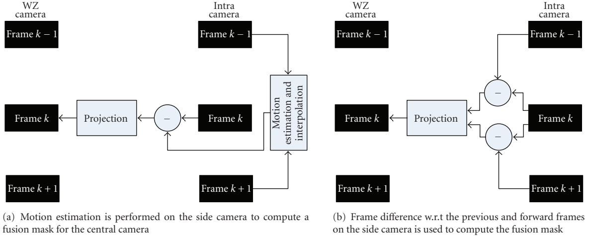
FIGURE 6: Fusion techniques proposed by Artigas et al. [13].
