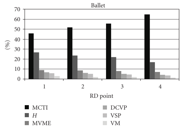
FIGURE 28: The percentage of contribution of the different side information in the GT fusion for Ballet .
