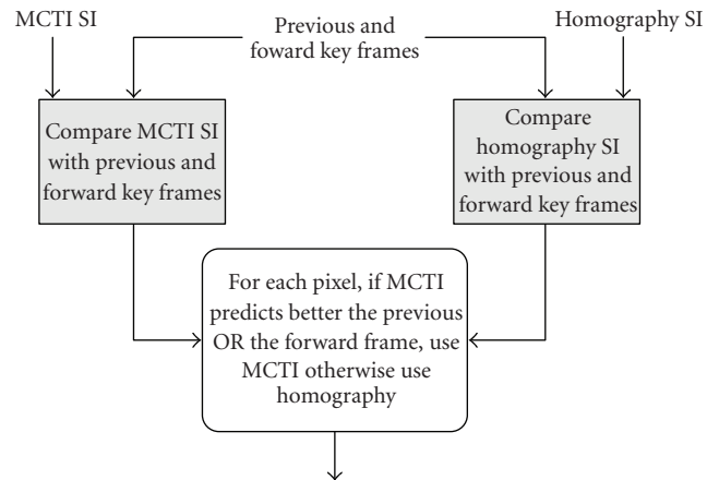
FIGURE 5: Decoder-driven fusion [12].
