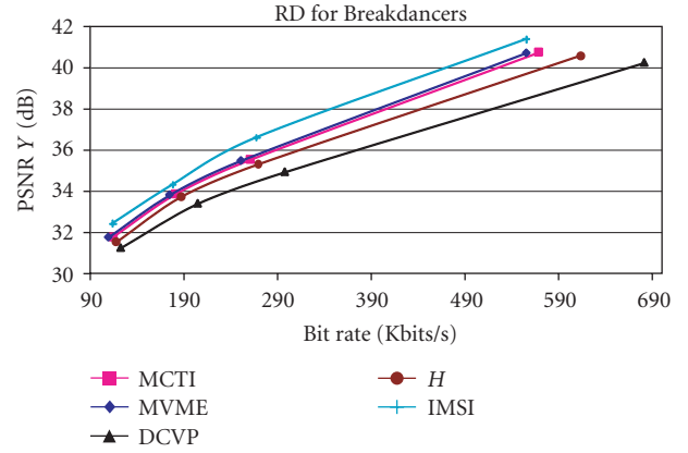
FIGURE 30: RD performance for Breakdancers .
