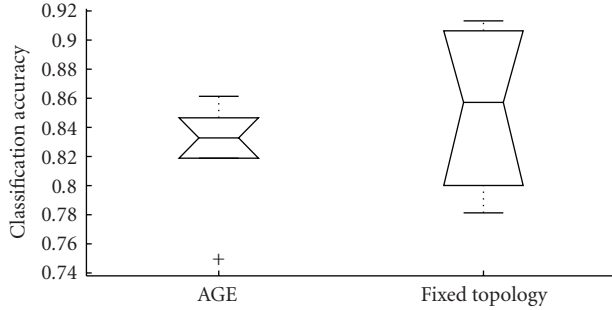
FIGURE 8: The average classification accuracy of the evolved networks (AGE) and the fixed topology networks trained with back propagation ( fixed topology ). The midline in each box is the median, the borders of the box represent the upper and the lower quartiles. The whiskers outside the box represent the minimum and maximum values obtained, except when there are outliers which are shown as small crosses. We define outliers as data points which differ more than 1.5 times the interquartile range from the border of the box. The notches permit the assessment of the significance of the differences of the medians. When the notches of two boxes overlap, the corresponding medians are not significantly different at (approximately) the 95% confidence level [34].
