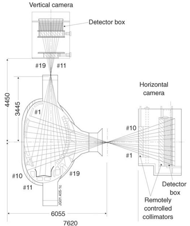
Fig. 29. Schematic view of the JET neutron emission profile monitor used for the spatial gamma ray emission measurements. 74
