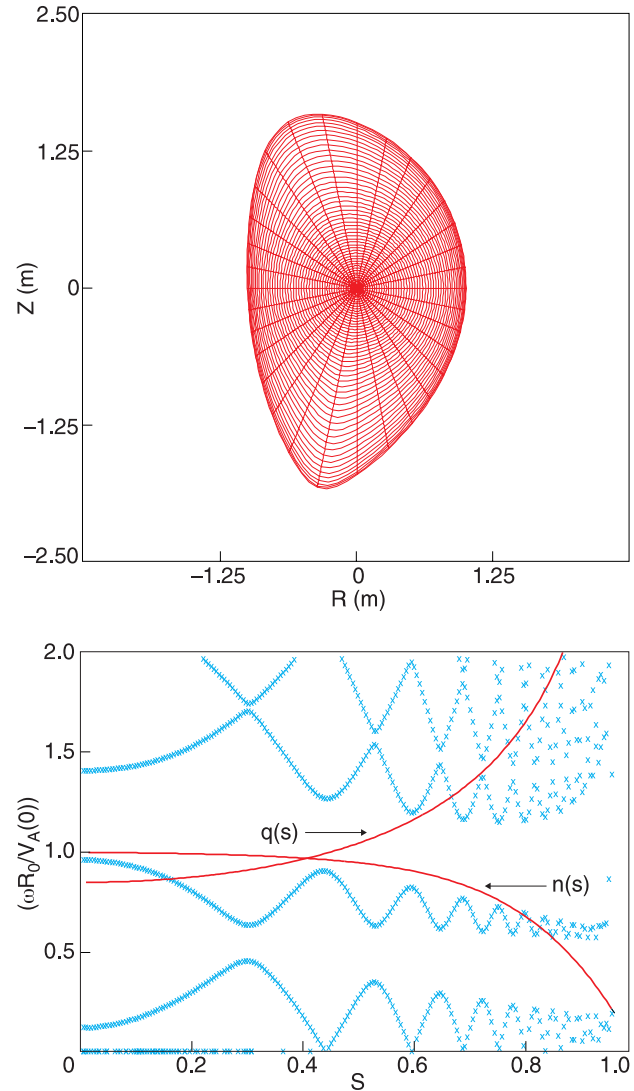
Fig. 10. The reconstructed equilibrium 9 for D-T discharge 42677 at t = 13.3 s, together with the Alfvén continuum structure. q(s) and n(s) are the safety factor and electron density radial profiles; q(0) = 0.85 .
