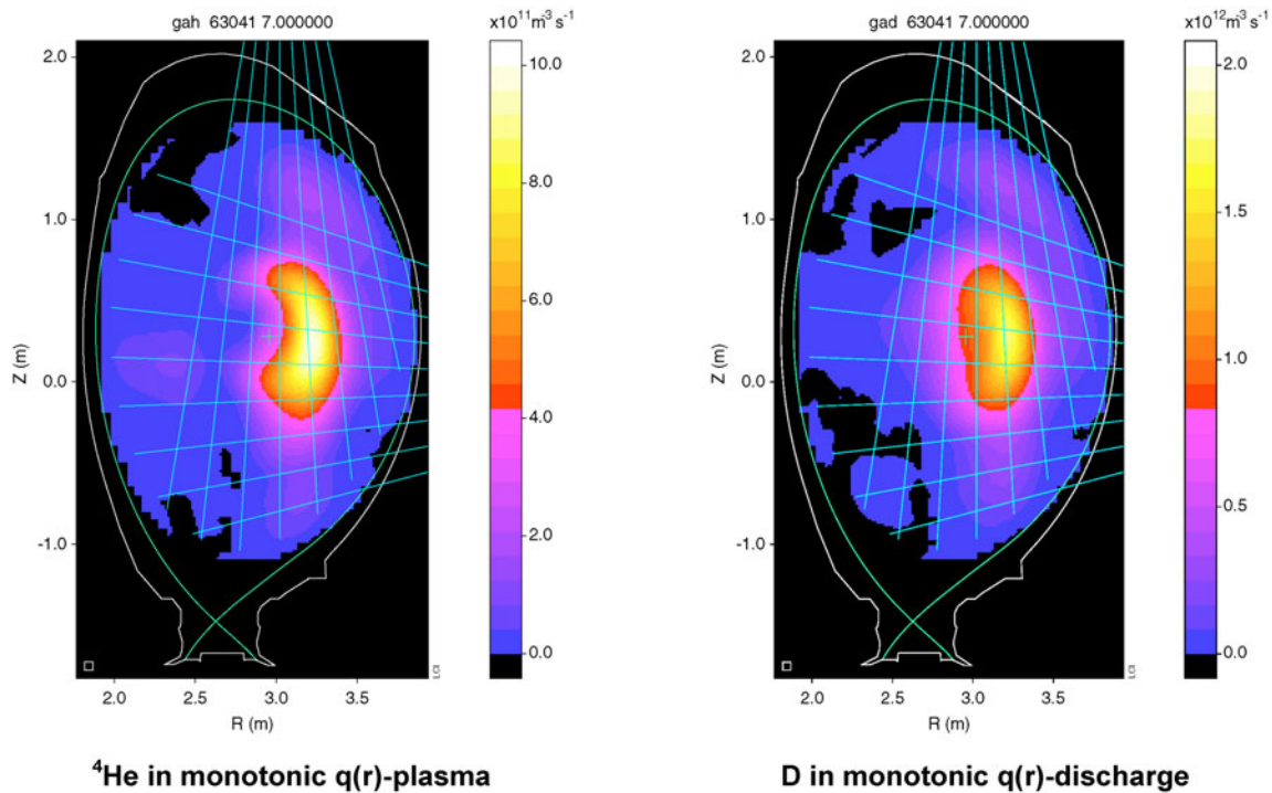
Fig. 30. Tomographic reconstructions of 4.44-MeV gamma-ray emission from nuclear reaction {}^9\text{Be}({}^4\text{He}, n\gamma){}^{12}\text{C} (left) and 3.09-MeV gamma-ray emission from the reaction {}^{12}\text{C}(\text{D}, p\gamma){}^{13}\text{C} (right) deduced from simultaneously measured profiles. 77
