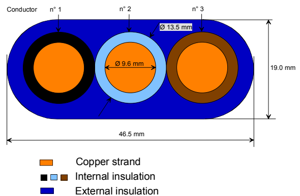
Figure 2. Cable n° 1. Pirelli SGFLT-0 3 x 50mm 2 , 20.5 m
